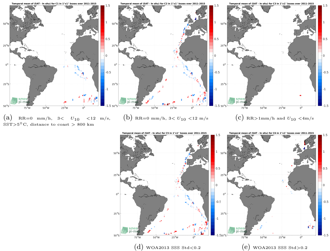
Figure 12: Temporal mean gridded over spatial boxes of size 1^\circ \times 1^\circ of \Delta SSS (Aquarius SSS L2 CAP v5 (JPL) - TSG (Polarstern)) for 5 different subdatasets corresponding to:RR=0 mm/h, 3 < U_{10} < 12 m/s, SST >5^\circ\text{C} , distance to coast > 800 km (a), RR=0 mm/h, 3 < U_{10} < 12 m/s (b), RR >1 mm/h and U_{10} < 4 m/s (c), WOA2013 SSS Std <0.2 (d), WOA2013 SSS Std >0.2 (e).
