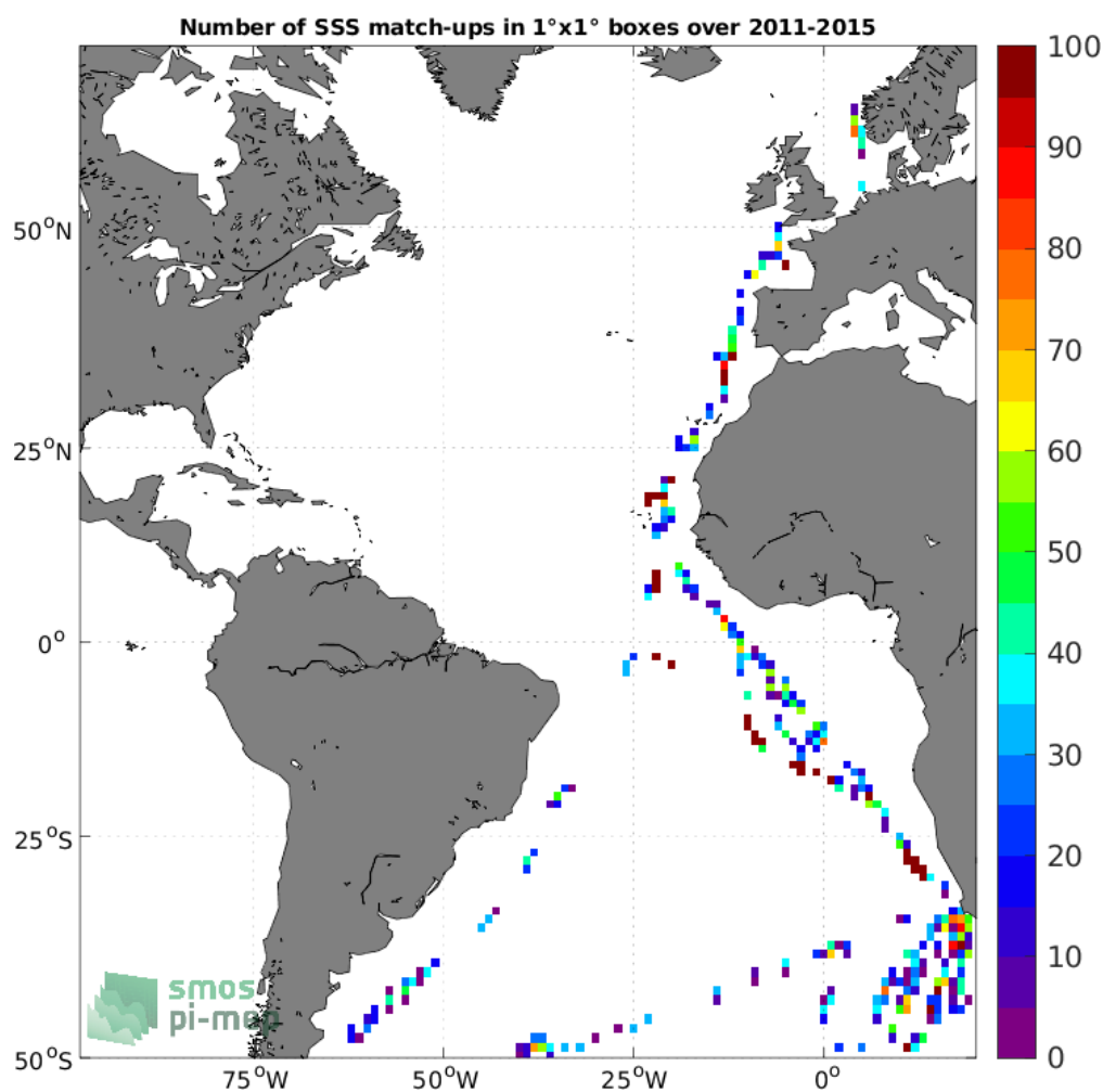
Figure 4: Number of SSS match-ups between TSG (Polarstern) SSS and the Aquarius SSS L2 CAP v5 (JPL) SSS product for the Atlantic Ocean Pi-MEP region over 1°x1° boxes and for the full satellite product period.
