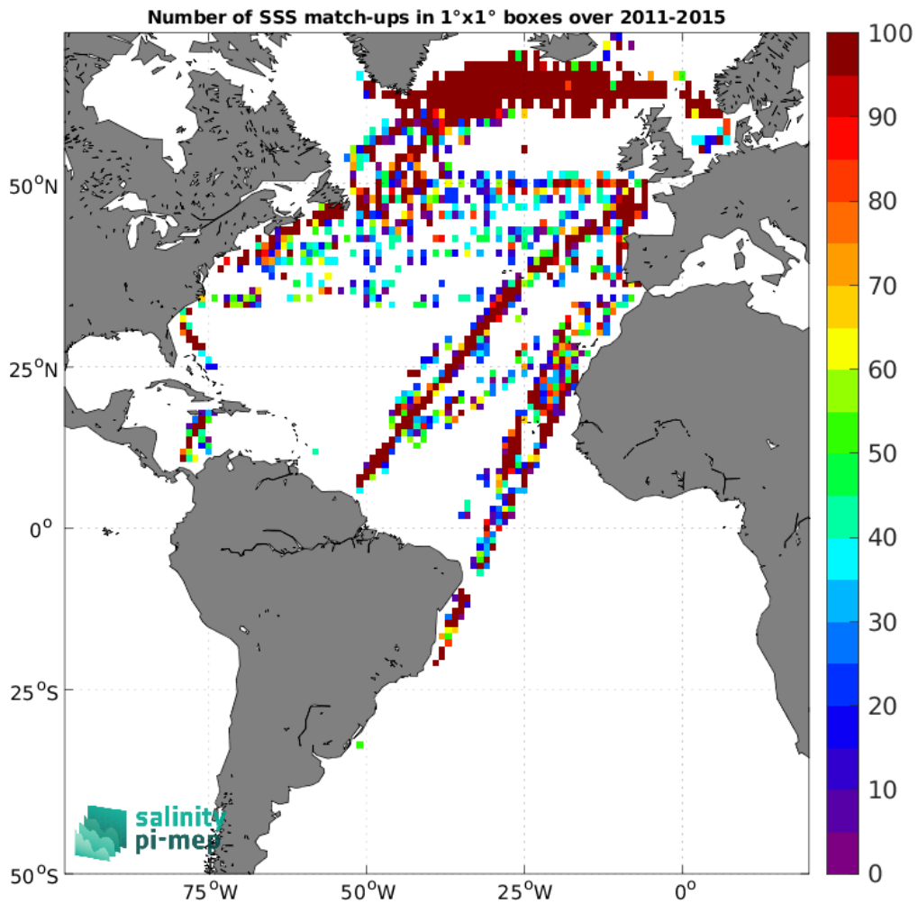
Figure 4: Number of SSS match-ups between TSG (LEGOS-DM) SSS and the Aquarius SSS L2 CAP v5 (JPL) SSS product for the Atlantic Ocean Pi-MEP region over 1^\circ \times 1^\circ boxes and for the full satellite product period.
