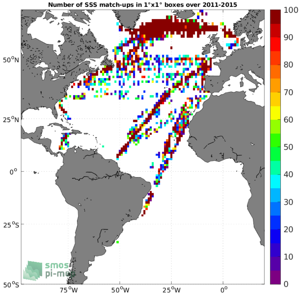
Figure 4: Number of SSS match-ups between TSG (LEGOS-DM) SSS and the Aquarius SSS L2 CAP v5 (JPL) SSS product for the Atlantic Ocean Pi-MEP region over 1°×1° boxes and for the full satellite product period.
