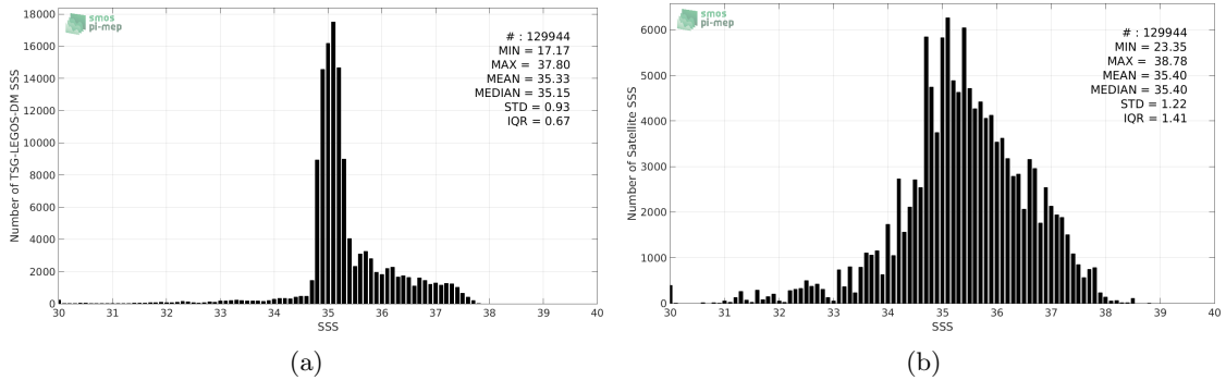
Figure 2: Histograms of SSS from TSG-LEGOS-DM (a) and Aquarius-L2-JPL-V5 (b) considering all match-up pairs per bins of 0.1 over the Atlantic Ocean Pi-MEP region and for the full satellite product period.
