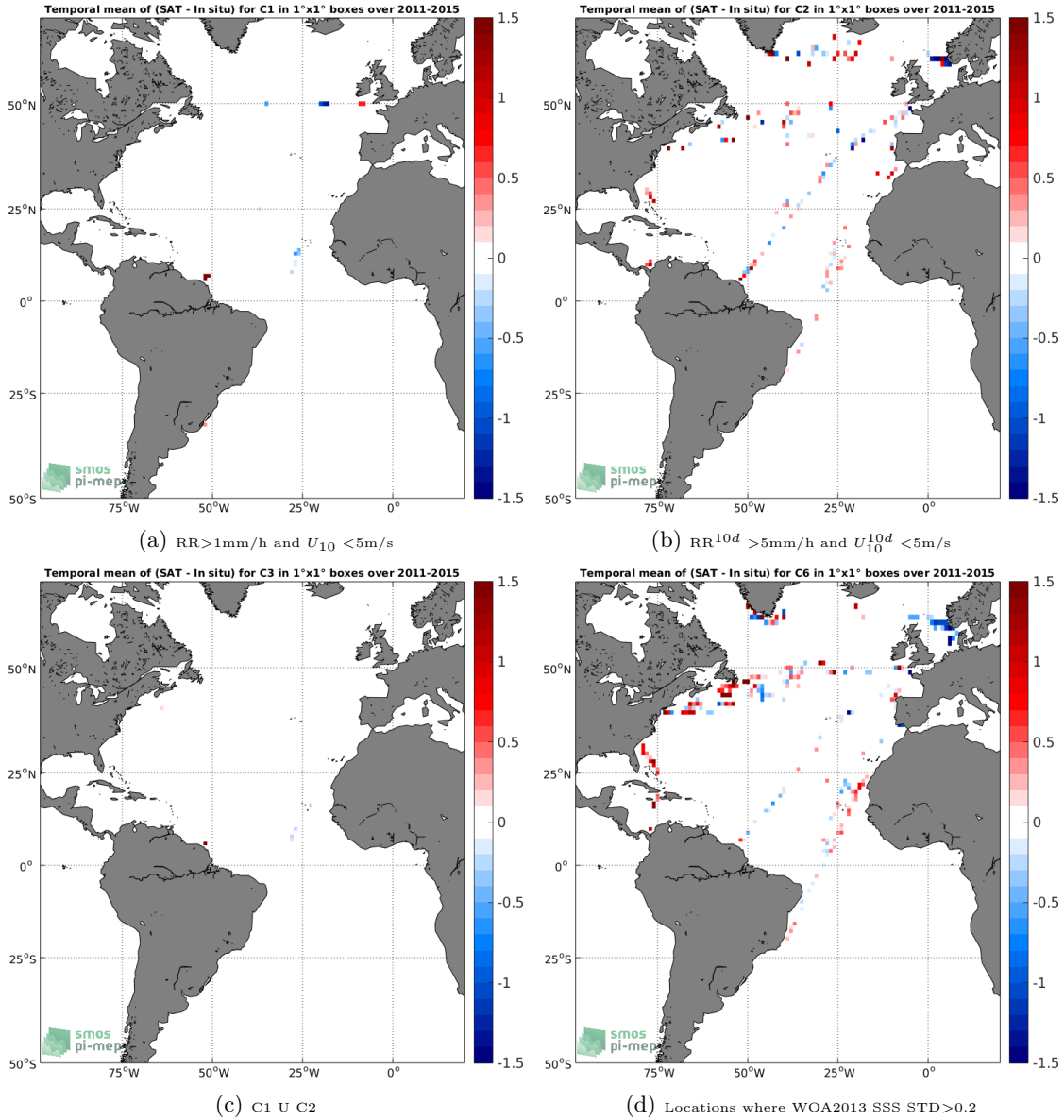
Figure 12: Temporal mean gridded over spatial boxes of size 1^\circ \times 1^\circ of \Delta SSS (Aquarius-L2-JPL-V5 - TSG-LEGOS-DM) for 4 different subdatasets corresponding to: RR > 1mm/h and U_{10} < 5\text{m/s} (a), RR^{10d} > 5\text{mm/h} and U_{10}^{10d} < 5\text{m/s} (b), C1 U C2 (c), Locations where WOA2013 SSS STD > 0.2 (d).
