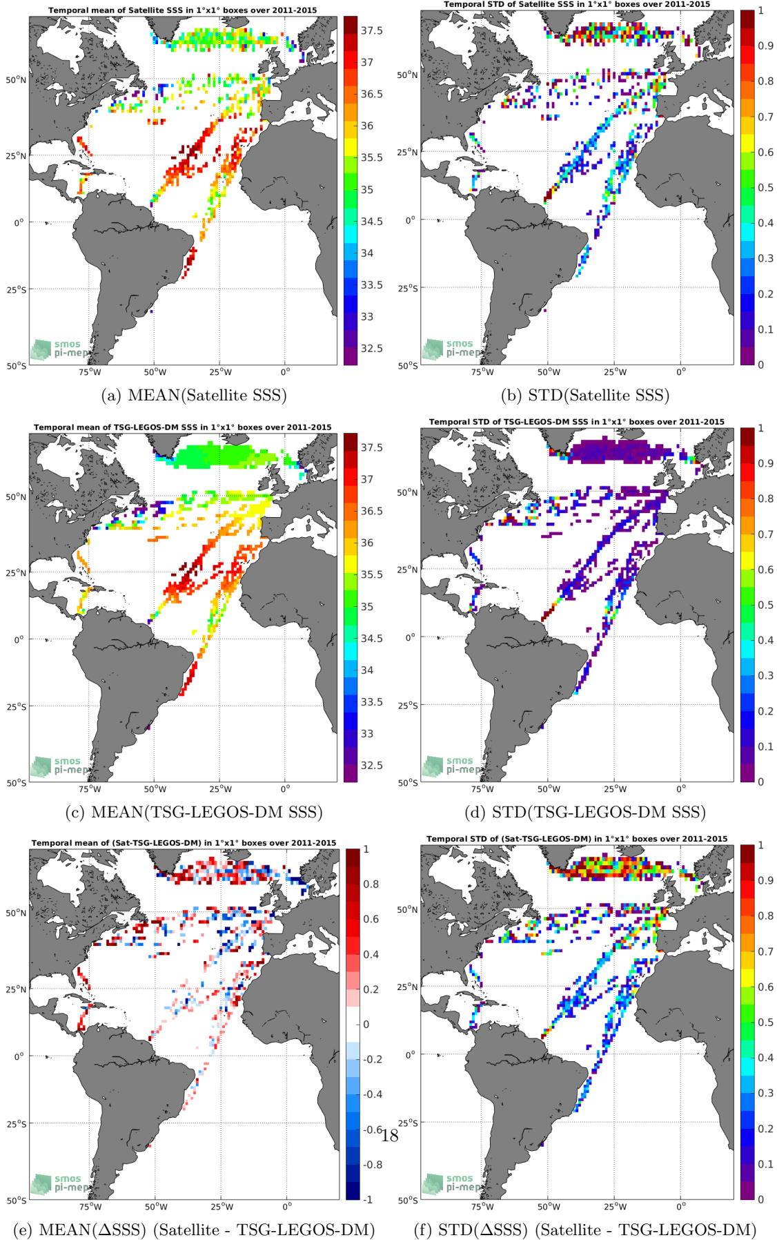
(e) MEAN( \Delta SSS) (Satellite - TSG-LEGOS-DM) (f) STD( \Delta SSS) (Satellite - TSG-LEGOS-DM) Figure 6: Temporal mean (left) and STD (right) of SSS from Aquarius-L2-JPL-V5 (top), TSG-LEGOS-DM (middle), and of \Delta SSS (Satellite - TSG-LEGOS-DM). Only match-up pairs are used to generate these maps.
