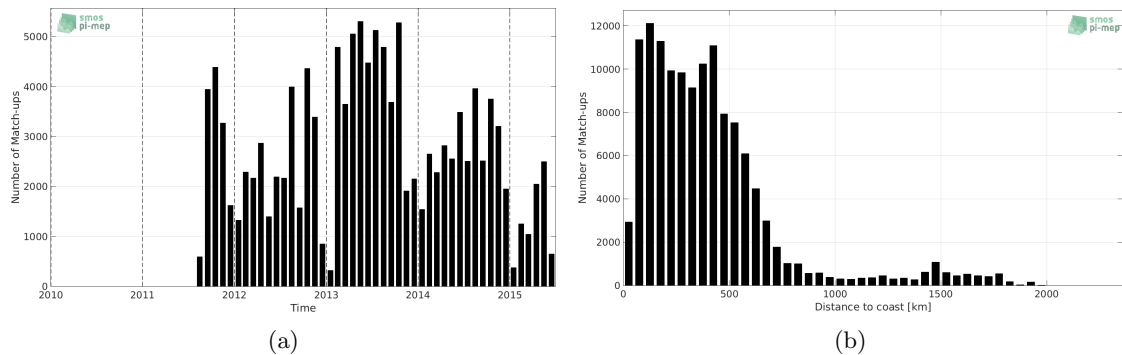
Figure 1: Number of match-ups between TSG-LEGOS-DM and Aquarius-L2-JPL-V5 SSS as a function of time (a) and as function of the distance to coast (b) over the Atlantic Ocean Pi-MEP region and for the full satellite product period.
