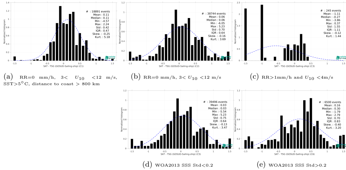
Figure 15: Normalized histogram of \Delta\text{SSS} (Aquarius SSS L2 CAP v5 (JPL) - TSG (GOSUD-Sailing-ship)) for 5 different subdatasets corresponding to: RR=0 mm/h, 3 < U_{10} < 12 m/s, SST > 5°C, distance to coast > 800 km (a), RR=0 mm/h, 3 < U_{10} < 12 m/s (b), RR > 1mm/h and U_{10} < 4 m/s (c), WOA2013 SSS Std < 0.2 (d), WOA2013 SSS Std > 0.2 (e).
