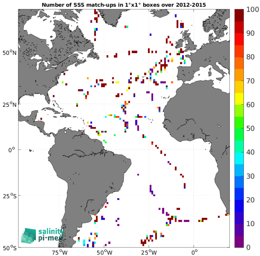
Figure 5: Number of SSS match-ups between TSG (GOSUD-Sailing-ship) SSS and the Aquarius SSS L2 CAP v5 (JPL) SSS product for the Atlantic Ocean Pi-MEP region over 1°×1° boxes and for the full satellite product period.
