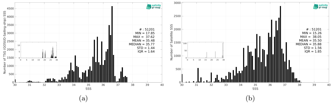
Figure 3: Histograms of SSS from TSG (GOSUD-Sailing-ship) (a) and Aquarius SSS L2 CAP v5 (JPL) (b) considering all match-up pairs per bins of 0.1 over the Atlantic Ocean Pi-MEP region and for the full satellite product period.
