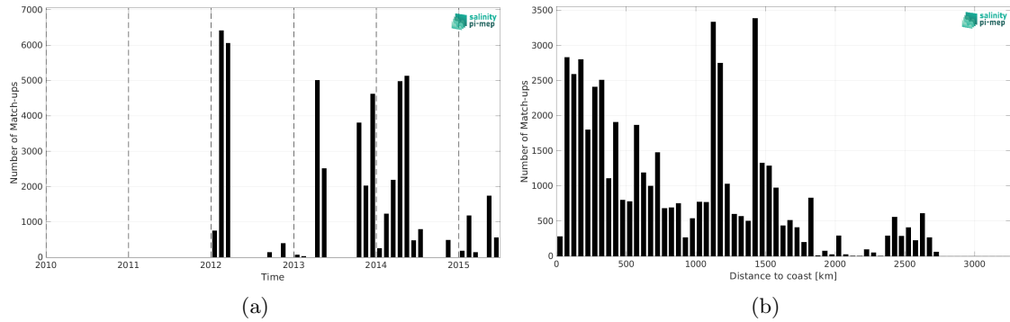
Figure 2: Number of match-ups between TSG (GOSUD-Sailing-ship) and Aquarius SSS L2 CAP v5 (JPL) SSS as a function of time (a) and as function of the distance to coast (b) over the Atlantic Ocean Pi-MEP region and for the full satellite product period.
