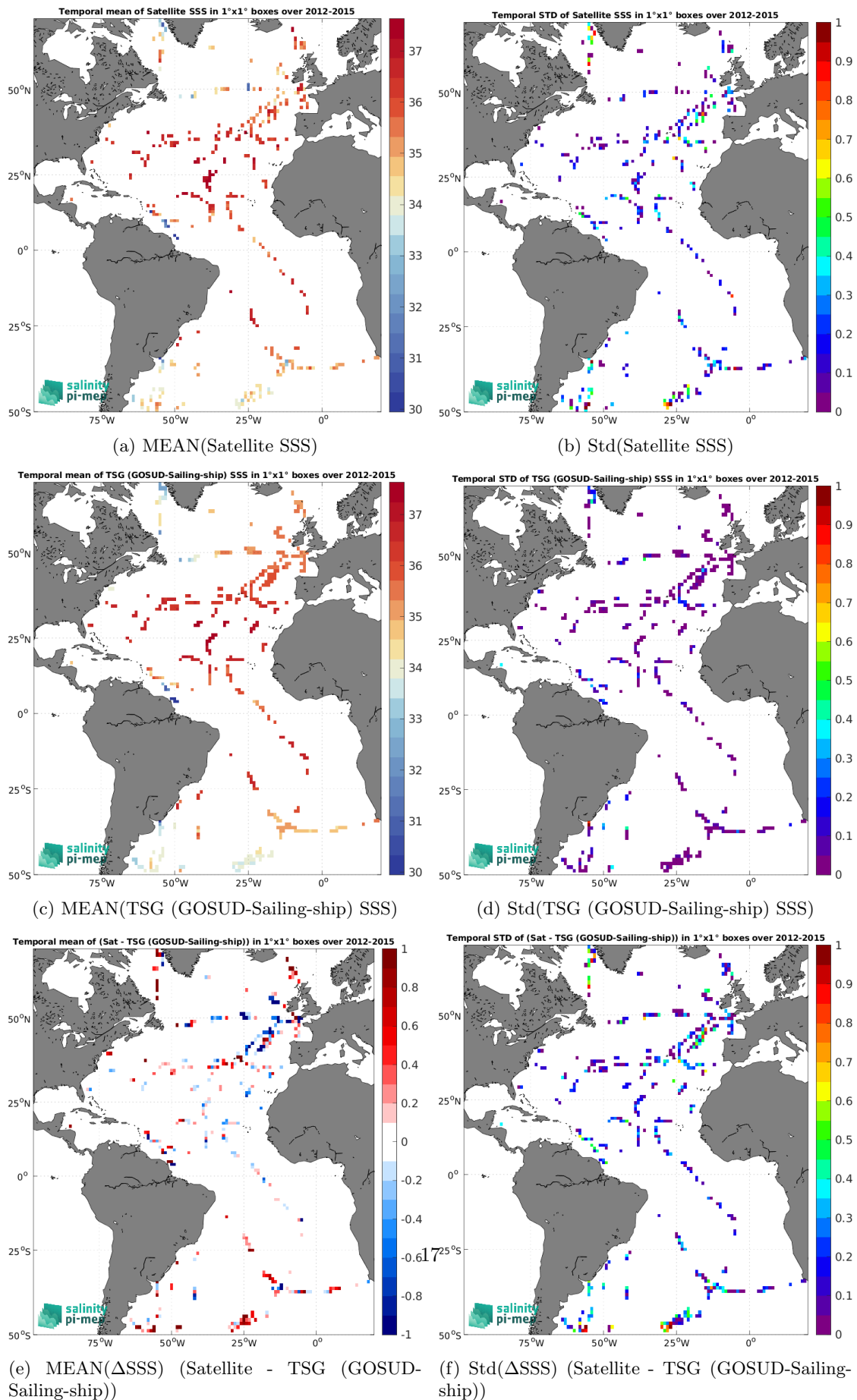
Figure 7: Temporal mean (left) and Std (right) of SSS from Aquarius SSS L2 CAP v5 (JPL) (top), TSG (GOSUD-Sailing-ship) (middle), and of \Delta SSS (Satellite - TSG (GOSUD-Sailing-ship)). Only match-up pairs are used to generate these maps.
