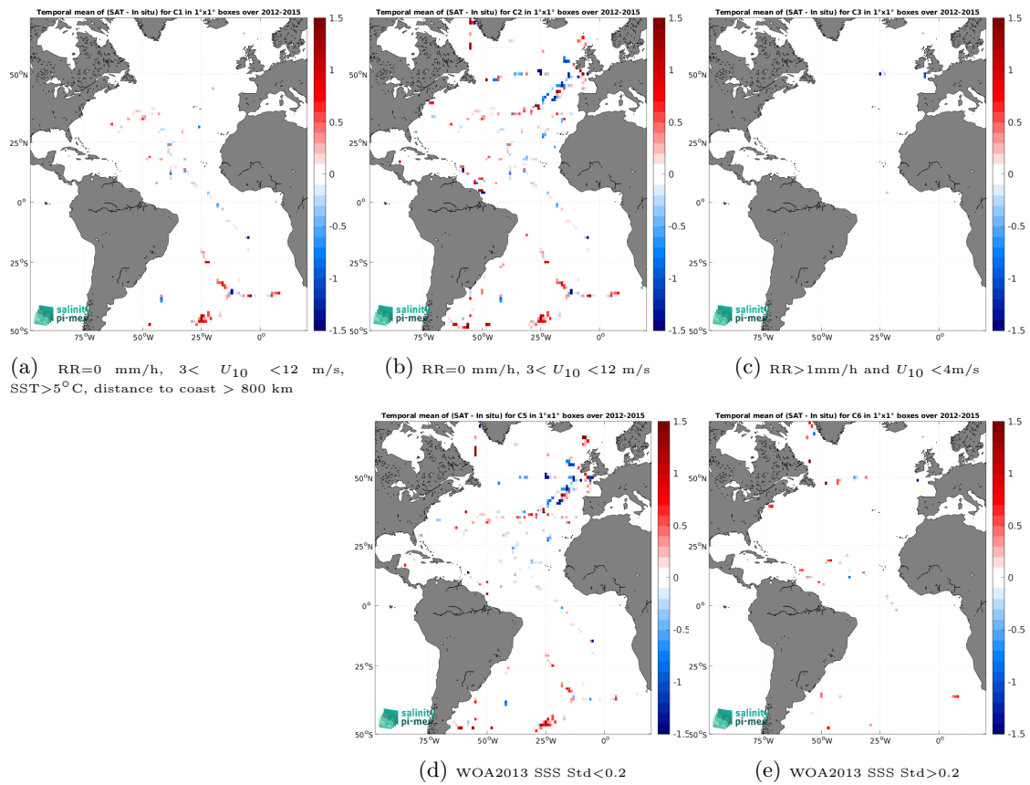
Figure 14: Temporal mean gridded over spatial boxes of size 1^\circ \times 1^\circ of \Delta\text{SSS} (Aquarius SSS L2 CAP v5 (JPL) - TSG (GOSUD-Sailing-ship)) for 5 different subdatasets corresponding to:RR=0 mm/h, 3 < U_{10} < 12 m/s, SST>5°C, distance to coast > 800 km (a), RR=0 mm/h, 3 < U_{10} < 12 m/s (b), RR>1mm/h and U_{10} < 4 m/s (c), WOA2013 SSS Std<0.2 (d), WOA2013 SSS Std>0.2 (e).
