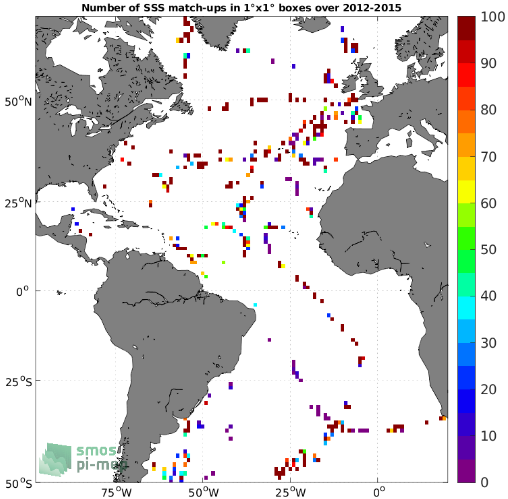
Figure 4: Number of SSS match-ups between TSG (GOSUD-Sailing-ship) SSS and the Aquarius SSS L2 CAP v5 (JPL) SSS product for the Atlantic Ocean Pi-MEP region over 1°×1° boxes and for the full satellite product period.
