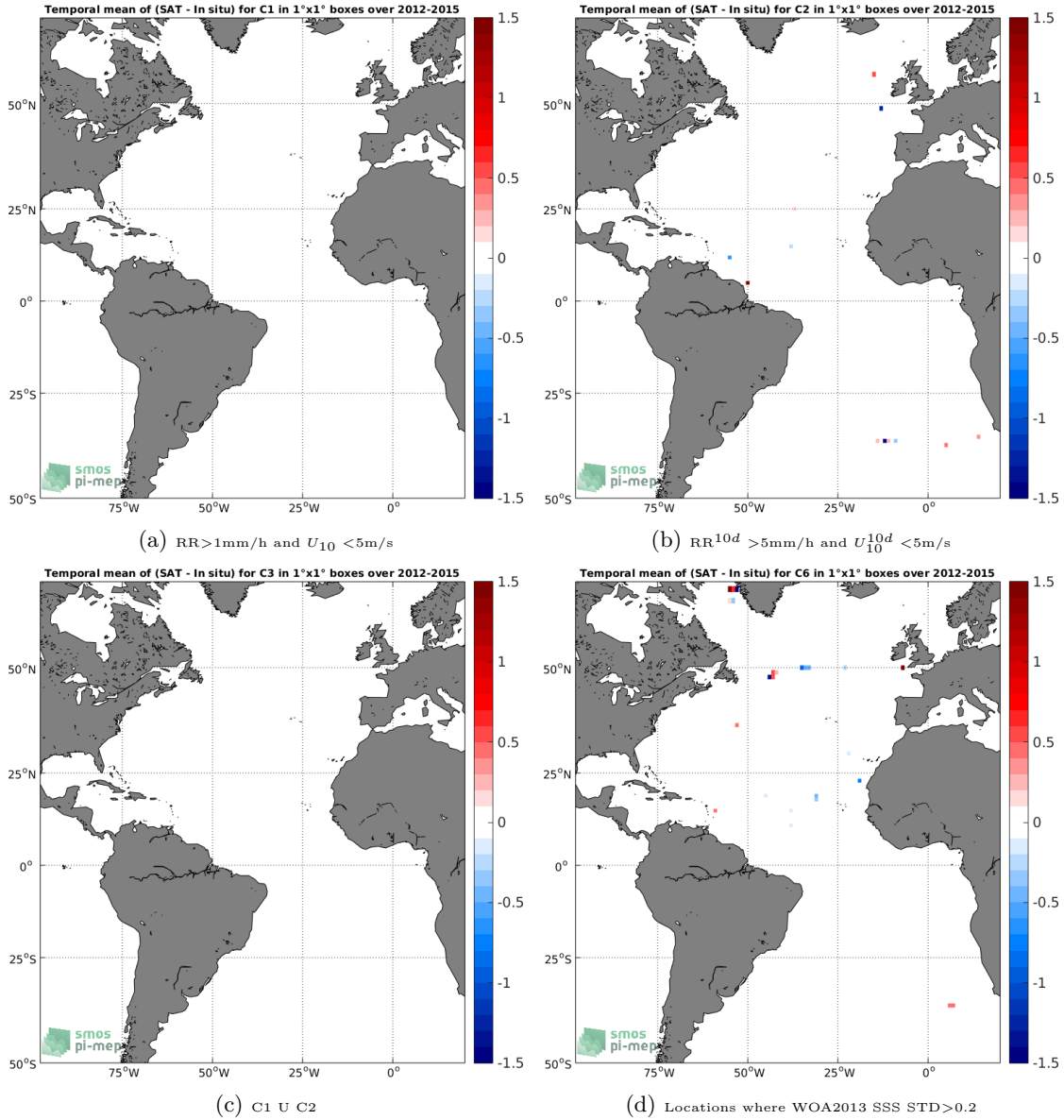
Figure 12: Temporal mean gridded over spatial boxes of size 1^\circ \times 1^\circ of \Delta SSS (Aquarius-L2-JPL-V5 - TSG-GOSUD-Sailing-ship) for 4 different subdatasets corresponding to:RR >1\text{mm/h} and U_{10} < 5\text{m/s} (a), RR^{10d} > 5\text{mm/h} and U_{10}^{10d} < 5\text{m/s} (b), C1 U C2 (c),Locations where WOA2013 SSS STD >0.2 (d).
