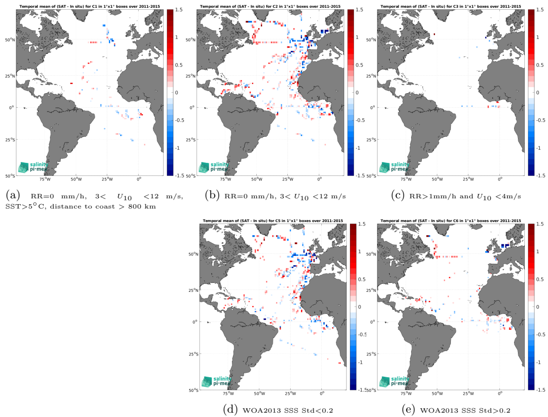
Figure 14: Temporal mean gridded over spatial boxes of size 1^\circ \times 1^\circ of \Delta SSS (Aquarius SSS L2 CAP v5 (JPL) - TSG (GOSUD-Research-vessel)) for 5 different subdatasets corresponding to:RR=0 mm/h, 3 < U_{10} < 12 m/s, SST >5^\circ\text{C} , distance to coast > 800 km (a), RR=0 mm/h, 3 < U_{10} < 12 m/s (b), RR >1 mm/h and U_{10} < 4 m/s (c), WOA2013 SSS Std <0.2 (d), WOA2013 SSS Std >0.2 (e).
