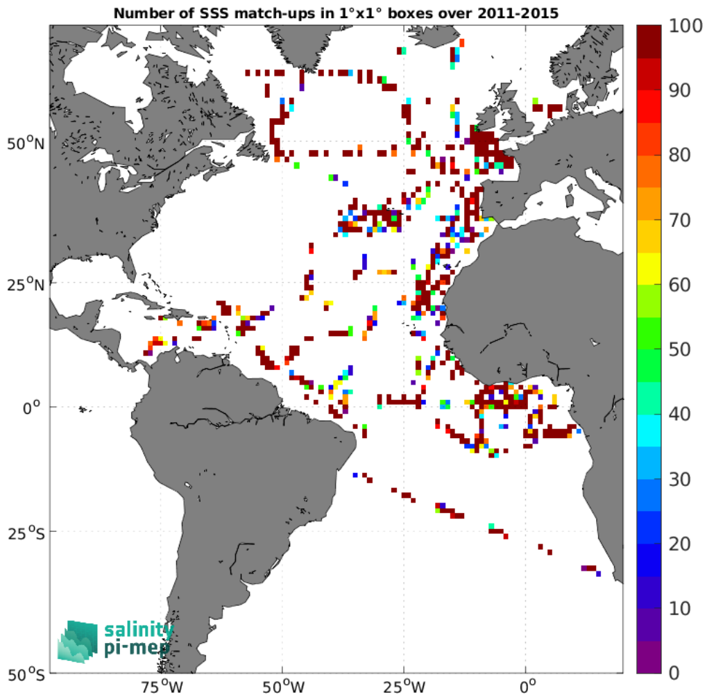
Figure 4: Number of SSS match-ups between TSG (GOSUD-Research-vessel) SSS and the Aquarius SSS L2 CAP v5 (JPL) SSS product for the Atlantic Ocean Pi-MEP region over 1^{\circ} \times 1^{\circ} boxes and for the full satellite product period.
