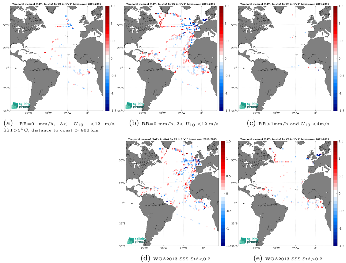
Figure 12: Temporal mean gridded over spatial boxes of size 1^\circ \times 1^\circ of \Delta SSS (Aquarius SSS L2 CAP v5 (JPL) - TSG (GOSUD-Research-vessel)) for 5 different subdatasets corresponding to:RR=0 mm/h, 3 < U_{10} < 12 m/s, SST >5^\circ\text{C} , distance to coast > 800 km (a), RR=0 mm/h, 3 < U_{10} < 12 m/s (b), RR >1 mm/h and U_{10} < 4 m/s (c), WOA2013 SSS Std <0.2 (d), WOA2013 SSS Std >0.2 (e).
