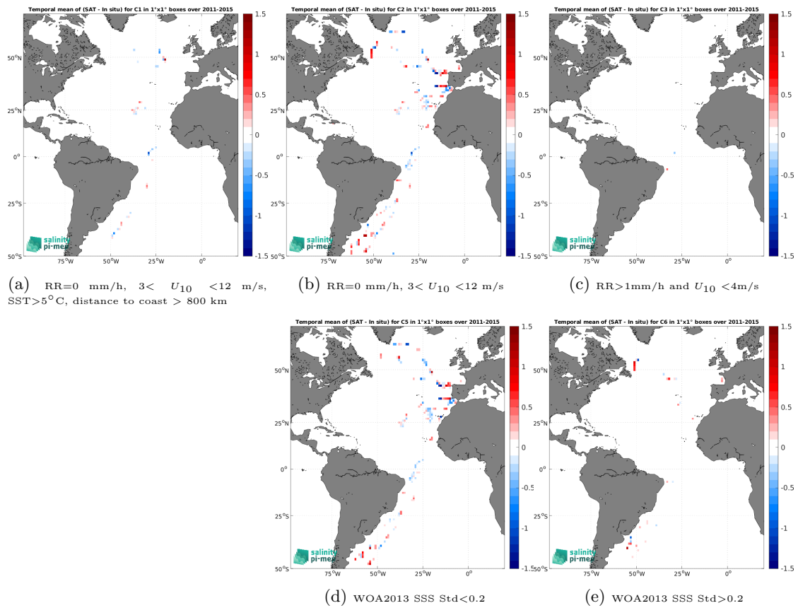
Figure 14: Temporal mean gridded over spatial boxes of size 1^\circ \times 1^\circ of \Delta SSS (Aquarius SSS L2 CAP v5 (JPL) - TSG (CSIC-UTM)) for 5 different subdatasets corresponding to:RR=0 mm/h, 3 < U_{10} < 12 m/s, SST >5^\circ\text{C} , distance to coast > 800 km (a), RR=0 mm/h, 3 < U_{10} < 12 m/s (b), RR >1 mm/h and U_{10} < 4 m/s (c), WOA2013 SSS Std <0.2 (d), WOA2013 SSS Std >0.2 (e).
