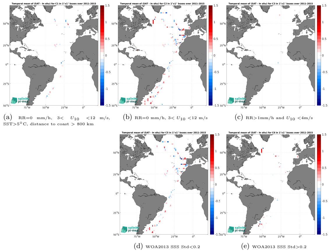
Figure 12: Temporal mean gridded over spatial boxes of size 1^\circ \times 1^\circ of \Delta SSS (Aquarius SSS L2 CAP v5 (JPL) - TSG (CSIC-UTM)) for 5 different subdatasets corresponding to:RR=0 mm/h, 3 < U_{10} < 12 m/s, SST >5^\circ\text{C} , distance to coast > 800 km (a), RR=0 mm/h, 3 < U_{10} < 12 m/s (b), RR >1 mm/h and U_{10} < 4 m/s (c), WOA2013 SSS Std <0.2 (d), WOA2013 SSS Std >0.2 (e).
