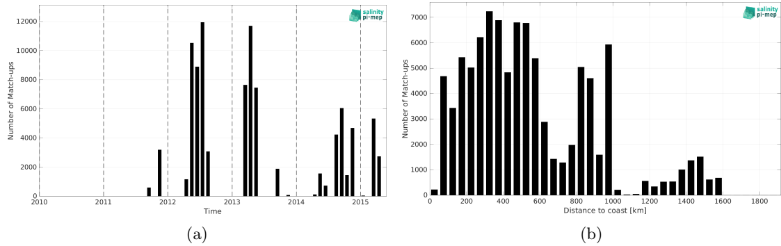
Figure 1: Number of match-ups between TSG (CSIC-UTM) and Aquarius SSS L2 CAP v5 (JPL) SSS as a function of time (a) and as function of the distance to coast (b) over the Atlantic Ocean Pi-MEP region and for the full satellite product period.
