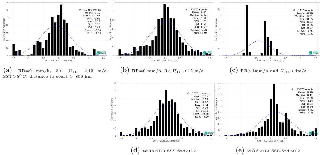
Figure 13: Normalized histogram of \Delta\text{SSS} (Aquarius SSS L2 CAP v5 (JPL) - TSG (CSIC-UTM)) for 5 different subdatasets corresponding to: RR=0 mm/h, 3 < U_{10} < 12 m/s, SST>5°C, distance to coast > 800 km (a), RR=0 mm/h, 3 < U_{10} < 12 m/s (b), RR>1mm/h and U_{10} < 4 m/s (c), WOA2013 SSS Std<0.2 (d), WOA2013 SSS Std>0.2 (e).
