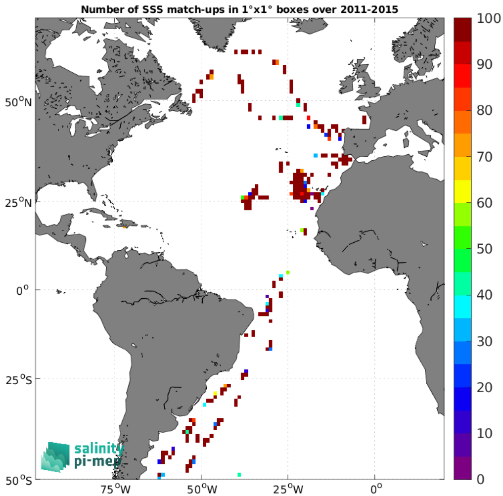
Figure 4: Number of SSS match-ups between TSG (CSIC-UTM) SSS and the Aquarius SSS L2 CAP v5 (JPL) SSS product for the Atlantic Ocean Pi-MEP region over 1^\circ \times 1^\circ boxes and for the full satellite product period.
