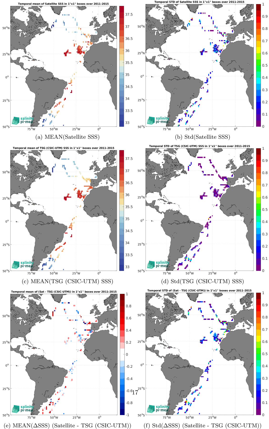
Figure 6: Temporal mean (left) and Std (right) of SSS from Aquarius SSS L2 CAP v5 (JPL) (top), TSG (CSIC-UTM) (middle), and of \Delta SSS (Satellite - TSG (CSIC-UTM)). Only match-up pairs are used to generate these maps.
