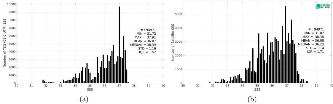
Figure 2: Histograms of SSS from TSG (CSIC-UTM) (a) and Aquarius SSS L2 CAP v5 (JPL) (b) considering all match-up pairs per bins of 0.1 over the Atlantic Ocean Pi-MEP region and for the full satellite product period.
