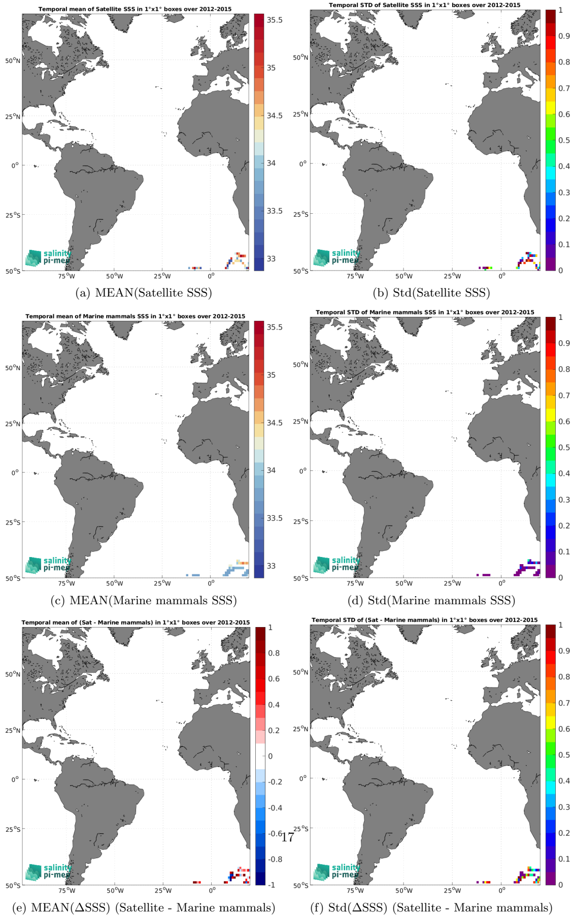
Figure 6: Temporal mean (left) and Std (right) of SSS from Aquarius SSS L2 CAP v5 (JPL) (top), Marine mammals (middle), and of \Delta SSS (Satellite - Marine mammals). Only match-up pairs are used to generate these maps.
