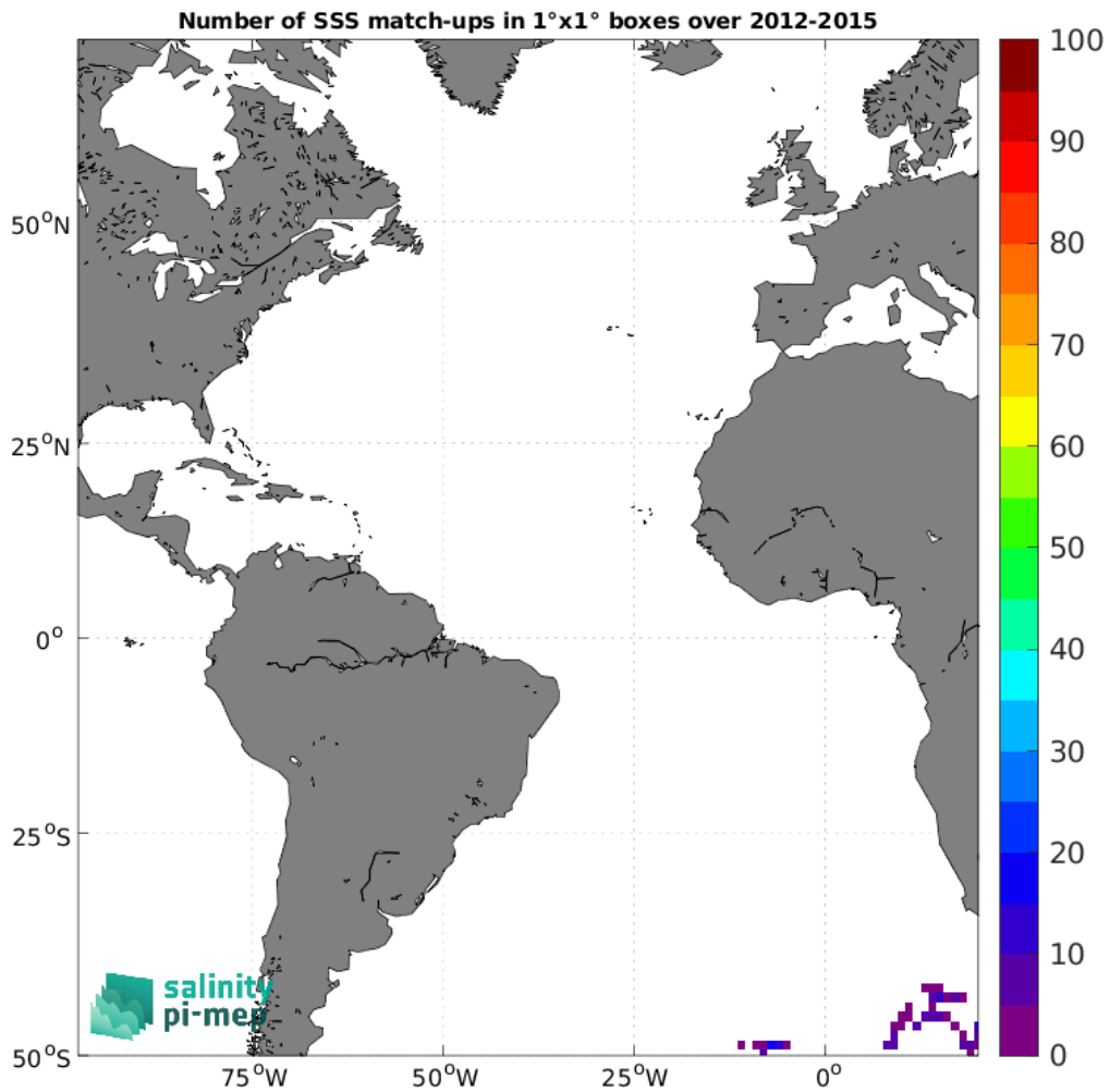
Figure 4: Number of SSS match-ups between Marine mammals SSS and the Aquarius SSS L2 CAP v5 (JPL) SSS product for the Atlantic Ocean Pi-MEP region over 1^{\circ} \times 1^{\circ} boxes and for the full satellite product period.
