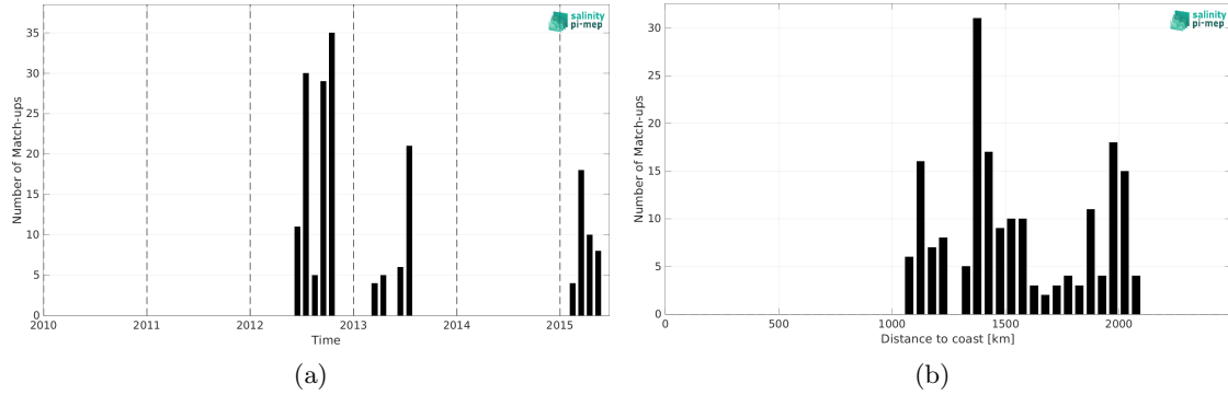
Figure 1: Number of match-ups between Marine mammals and Aquarius SSS L2 CAP v5 (JPL) SSS as a function of time (a) and as function of the distance to coast (b) over the Atlantic Ocean Pi-MEP region and for the full satellite product period.
