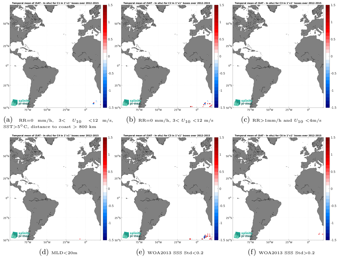
Figure 12: Temporal mean gridded over spatial boxes of size 1^\circ \times 1^\circ of \Delta\text{SSS} (Aquarius SSS L2 CAP v5 (JPL) - Marine mammals) for 6 different subdatasets corresponding to: RR=0 mm/h, 3 < U_{10} < 12 m/s, SST > 5^\circ\text{C} , distance to coast > 800 km (a), RR=0 mm/h, 3 < U_{10} < 12 m/s (b), RR > 1\text{mm/h} and U_{10} < 4\text{m/s} (c), MLD < 20\text{m} (d), WOA2013 SSS Std < 0.2 (e), WOA2013 SSS Std > 0.2 (f).
