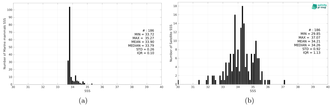
Figure 2: Histograms of SSS from Marine mammals (a) and Aquarius SSS L2 CAP v5 (JPL) (b) considering all match-up pairs per bins of 0.1 over the Atlantic Ocean Pi-MEP region and for the full satellite product period.
