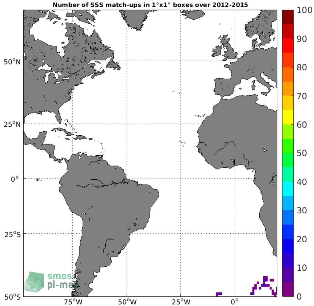
Figure 4: Number of SSS match-ups between Sea mammals SSS and the Aquarius SSS L2 CAP v5 (JPL) SSS product for the Atlantic Ocean Pi-MEP region over 1°x1° boxes and for the full satellite product period.
