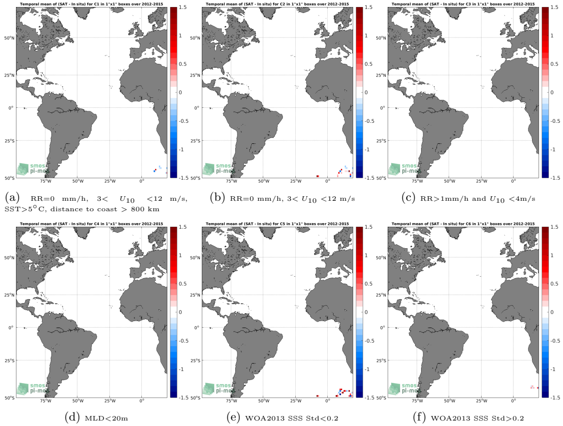
Figure 12: Temporal mean gridded over spatial boxes of size 1^\circ \times 1^\circ of \Delta\text{SSS} (Aquarius SSS L2 CAP v5 (JPL) - Sea mammals) for 6 different subdatasets corresponding to: RR=0 mm/h, 3 < U_{10} < 12 m/s, SST > 5^\circ\text{C} , distance to coast > 800 km (a), RR=0 mm/h, 3 < U_{10} < 12 m/s (b), RR > 1 mm/h and U_{10} < 4 m/s (c), MLD < 20 m (d), WOA2013 SSS Std < 0.2 (e), WOA2013 SSS Std > 0.2 (f).
