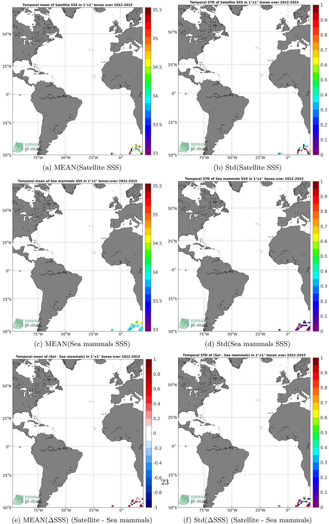
Figure 6: Temporal mean (left) and Std (right) of SSS from Aquarius SSS L2 CAP v5 (JPL) (top), Sea mammals (middle), and of \Delta SSS (Satellite - Sea mammals). Only match-up pairs are used to generate these maps.
