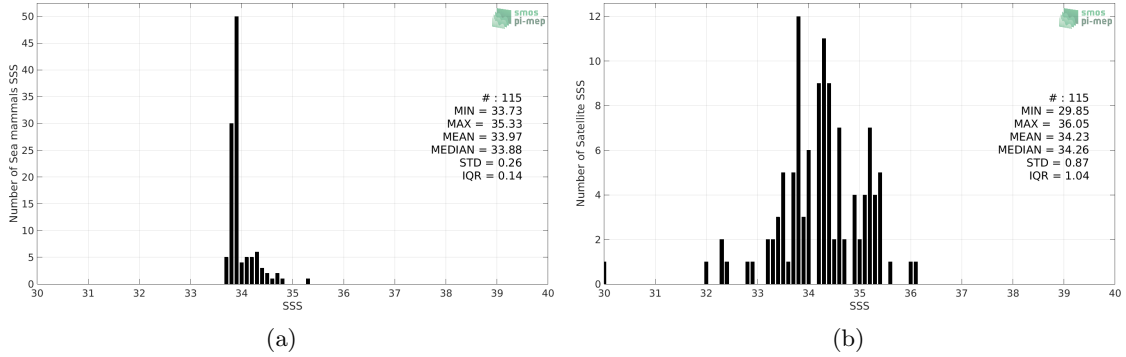
Figure 2: Histograms of SSS from Sea mammals (a) and Aquarius SSS L2 CAP v5 (JPL) (b) considering all match-up pairs per bins of 0.1 over the Atlantic Ocean Pi-MEP region and for the full satellite product period.
