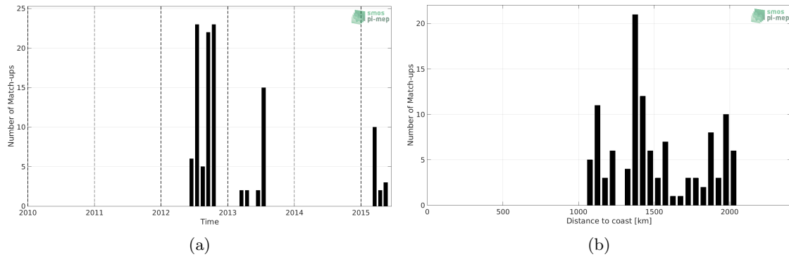
Figure 1: Number of match-ups between Sea mammals and Aquarius SSS L2 CAP v5 (JPL) SSS as a function of time (a) and as function of the distance to coast (b) over the Atlantic Ocean Pi-MEP region and for the full satellite product period.
