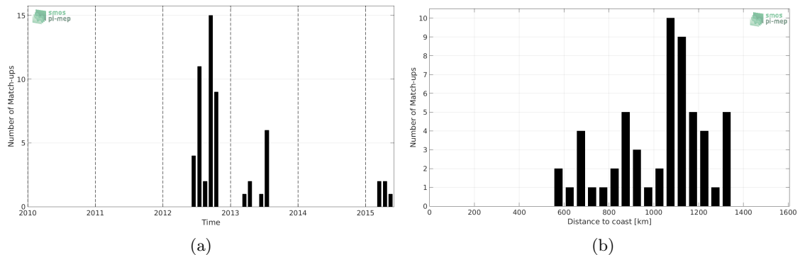
Figure 1: Number of match-ups between Sea mammals and Aquarius-L2-JPL-V5 SSS as a function of time (a) and as function of the distance to coast (b) over the Atlantic Ocean Pi-MEP region and for the full satellite product period.
