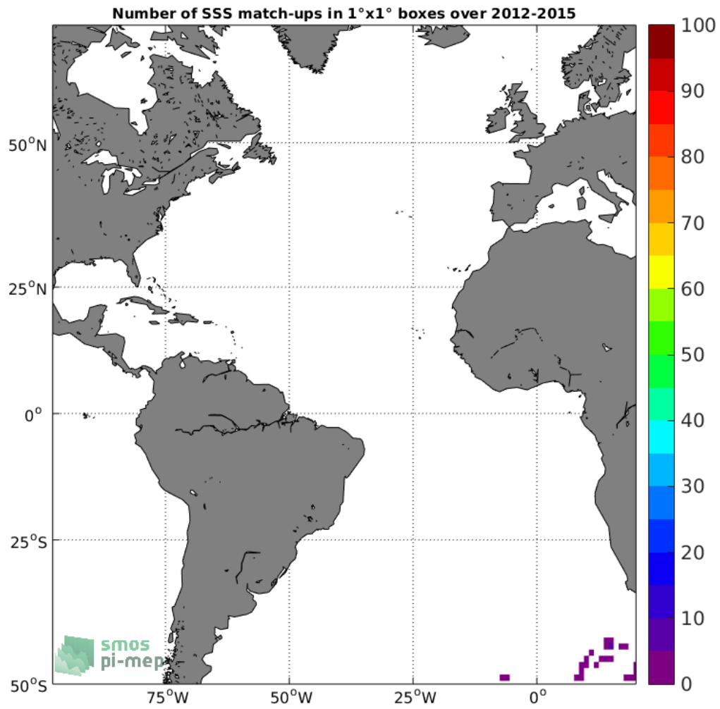
Figure 4: Number of SSS match-ups between Sea mammals SSS and the Aquarius-L2-JPL-V5 SSS product for the Atlantic Ocean Pi-MEP region over 1°x1° boxes and for the full satellite product period.
