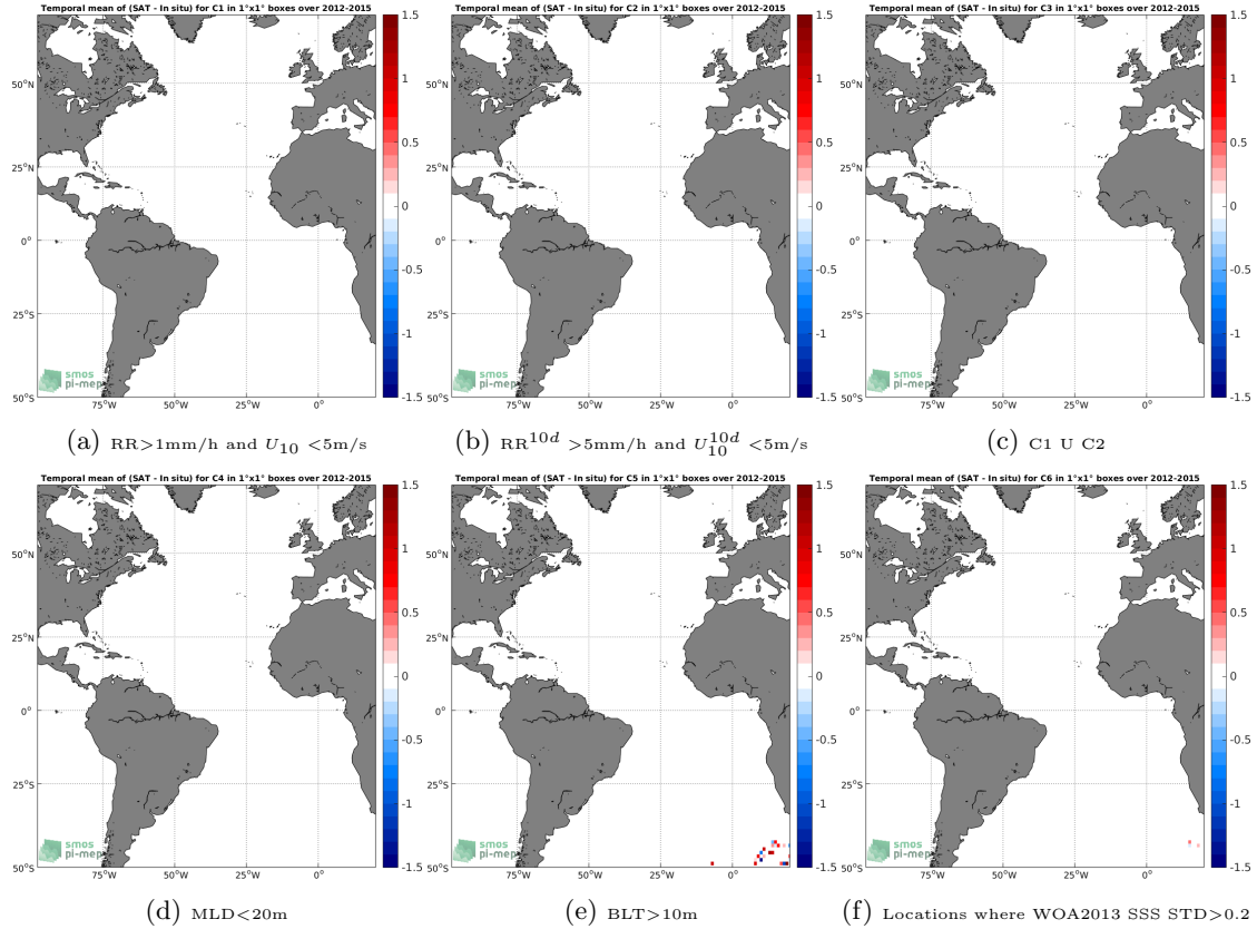
Figure 12: Temporal mean gridded over spatial boxes of size 1^\circ \times 1^\circ of \Delta\text{SSS} (Aquarius-L2-JPL-V5 - Sea mammals) for 6 different subdatasets corresponding to: \text{RR} > 1\text{mm/h} and U_{10} < 5\text{m/s} (a), \text{RR}^{10d} > 5\text{mm/h} and U_{10}^{10d} < 5\text{m/s} (b), C1 U C2 (c), \text{MLD} < 20\text{m} (d), \text{BLT} > 10\text{m} (e), Locations where WOA2013 SSS STD > 0.2 (f).
