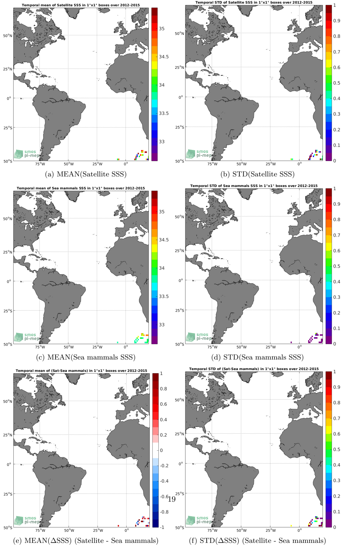
Figure 6: Temporal mean (left) and STD (right) of SSS from Aquarius-L2-JPL-V5 (top), Sea mammals (middle), and of \Delta SSS (Satellite - Sea mammals). Only match-up pairs are used to generate these maps.
