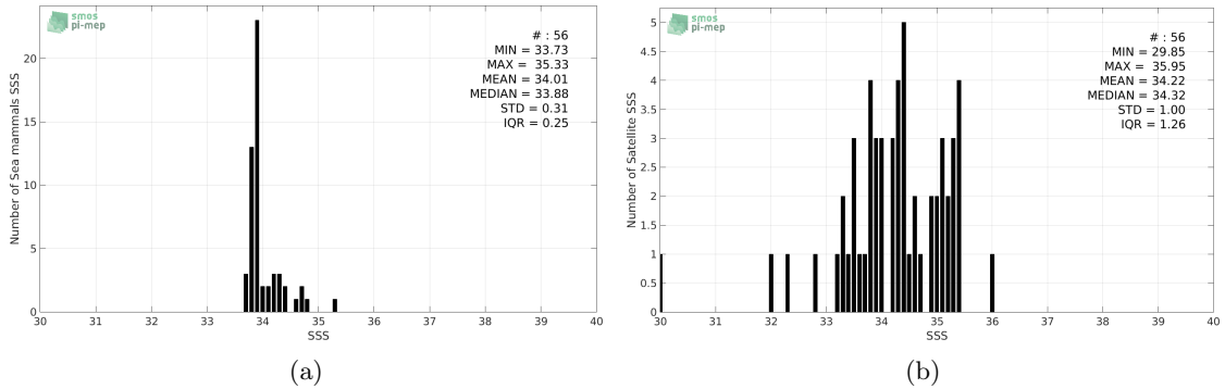
Figure 2: Histograms of SSS from Sea mammals (a) and Aquarius-L2-JPL-V5 (b) considering all match-up pairs per bins of 0.1 over the Atlantic Ocean Pi-MEP region and for the full satellite product period.
