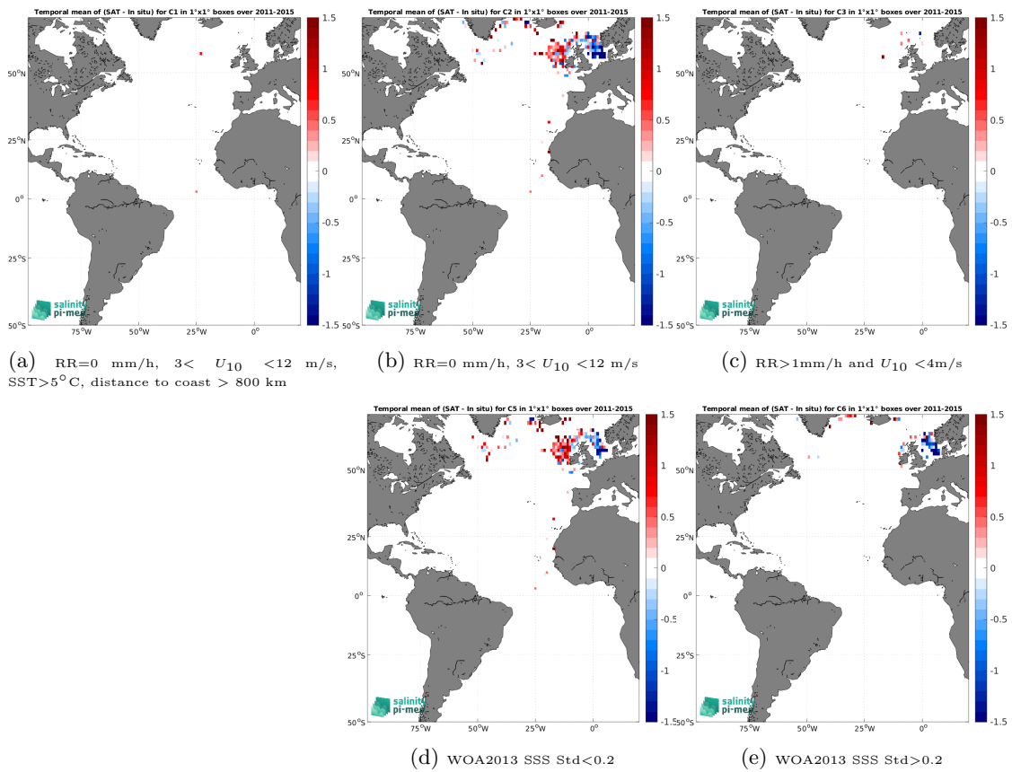
Figure 14: Temporal mean gridded over spatial boxes of size 1^\circ \times 1^\circ of \Delta SSS (Aquarius SSS L2 CAP v5 (JPL) - ICES) for 5 different subdatasets corresponding to:RR=0 mm/h, 3 < U_{10} < 12 m/s, SST >5^\circ\text{C} , distance to coast > 800 km (a), RR=0 mm/h, 3 < U_{10} < 12 m/s (b), RR >1 mm/h and U_{10} < 4 m/s (c), WOA2013 SSS Std <0.2 (d), WOA2013 SSS Std >0.2 (e).
