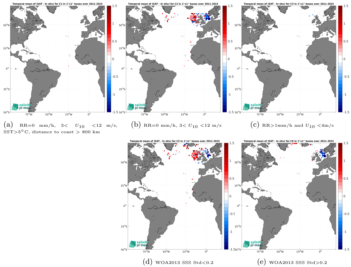
Figure 12: Temporal mean gridded over spatial boxes of size 1^\circ \times 1^\circ of \Delta SSS (Aquarius SSS L2 CAP v5 (JPL) - ICES) for 5 different subdatasets corresponding to:RR=0 mm/h, 3 < U_{10} < 12 m/s, SST >5^\circ\text{C} , distance to coast > 800 km (a), RR=0 mm/h, 3 < U_{10} < 12 m/s (b), RR >1 mm/h and U_{10} < 4 m/s (c), WOA2013 SSS Std <0.2 (d), WOA2013 SSS Std >0.2 (e).
