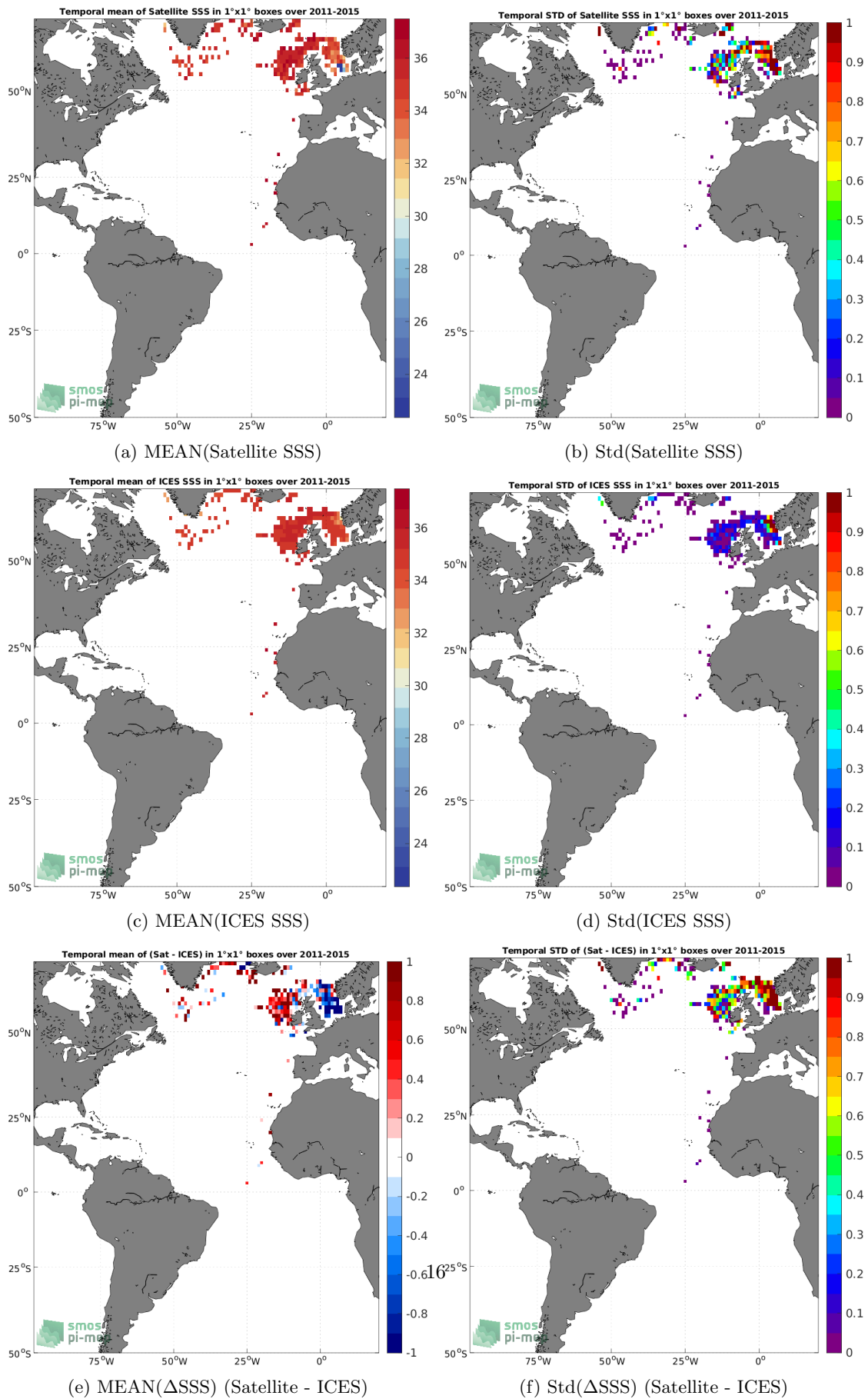
Figure 6: Temporal mean (left) and Std (right) of SSS from Aquarius SSS L2 CAP v5 (JPL) (top), ICES (middle), and of \Delta SSS (Satellite - ICES). Only match-up pairs are used to generate these maps.
