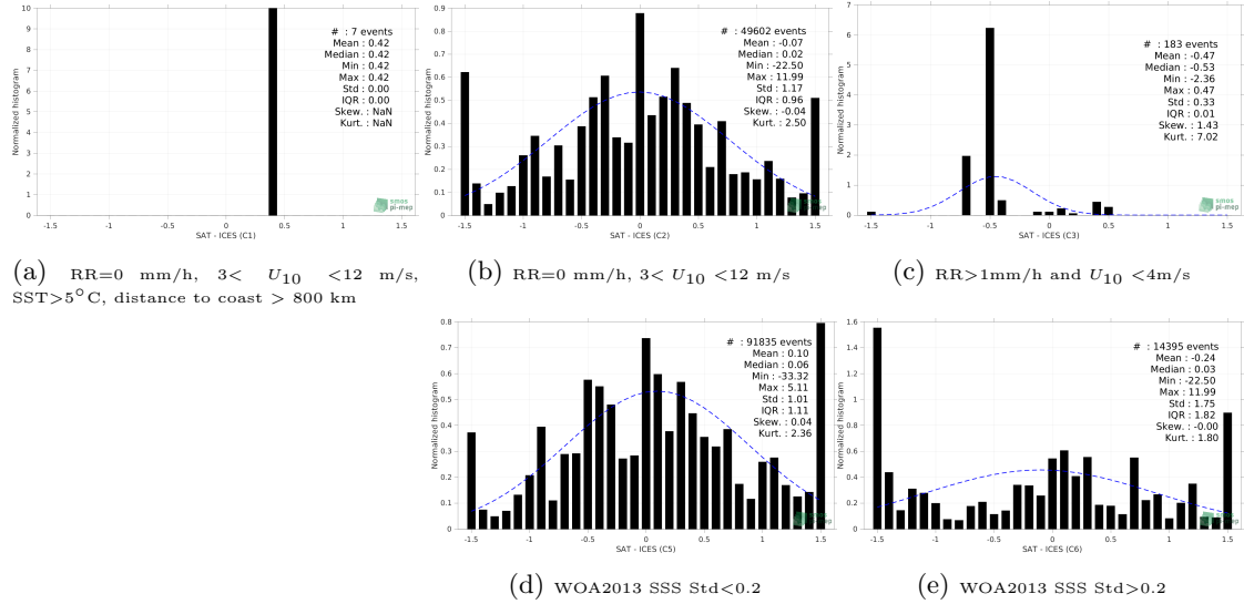
Figure 13: Normalized histogram of \Delta SSS (Aquarius SSS L2 CAP v5 (JPL) - ICES) for 5 different subdatasets corresponding to: RR=0 mm/h, 3 < U_{10} < 12 m/s, SST > 5°C, distance to coast > 800 km (a), RR=0 mm/h, 3 < U_{10} < 12 m/s (b), RR > 1mm/h and U_{10} < 4 m/s (c), WOA2013 SSS Std < 0.2 (d), WOA2013 SSS Std > 0.2 (e).
