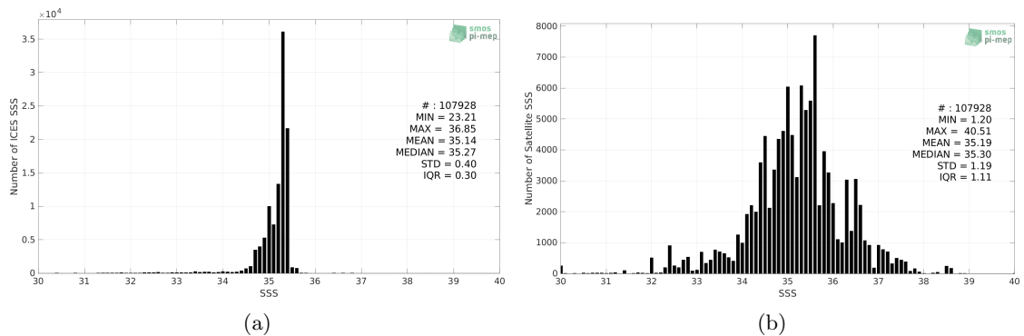
Figure 2: Histograms of SSS from ICES (a) and Aquarius SSS L2 CAP v5 (JPL) (b) considering all match-up pairs per bins of 0.1 over the Atlantic Ocean Pi-MEP region and for the full satellite product period.
