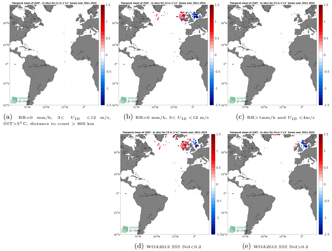
Figure 12: Temporal mean gridded over spatial boxes of size 1^\circ \times 1^\circ of \Delta SSS (Aquarius SSS L2 CAP v5 (JPL) - ICES) for 5 different subdatasets corresponding to:RR=0 mm/h, 3 < U_{10} < 12 m/s, SST>5°C, distance to coast > 800 km (a), RR=0 mm/h, 3 < U_{10} < 12 m/s (b), RR>1mm/h and U_{10} < 4 m/s (c), WOA2013 SSS Std<0.2 (d), WOA2013 SSS Std>0.2 (e).
