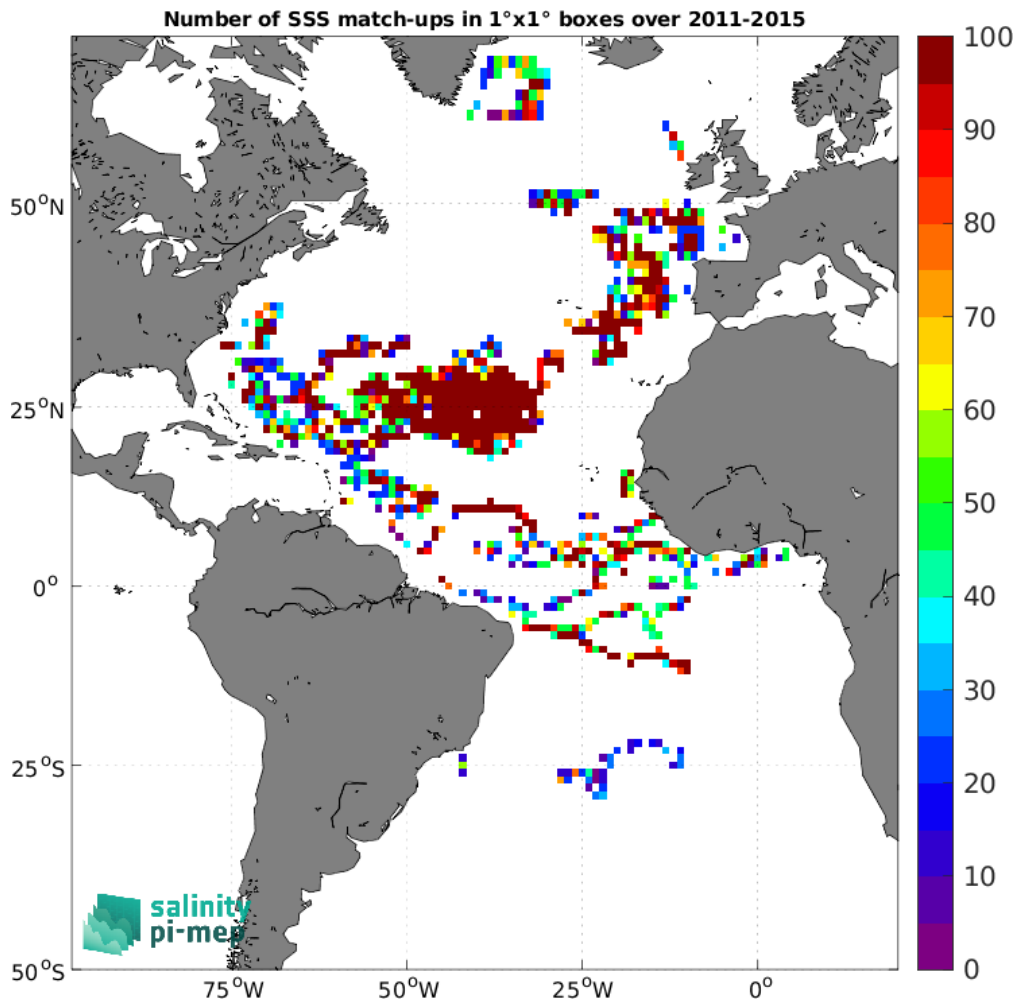
Figure 4: Number of SSS match-ups between Surface drifters SSS and the Aquarius SSS L2 CAP v5 (JPL) SSS product for the Atlantic Ocean Pi-MEP region over 1°×1° boxes and for the full satellite product period.
