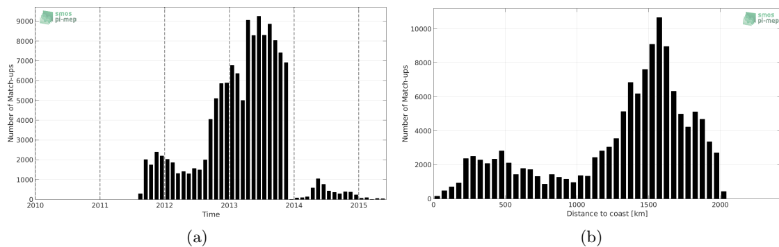
Figure 1: Number of match-ups between Surface drifters and Aquarius-L2-JPL-V5 SSS as a function of time (a) and as function of the distance to coast (b) over the Atlantic Ocean Pi-MEP region and for the full satellite product period.
