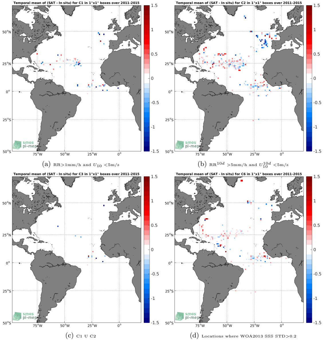
Figure 11: Temporal mean gridded over spatial boxes of size 1^\circ \times 1^\circ of \Delta SSS (Aquarius-L2-JPL-V5 - Surface drifters) for 4 different subdatasets corresponding to: RR > 1mm/h and U_{10} < 5\text{m/s} (a), RR^{10d} > 5\text{mm/h} and U_{10}^{10d} < 5\text{m/s} (b), C1 U C2 (c), Locations where WOA2013 SSS STD > 0.2 (d).
