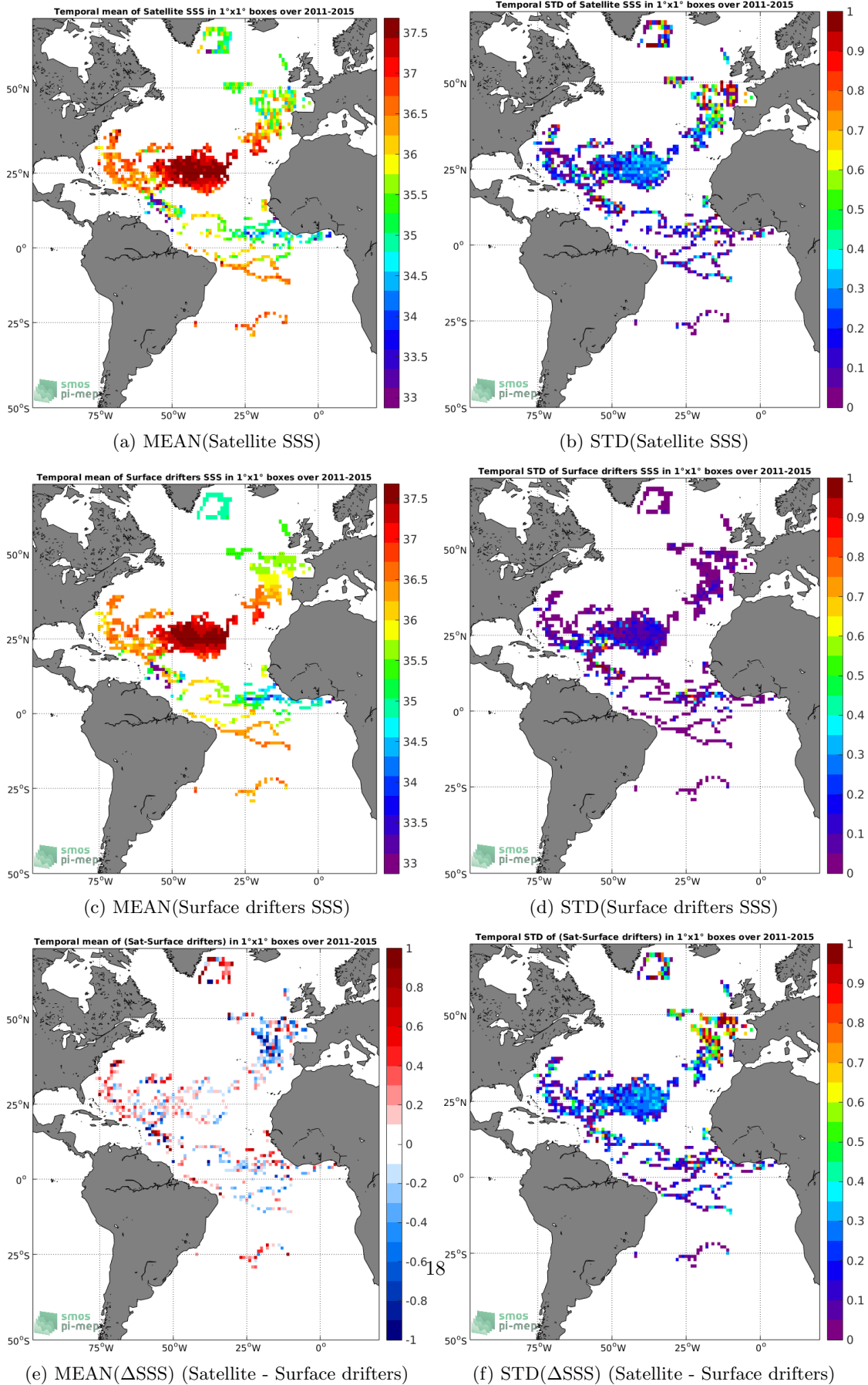
(e) MEAN( \Delta SSS) (Satellite - Surface drifters) (f) STD( \Delta SSS) (Satellite - Surface drifters) Figure 5: Temporal mean (left) and STD (right) of SSS from Aquarius-L2-JPL-V5 (top), Surface drifters (middle), and of \Delta SSS (Satellite - Surface drifters). Only match-up pairs are used to generate these maps.
