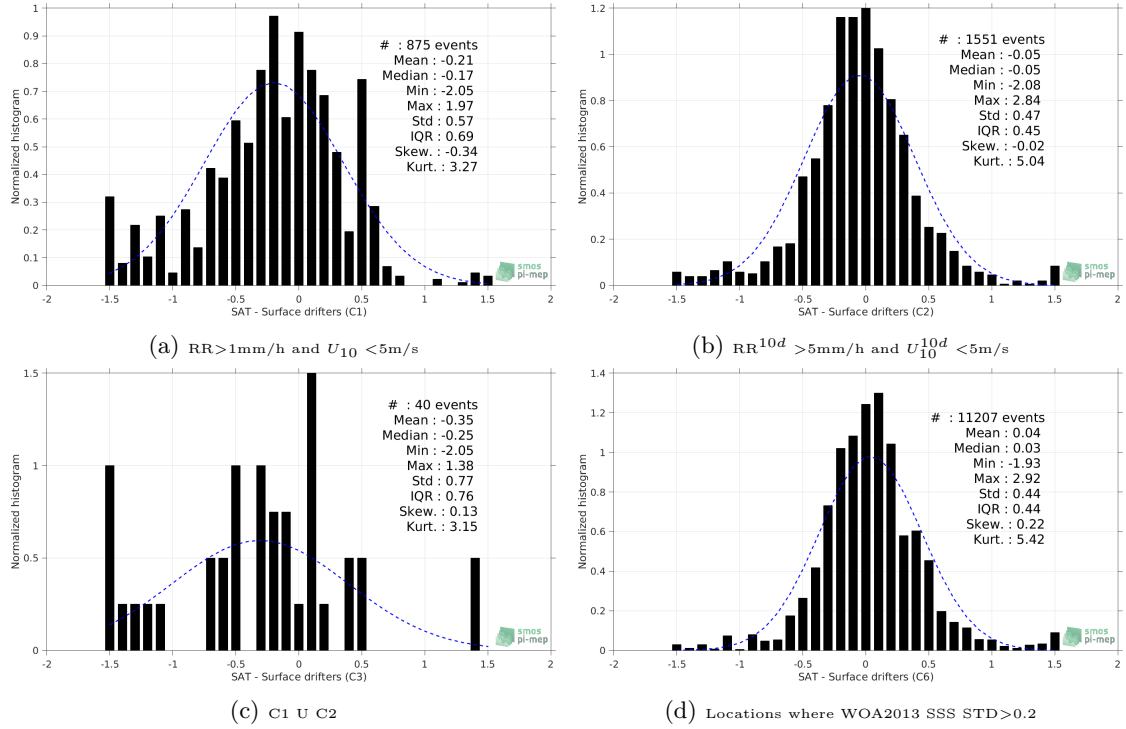
Figure 12: Normalized histogram of \Delta\text{SSS} (Aquarius-L2-JPL-V5 - Surface drifters) for 6 different subdatasets corresponding to: RR > 1mm/h and U_{10} < 5\text{m/s} (a), \text{RR}^{10d} > 5\text{mm/h} and U_{10}^{10d} < 5\text{m/s} (b), C1 U C2 (c), Locations where WOA2013 SSS STD > 0.2 (d).
