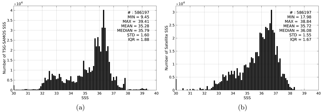
Figure 2: Histograms of SSS from TSG-SAMOS (a) and AQUARIUS-L2-JPL-V4 (b) considering all match-up pairs per bins of 0.1 over the Atlantic Ocean Pi-MEP region and for the full satellite product period.
