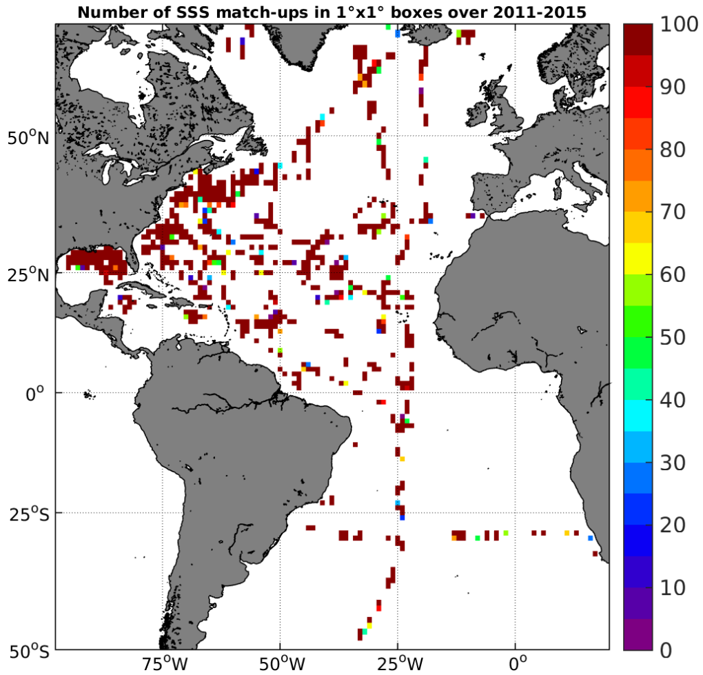
Figure 4: Number of SSS match-ups between TSG-SAMOS SSS and the AQUARIUS-L2-JPL-V4 SSS product for the Atlantic Ocean Pi-MEP region over 1°x1° boxes and for the full satellite product period.
