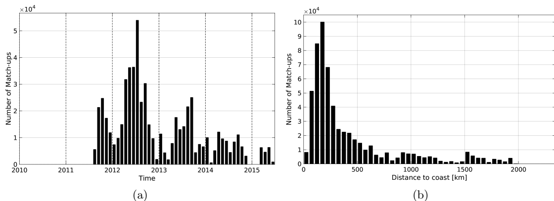
Figure 1: Number of match-ups between TSG-SAMOS and AQUARIUS-L2-JPL-V4 SSS as a function of time (a) and as function of the distance to coast (b) over the Atlantic Ocean Pi-MEP region and for the full satellite product period.
