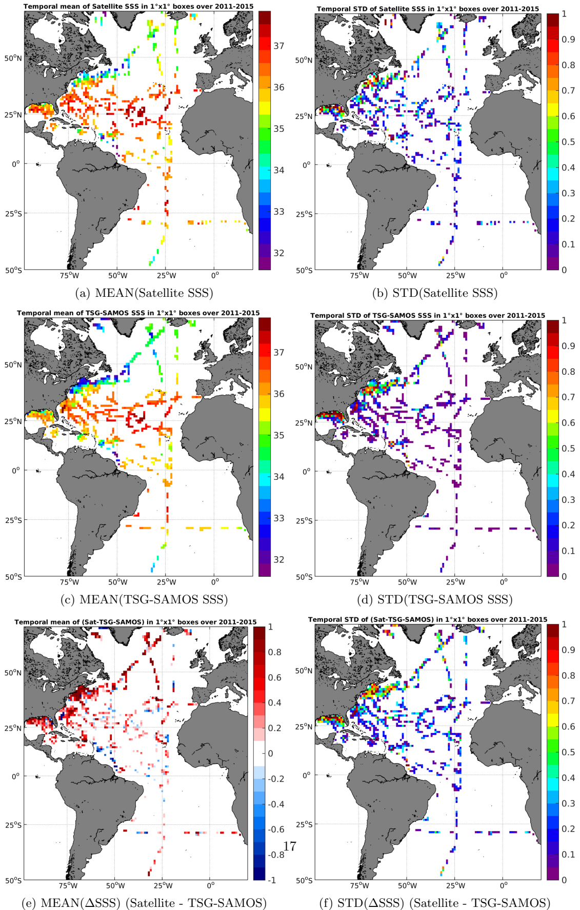
Figure 6: Temporal mean (left) and STD (right) of SSS from AQUARIUS-L2-JPL-V4 (top), TSG-SAMOS (middle), and of \Delta SSS (Satellite - TSG-SAMOS). Only match-up pairs are used to generate these maps.
