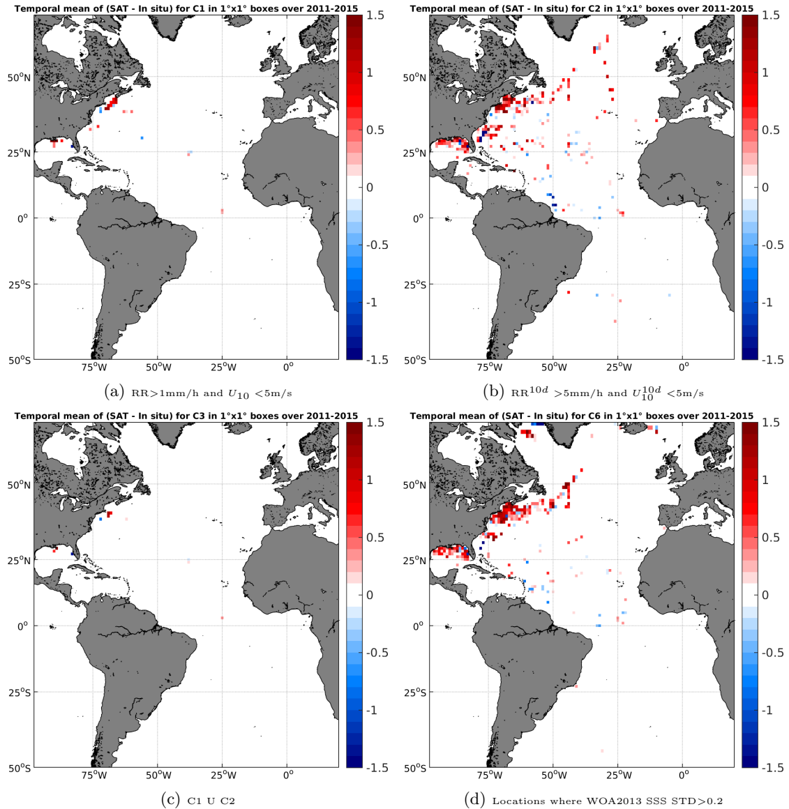
Figure 12: Temporal mean gridded over spatial boxes of size 1^\circ \times 1^\circ of \Delta SSS (AQUARIUS-L2-JPL-V4 - TSG-SAMOS) for 4 different subdatasets corresponding to:RR >1 mm/h and U_{10} < 5 m/s (a), RR^{10d} > 5 mm/h and U_{10}^{10d} < 5 m/s (b), C1 U C2 (c),Locations where WOA2013 SSS STD >0.2 (d).
