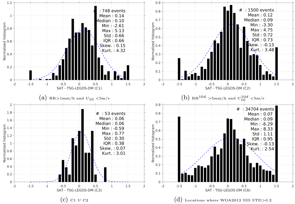
Figure 13: Normalized histogram of \Delta SSS (AQUARIUS-L2-JPL-V4 - TSG-LEGOS-DM) for 6 different subdatasets corresponding to: RR > 1\text{mm/h} and U_{10} < 5\text{m/s} (a), RR^{10d} > 5\text{mm/h} and U_{10}^{10d} < 5\text{m/s} (b), C1 U C2 (c), Locations where WOA2013 SSS STD > 0.2 (d).
