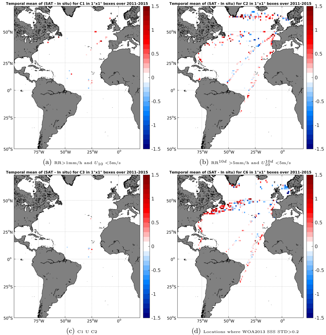
Figure 12: Temporal mean gridded over spatial boxes of size 1^\circ \times 1^\circ of \Delta SSS (AQUARIUS-L2-JPL-V4 - TSG-LEGOS-DM) for 4 different subdatasets corresponding to: RR > 1\text{mm/h} and U_{10} < 5\text{m/s} (a), RR^{10d} > 5\text{mm/h} and U_{10}^{10d} < 5\text{m/s} (b), C1 U C2 (c), Locations where WOA2013 SSS STD > 0.2 (d).
