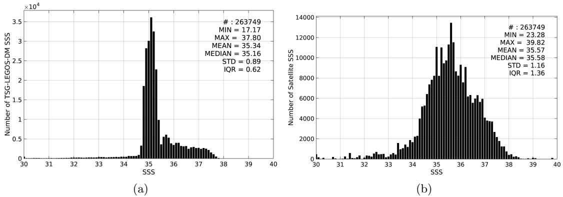
Figure 2: Histograms of SSS from TSG-LEGOS-DM (a) and AQUARIUS-L2-JPL-V4 (b) considering all match-up pairs per bins of 0.1 over the Atlantic Ocean Pi-MEP region and for the full satellite product period.
