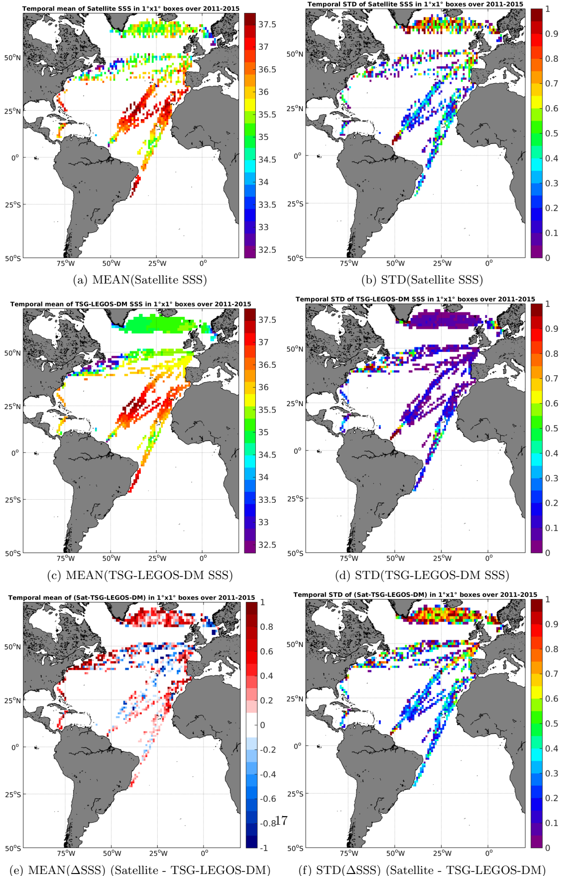
Figure 6: Temporal mean (left) and STD (right) of SSS from AQUARIUS-L2-JPL-V4 (top), TSG-LEGOS-DM (middle), and of \Delta SSS (Satellite - TSG-LEGOS-DM). Only match-up pairs are used to generate these maps.
