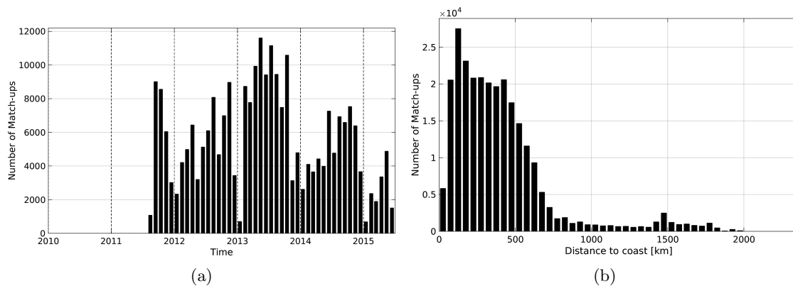
Figure 1: Number of match-ups between TSG-LEGOS-DM and AQUARIUS-L2-JPL-V4 SSS as a function of time (a) and as function of the distance to coast (b) over the Atlantic Ocean Pi-MEP region and for the full satellite product period.
