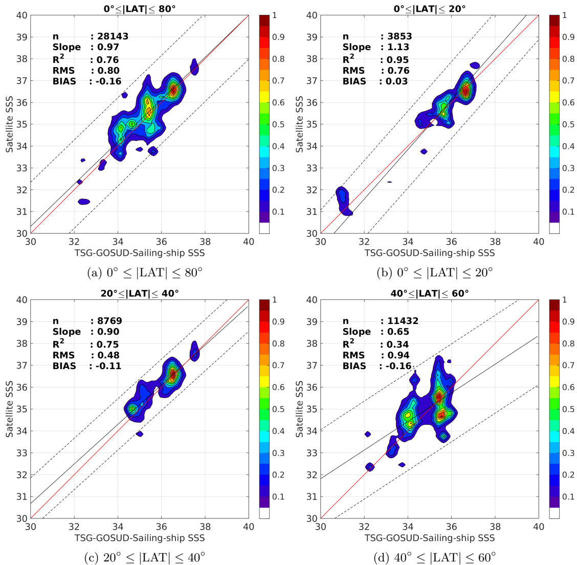
Figure 9: Contour maps of the concentration of AQUARIUS-L2-JPL-V4 SSS (y-axis) versus TSG-GOSUD-Sailing-ship SSS (x-axis) at match-up pairs for different latitude bands. For each plot, the red line shows x=y . The black thin and dashed lines indicate a linear fit through the data cloud and the \pm 95\% confidence levels, respectively. The number match-up pairs n , the slope and R^2 coefficient of the linear fit, the root mean square (RMS) and the mean bias between satellite and in situ data are indicated for each latitude band in each plots.
