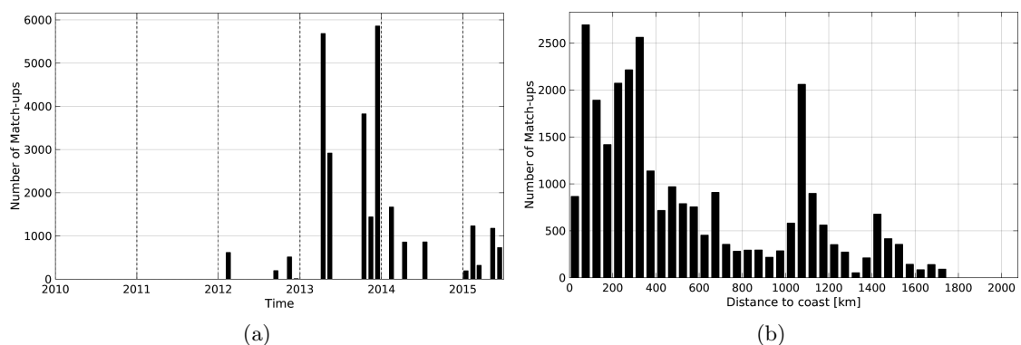
Figure 1: Number of match-ups between TSG-GOSUD-Sailing-ship and AQUARIUS-L2-JPL-V4 SSS as a function of time (a) and as function of the distance to coast (b) over the Atlantic Ocean Pi-MEP region and for the full satellite product period.
