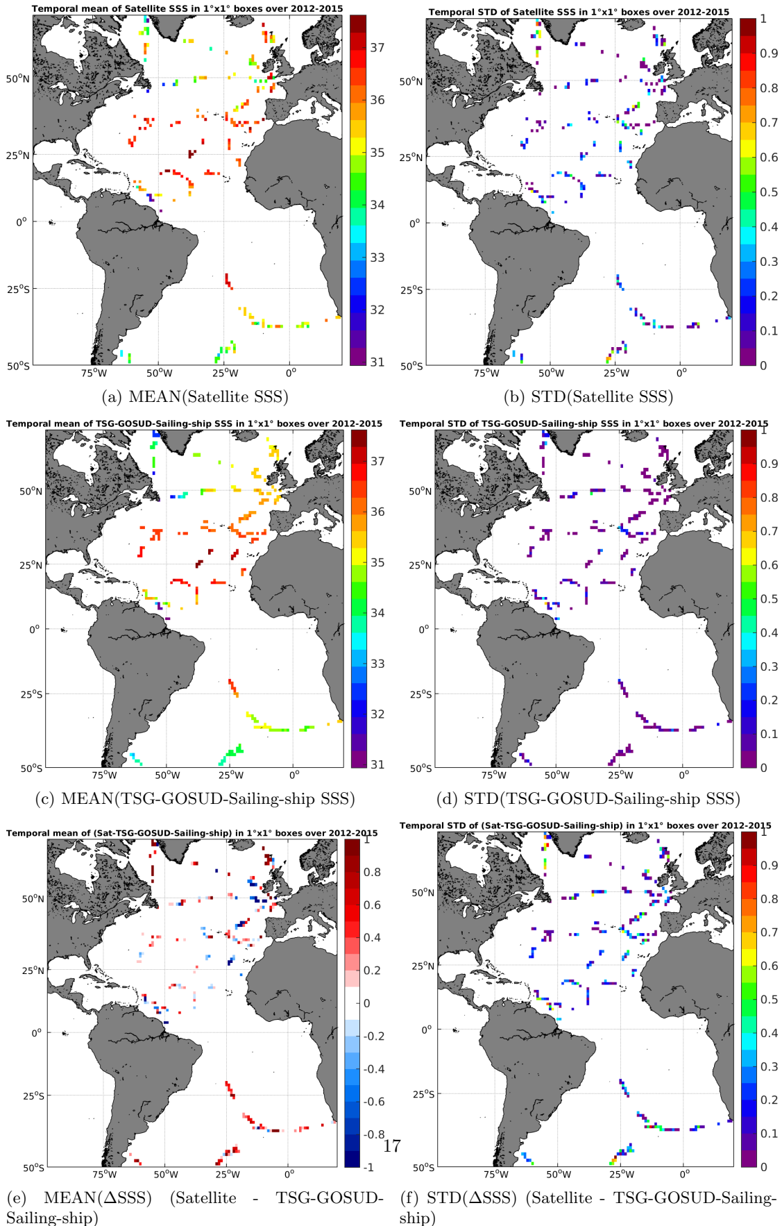
Figure 6: Temporal mean (left) and STD (right) of SSS from AQUARIUS-L2-JPL-V4 (top), TSG-GOSUD-Sailing-ship (middle), and of \Delta SSS (Satellite - TSG-GOSUD-Sailing-ship). Only match-up pairs are used to generate these maps.
