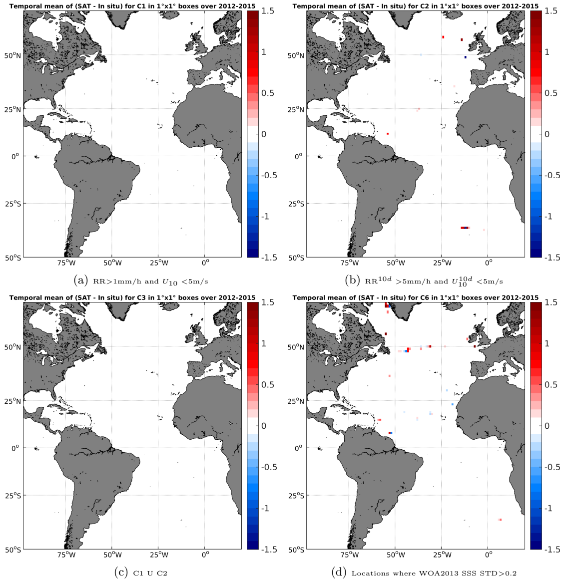
Figure 12: Temporal mean gridded over spatial boxes of size 1°x1° of \Delta SSS (AQUARIUS-L2-JPL-V4 - TSG-GOSUD-Sailing-ship) for 4 different subdatasets corresponding to:RR>1mm/h and U_{10} < 5m/s (a), RR^{10d} > 5mm/h and U_{10}^{10d} < 5m/s (b), C1 U C2 (c),Locations where WOA2013 SSS STD>0.2 (d).
