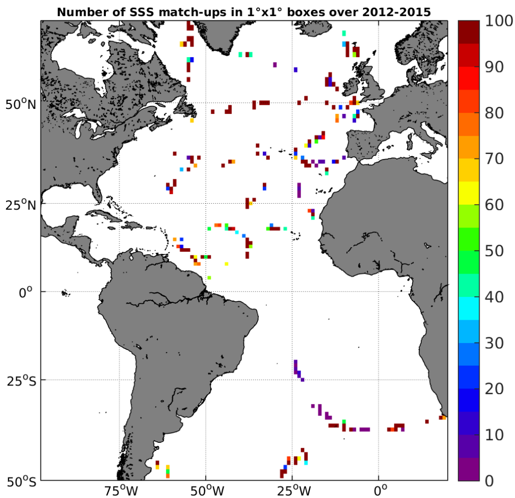
Figure 4: Number of SSS match-ups between TSG-GOSUD-Sailing-ship SSS and the AQUARIUS-L2-JPL-V4 SSS product for the Atlantic Ocean Pi-MEP region over 1°x1° boxes and for the full satellite product period.
