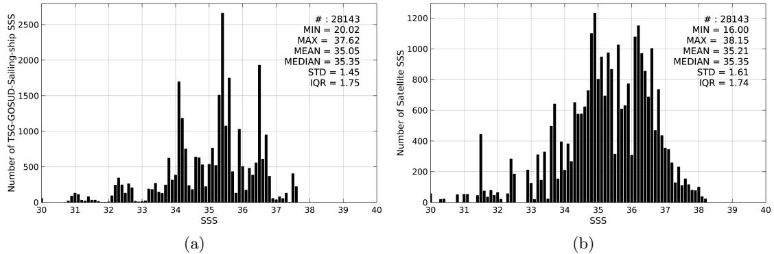
Figure 2: Histograms of SSS from TSG-GOSUD-Sailing-ship (a) and AQUARIUS-L2-JPL-V4 (b) considering all match-up pairs per bins of 0.1 over the Atlantic Ocean Pi-MEP region and for the full satellite product period.
