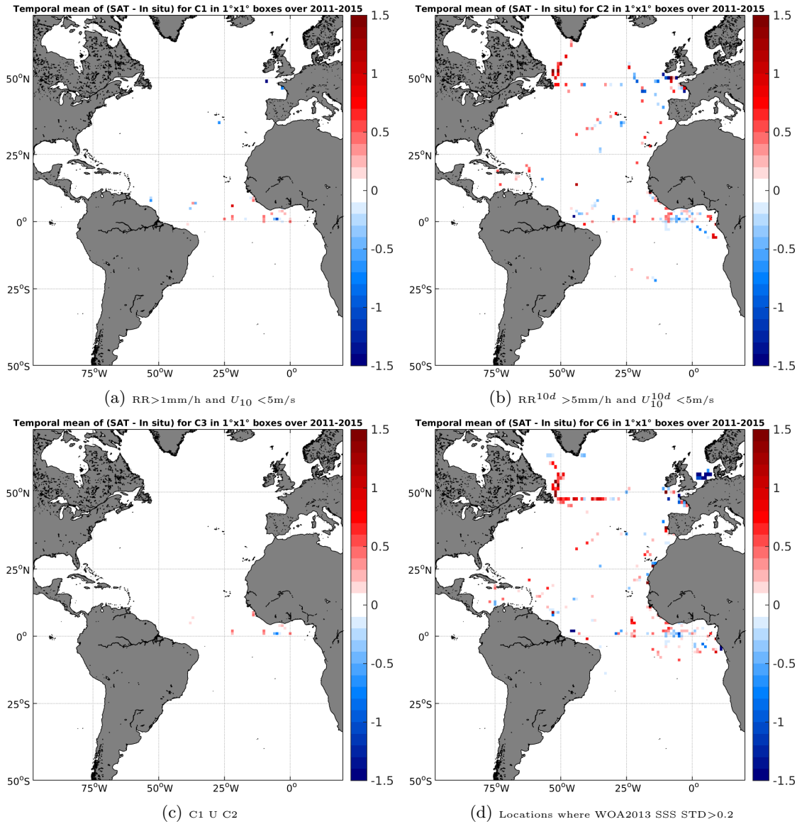
Figure 12: Temporal mean gridded over spatial boxes of size 1°x1° of \Delta\text{SSS} (AQUARIUS-L2-JPL-V4 - TSG-GOSUD-Research-vessel) for 4 different subdatasets corresponding to: RR > 1\text{mm/h} and U_{10} < 5\text{m/s} (a), RR^{10d} > 5\text{mm/h} and U_{10}^{10d} < 5\text{m/s} (b), C1 U C2 (c), Locations where WOA2013 SSS STD > 0.2 (d).
