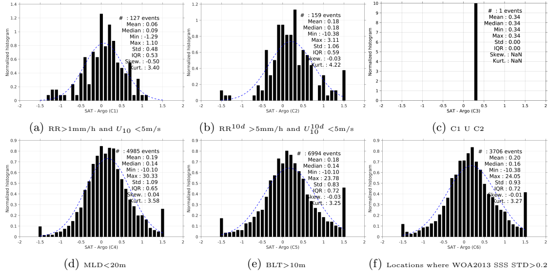
Figure 13: Normalized histogram of \Delta\text{SSS} (AQUARIUS-L2-JPL-V4 - Argo) for 6 different sub-datasets corresponding to: RR>1mm/h and U_{10} < 5\text{m/s} (a), RR^{10d} > 5\text{mm/h} and U_{10}^{10d} < 5\text{m/s} (b), C1 U C2 (c),MLD<20m (d),BLT>10m (e),Locations where WOA2013 SSS STD>0.2 (f).
