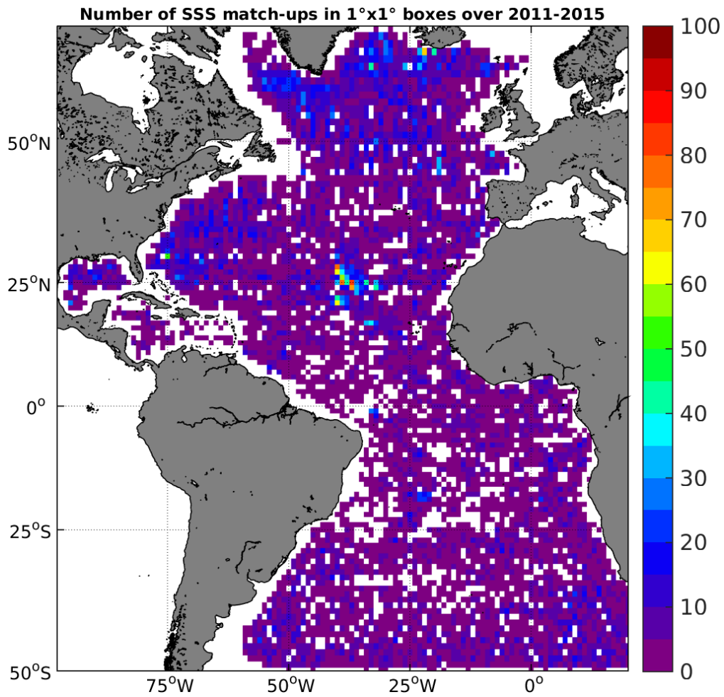
Figure 4: Number of SSS match-ups between Argo SSS and the AQUARIUS-L2-JPL-V4 SSS product for the Atlantic Ocean Pi-MEP region over 1°x1° boxes and for the full satellite product period.
