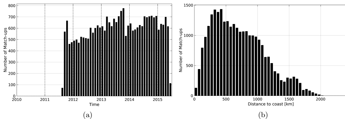
Figure 1: Number of match-ups between Argo and AQUARIUS-L2-JPL-V4 SSS as a function of time (a) and as function of the distance to coast (b) over the Atlantic Ocean Pi-MEP region and for the full satellite product period.
