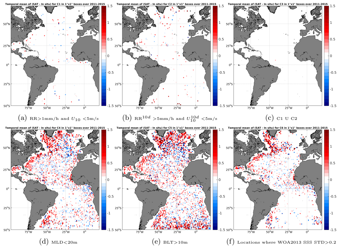
Figure 12: Temporal mean gridded over spatial boxes of size 1^\circ \times 1^\circ of \Delta SSS (AQUARIUS-L2-JPL-V4 - Argo) for 6 different subdatasets corresponding to: RR > 1\text{mm/h} and U_{10} < 5\text{m/s} (a), RR^{10d} > 5\text{mm/h} and U_{10}^{10d} < 5\text{m/s} (b), C1 U C2 (c), MLD < 20\text{m} (d), BLT > 10\text{m} (e), Locations where WOA2013 SSS STD > 0.2 (f).
