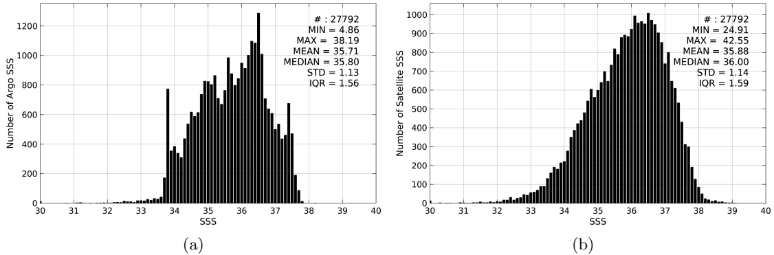
Figure 2: Histograms of SSS from Argo (a) and AQUARIUS-L2-JPL-V4 (b) considering all match-up pairs per bins of 0.1 over the Atlantic Ocean Pi-MEP region and for the full satellite product period.
