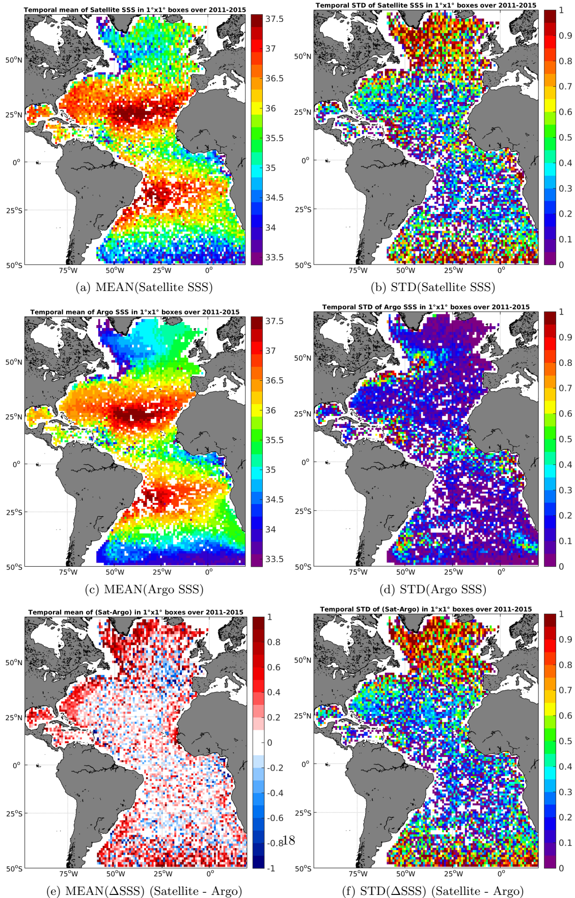
Figure 6: Temporal mean (left) and STD (right) of SSS from AQUARIUS-L2-JPL-V4 (top), Argo (middle), and of \Delta SSS (Satellite - Argo). Only match-up pairs are used to generate these maps.
