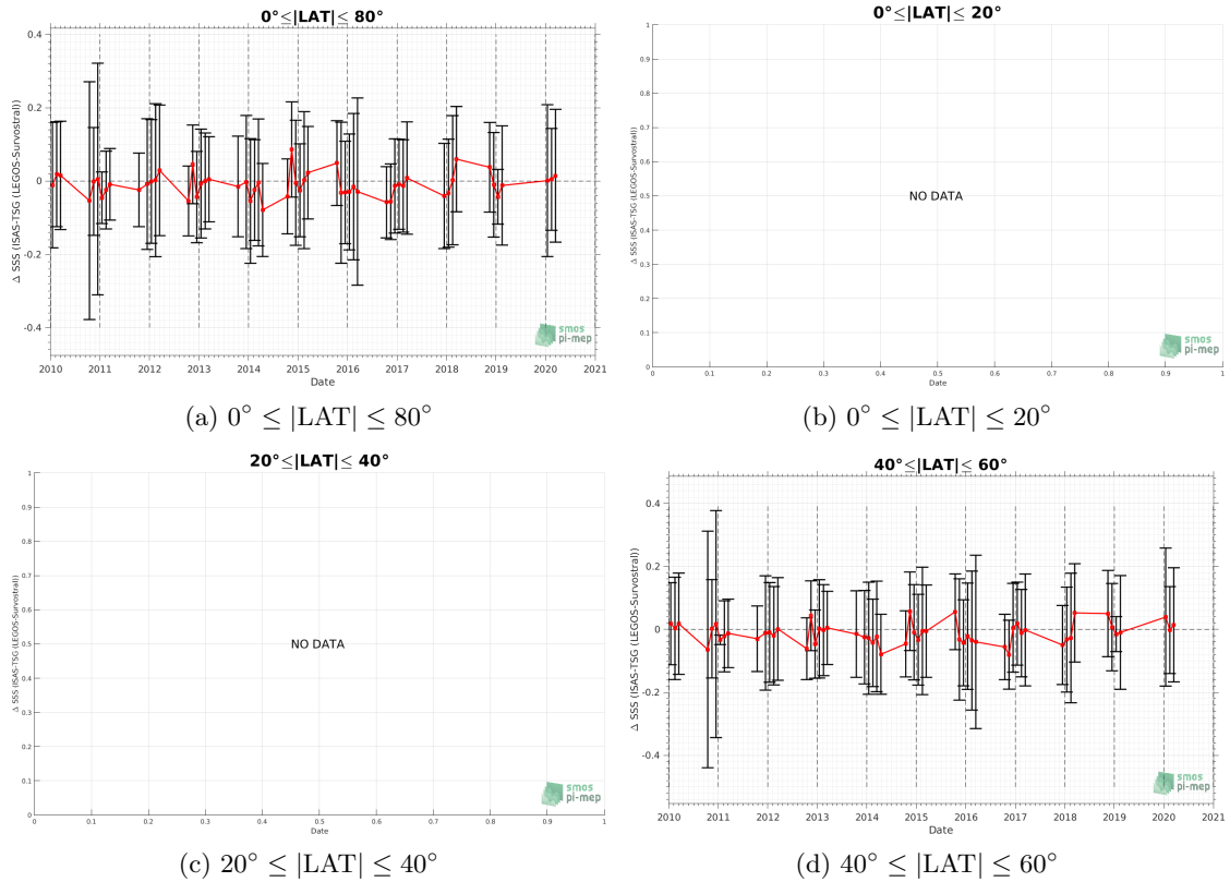
Figure 95: Monthly median (red curves) of \Delta SSS (ISAS - TSG (LEGOS-Survostral)) and \pm 1 Std (black vertical thick bars) as function of time for all the collected Pi-MEP match-up pairs for the full in situ dataset period are shown for different latitude bands: (a) 80^\circ\text{S}-80^\circ\text{N} , (b) 20^\circ\text{S}-20^\circ\text{N} , (c) 40^\circ\text{S}-20^\circ\text{S} and 20^\circ\text{N}-40^\circ\text{N} and (d) 60^\circ\text{S}-40^\circ\text{S} and 40^\circ\text{N}-60^\circ\text{N} .
