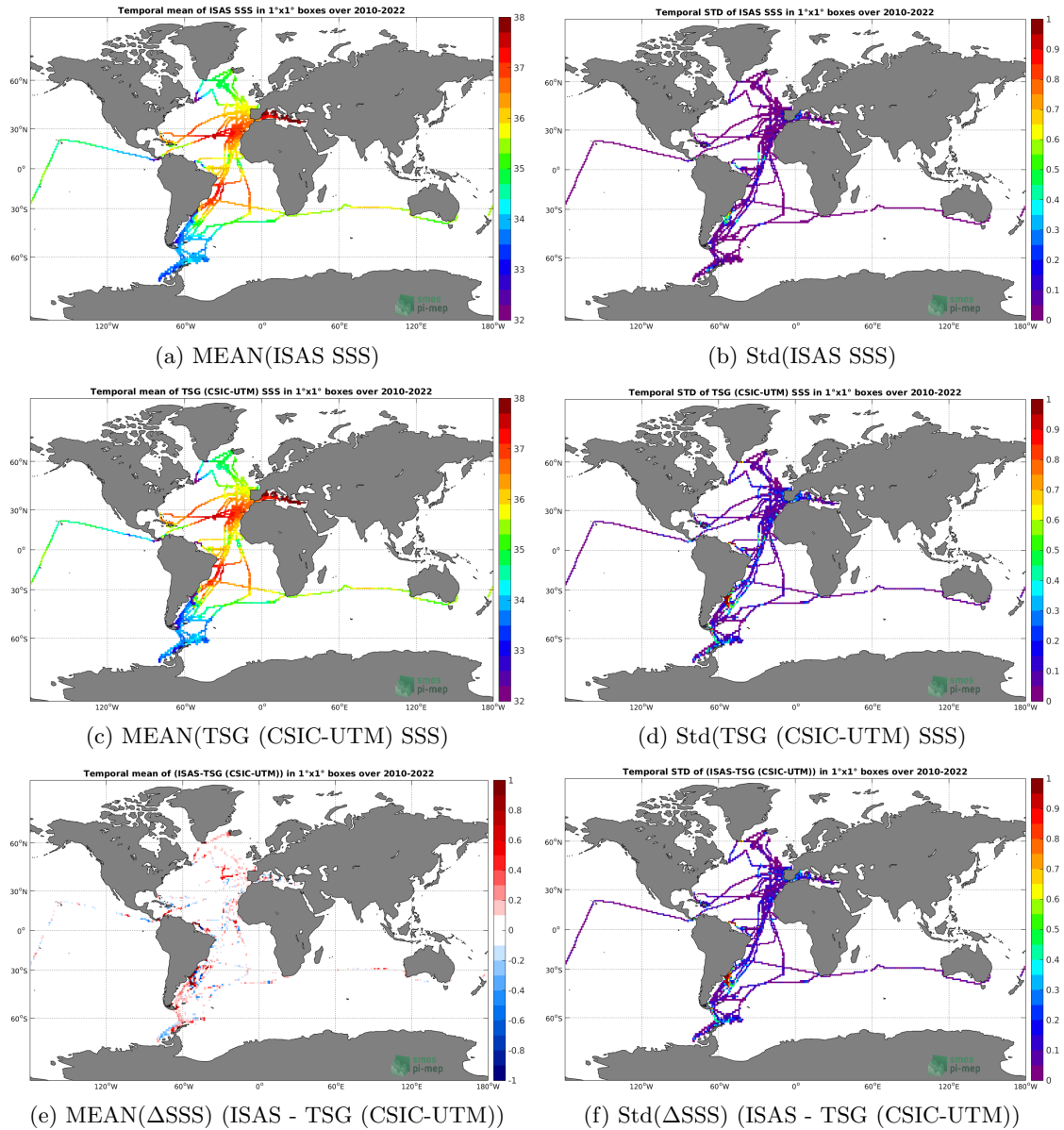
Figure 53: Temporal mean (left) and Std (right) of SSS from ISAS (top), TSG (CSIC-UTM) (middle), and of \Delta SSS (ISAS - TSG (CSIC-UTM)). Only match-up pairs are used to generate these maps.
