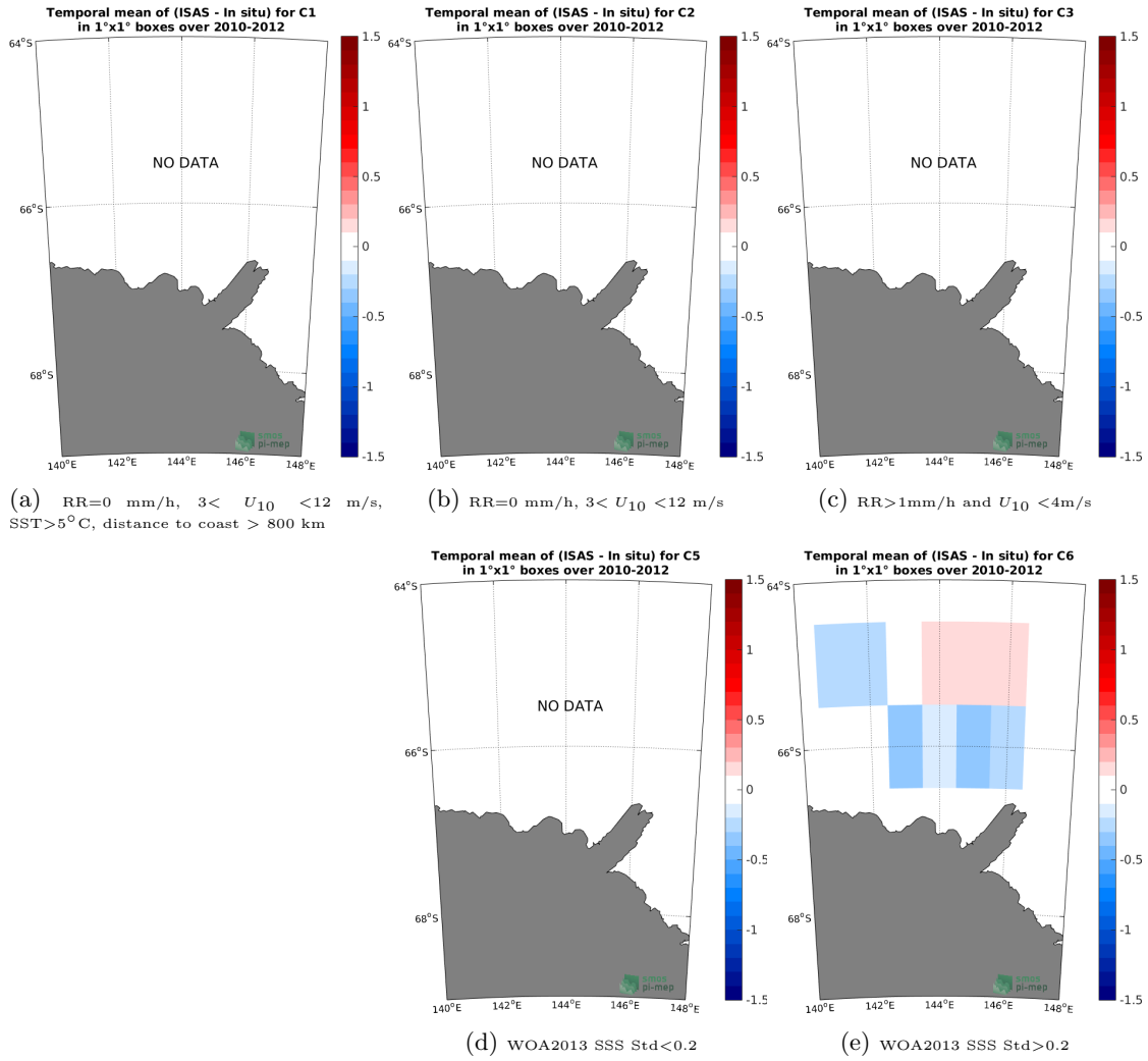
Figure 110: Temporal mean gridded over spatial boxes of size 1°x1° of \Delta SSS (ISAS - TSG (LEGOS-Survostral-Adelie)) for 5 different subdatasets corresponding to:RR=0 mm/h, 3 < U_{10} < 12 m/s, SST>5°C, distance to coast > 800 km (a), RR=0 mm/h, 3 < U_{10} < 12 m/s (b), RR>1mm/h and U_{10} < 4 m/s (c),WOA2013 SSS Std<0.2 (d),WOA2013 SSS Std>0.2 (e).
