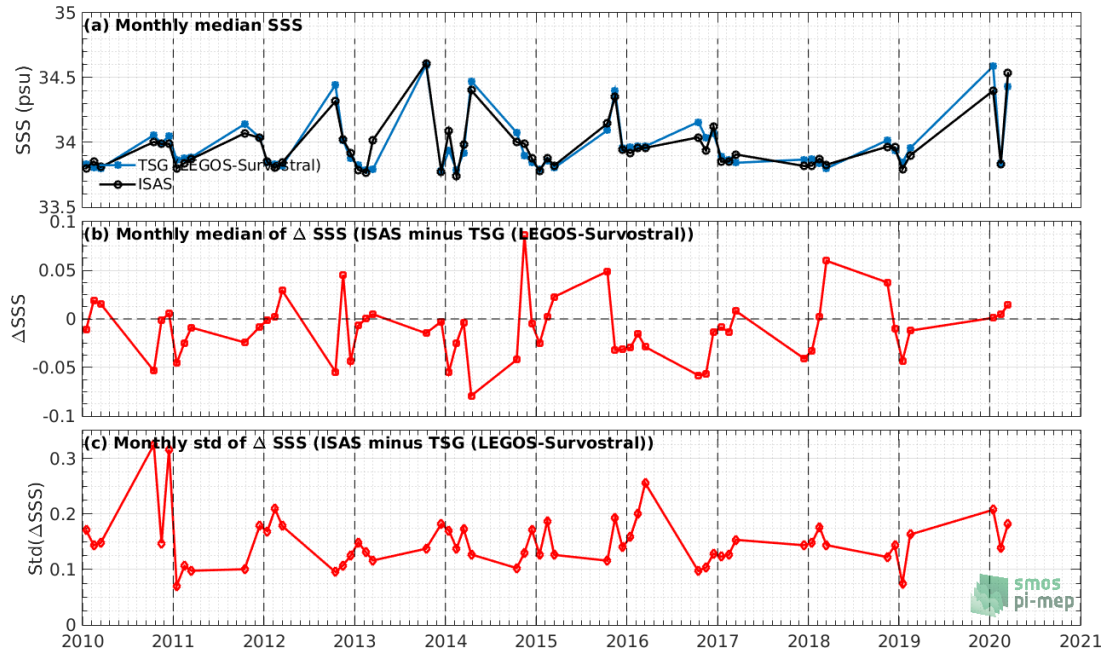
Figure 92: Time series of the monthly median SSS (top), median of \Delta SSS (ISAS - TSG (LEGOS-Survostral)) and Std of \Delta SSS (ISAS - TSG (LEGOS-Survostral)) considering all match-ups collected by the Pi-MEP.
