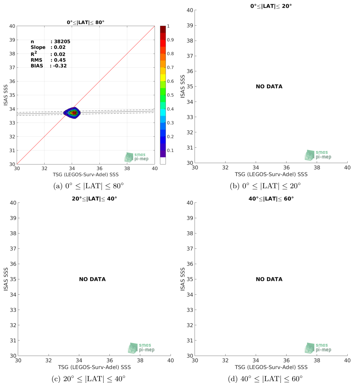
Figure 107: Contour maps of the concentration of ISAS SSS (y-axis) versus TSG (LEGOS-Survostral-Adelie) SSS (x-axis) at match-up pairs for different latitude bands. For each plot, the red line shows x=y . The black thin and dashed lines indicate a linear fit through the data cloud and the \pm 95\% confidence levels, respectively. The number match-up pairs n , the slope and R^2 coefficient of the linear fit, the root mean square (RMS) and the mean bias between ISAS and in situ data are indicated for each latitude band in each plots.
