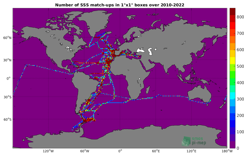
Figure 52: Number of SSS from TSG (CSIC-UTM) in 1^\circ \times 1^\circ boxes.
