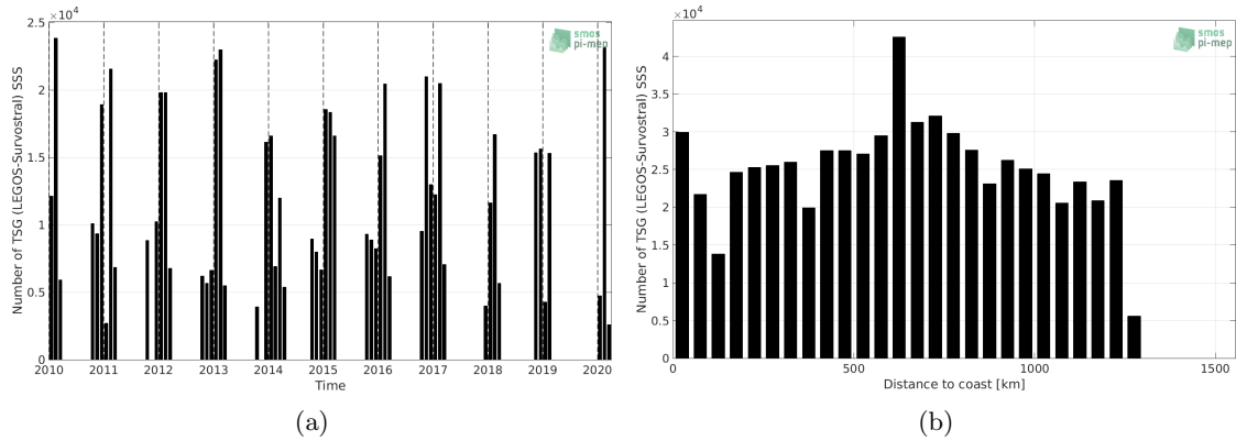
Figure 87: Number of SSS from TSG (LEGOS-Survostral) as a function of time (a) and distance to coast (b).
