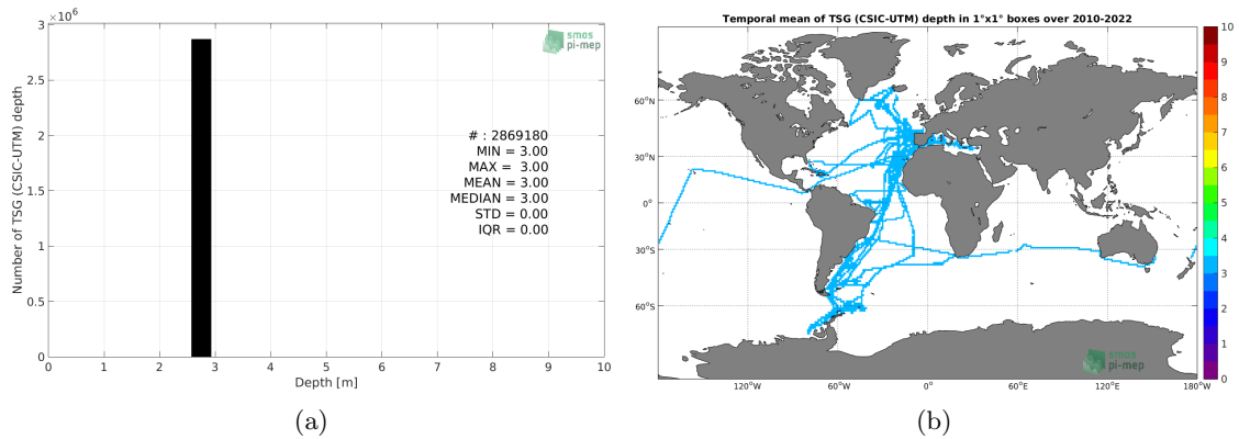
Figure 51: Depth distribution of the upper level SSS measurements from TSG (CSIC-UTM) (a) and spatial distribution of the in situ SSS depth measurements showing the mean value in 1^\circ \times 1^\circ boxes and considering the full in situ dataset period (b).
