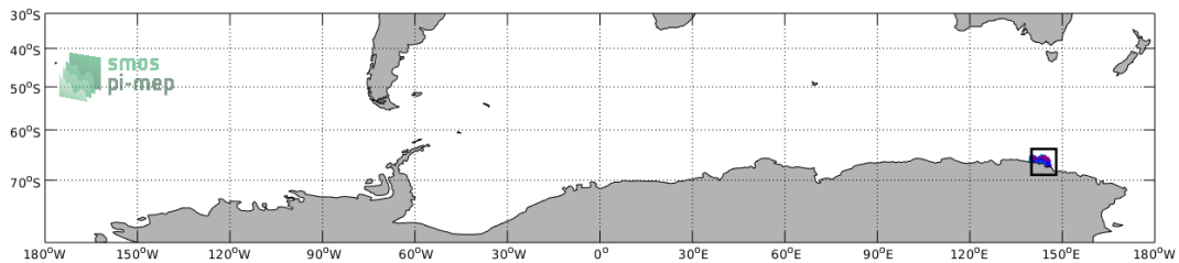
Figure 99: Location of the TSG (LEGOS-Survostral-Adelie) dataset.
