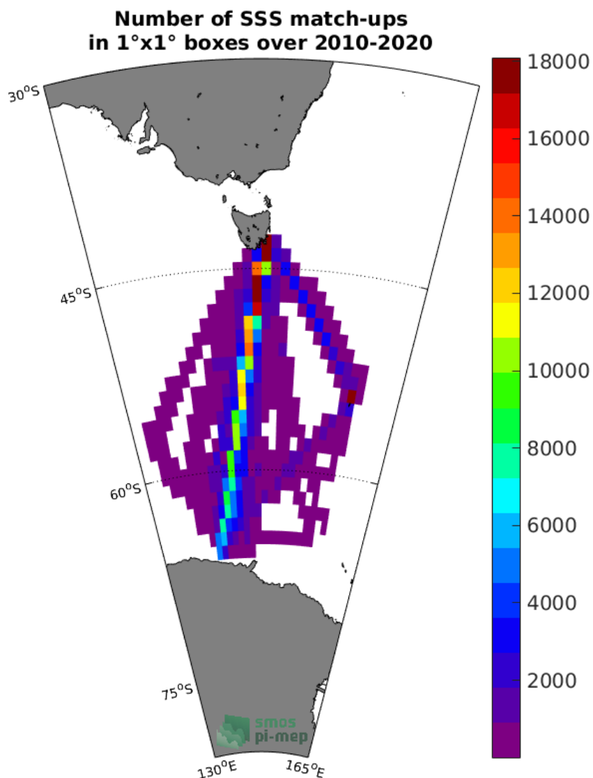
Figure 90: Number of SSS from TSG (LEGOS-Survostral) in 1°x1° boxes.
