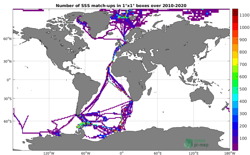
Figure 64: Number of SSS from TSG (Polarstern) in 1°x1° boxes.
