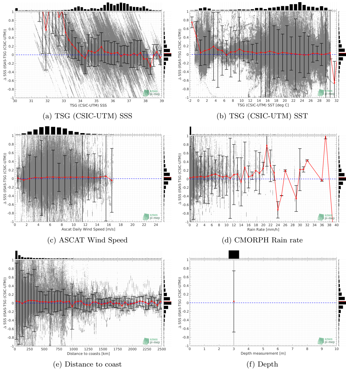
Figure 58: \Delta SSS (ISAS - TSG (CSIC-UTM)) sorted as geophysical conditions: TSG (CSIC-UTM) SSS a), TSG (CSIC-UTM) SST b), ASCAT Wind speed c), CMORPH rain rate d), distance to coast (e) and depth measurements (f).
