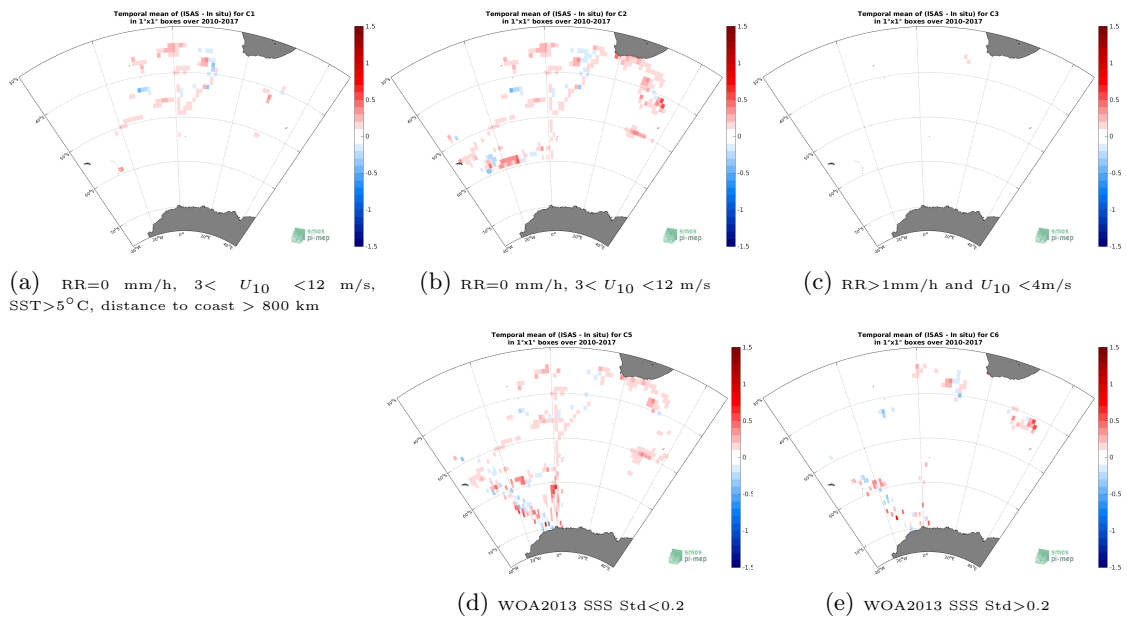
Figure 84: Temporal mean gridded over spatial boxes of size 1^\circ \times 1^\circ of \Delta SSS (ISAS - TSG (NCEI-0170743)) for 5 different subdatasets corresponding to:RR=0 mm/h, 3 < U_{10} < 12 m/s, SST > 5^\circ\text{C} , distance to coast > 800 km (a), RR=0 mm/h, 3 < U_{10} < 12 m/s (b), RR > 1 mm/h and U_{10} < 4 m/s (c), WOA2013 SSS Std < 0.2 (d), WOA2013 SSS Std > 0.2 (e).
