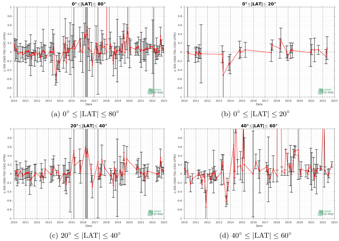
Figure 57: Monthly median (red curves) of \Delta\text{SSS} (ISAS - TSG (CSIC-UTM)) and \pm 1 Std (black vertical thick bars) as function of time for all the collected Pi-MEP match-up pairs for the full in situ dataset period are shown for different latitude bands: (a) 80^\circ\text{S}-80^\circ\text{N} , (b) 20^\circ\text{S}-20^\circ\text{N} , (c) 40^\circ\text{S}-20^\circ\text{S} and 20^\circ\text{N}-40^\circ\text{N} and (d) 60^\circ\text{S}-40^\circ\text{S} and 40^\circ\text{N}-60^\circ\text{N} .
