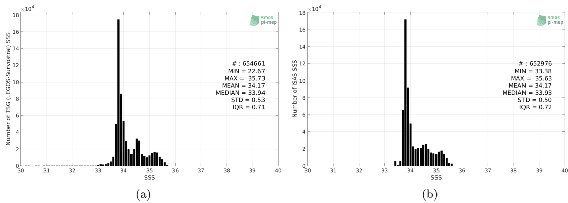
Figure 88: Histograms of SSS from TSG (LEGOS-Survostral) (a) and ISAS (b) per bins of 0.1.
