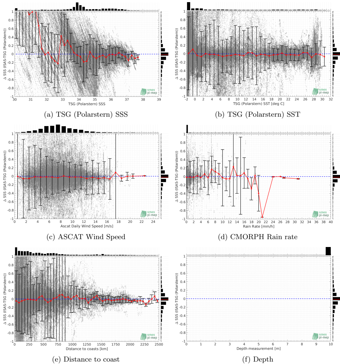
Figure 70: \Delta SSS (ISAS - TSG (Polarstern)) sorted as geophysical conditions: TSG (Polarstern) SSS a), TSG (Polarstern) SST b), ASCAT Wind speed c), CMORPH rain rate d), distance to coast (e) and depth measurements (f).
