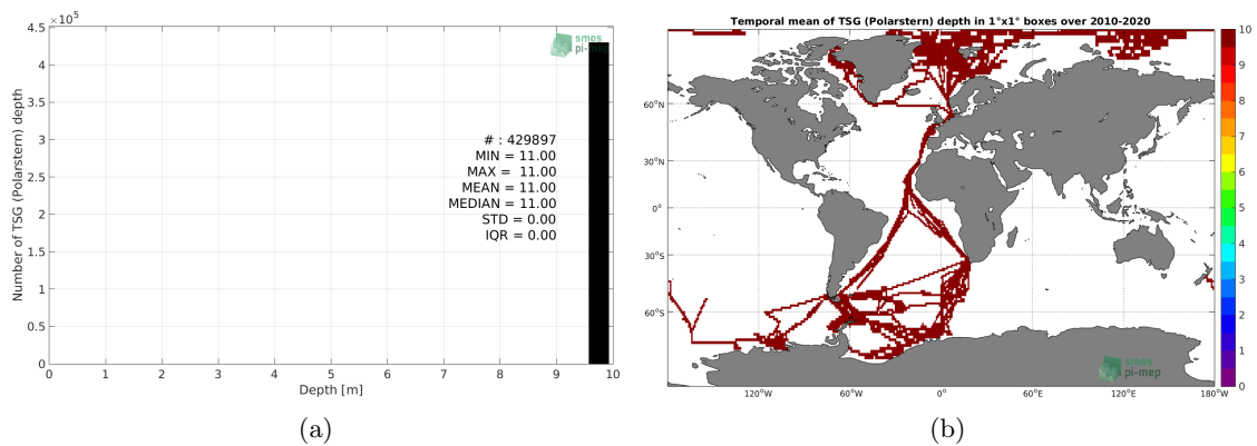
Figure 63: Depth distribution of the upper level SSS measurements from TSG (Polarstern) (a) and spatial distribution of the in situ SSS depth measurements showing the mean value in 1°x1° boxes and considering the full in situ dataset period (b).
