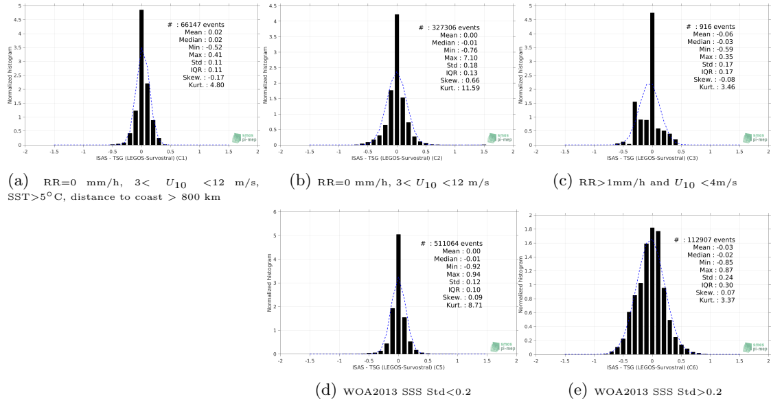
Figure 98: Normalized histogram of \Delta SSS (ISAS - TSG (LEGOS-Survostral)) for 5 different subdatasets corresponding to: RR=0 mm/h, 3 < U_{10} < 12 m/s, SST > 5°C, distance to coast > 800 km (a), RR=0 mm/h, 3 < U_{10} < 12 m/s (b), RR > 1mm/h and U_{10} < 4 m/s (c), WOA2013 SSS Std < 0.2 (d), WOA2013 SSS Std > 0.2 (e).
