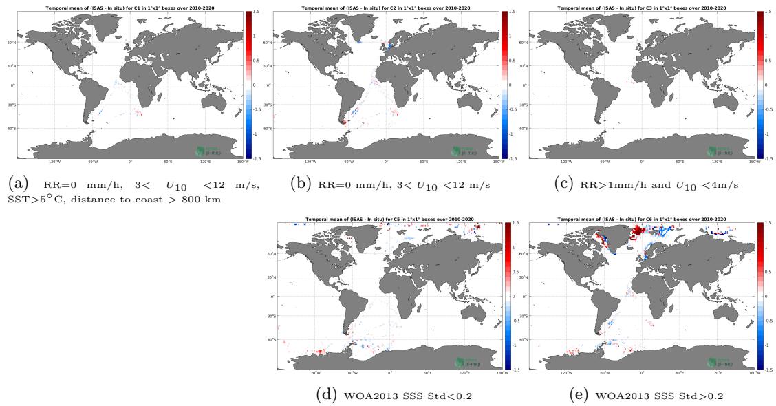
Figure 71: Temporal mean gridded over spatial boxes of size 1^\circ \times 1^\circ of \Delta SSS (ISAS - TSG (Polarstern)) for 5 different subdatasets corresponding to:RR=0 mm/h, 3 < U_{10} < 12 m/s, SST > 5^\circ C, distance to coast > 800 km (a), RR=0 mm/h, 3 < U_{10} < 12 m/s (b), RR > 1 mm/h and U_{10} < 4 m/s (c),WOA2013 SSS Std < 0.2 (d),WOA2013 SSS Std > 0.2 (e).
