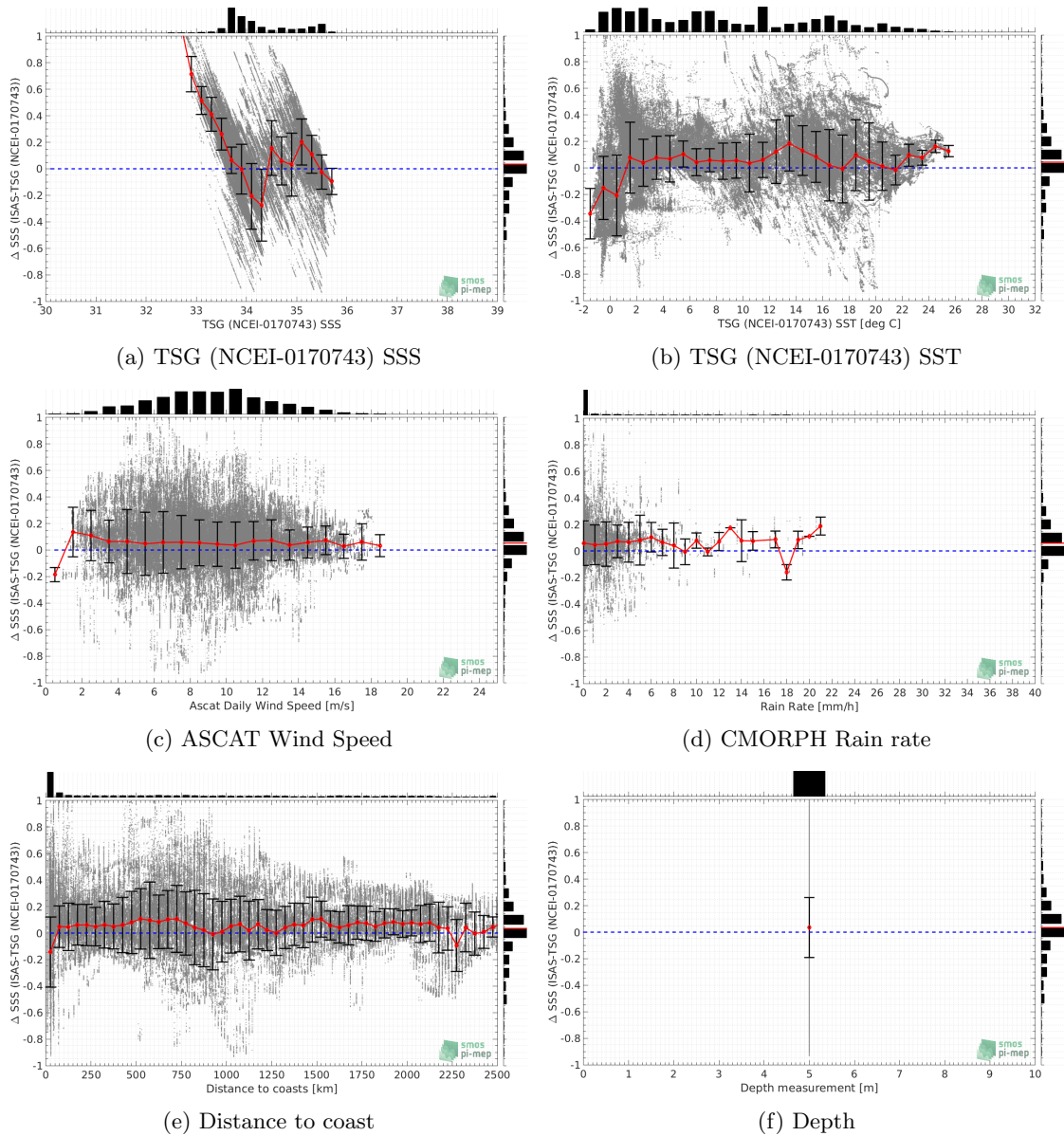
Figure 83: \Delta SSS (ISAS - TSG (NCEI-0170743)) sorted as geophysical conditions: TSG (NCEI-0170743) SSS a), TSG (NCEI-0170743) SST b), ASCAT Wind speed c), CMORPH rain rate d), distance to coast (e) and depth measurements (f).
