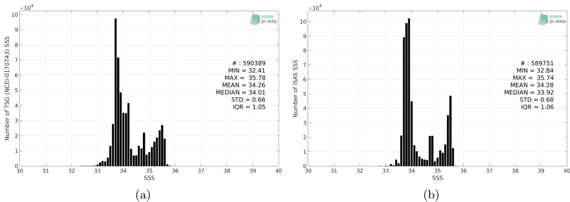
Figure 75: Histograms of SSS from TSG (NCEI-0170743) (a) and ISAS (b) per bins of 0.1.
