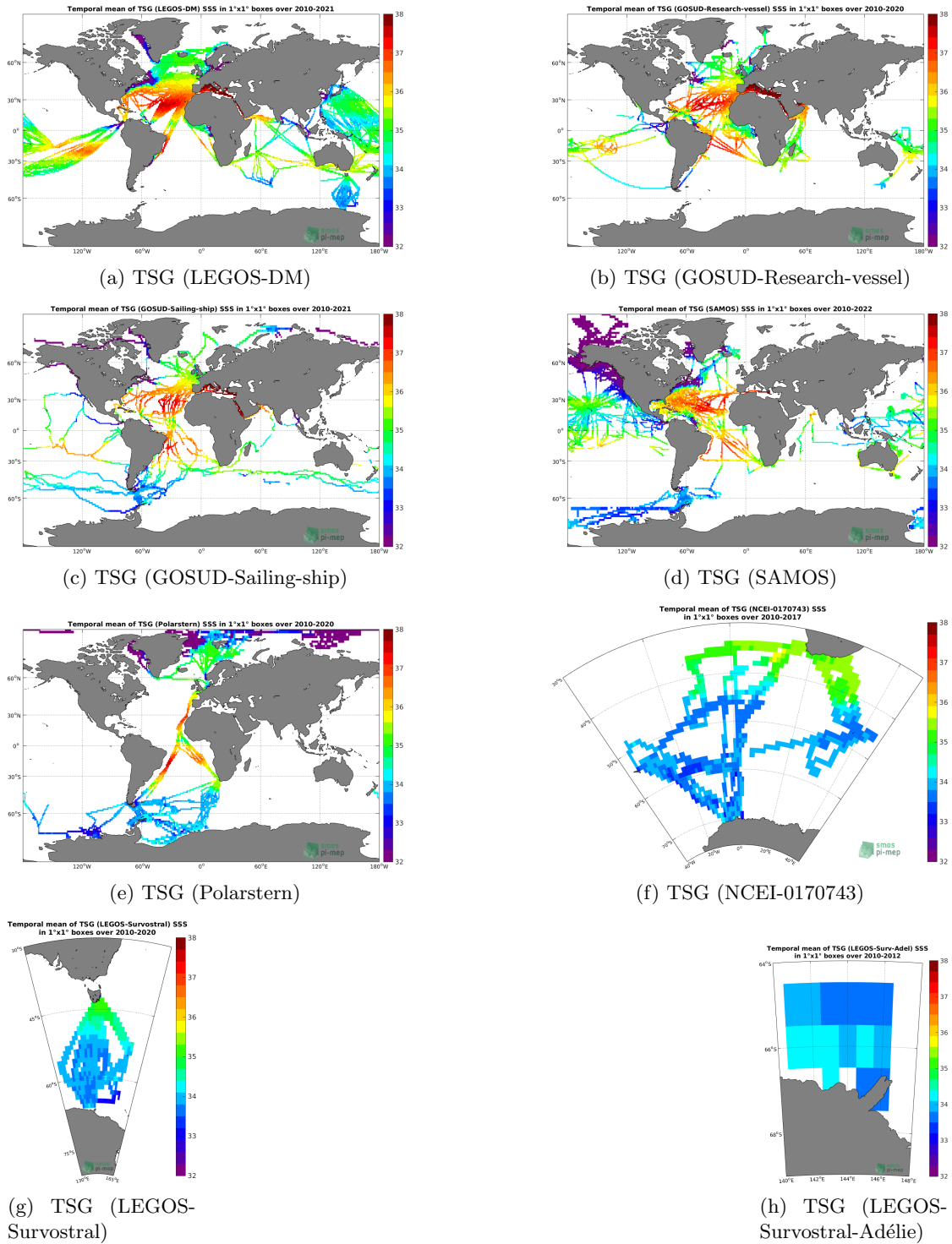
Figure 114: Temporal mean of SSS in 1^\circ \times 1^\circ boxes.
