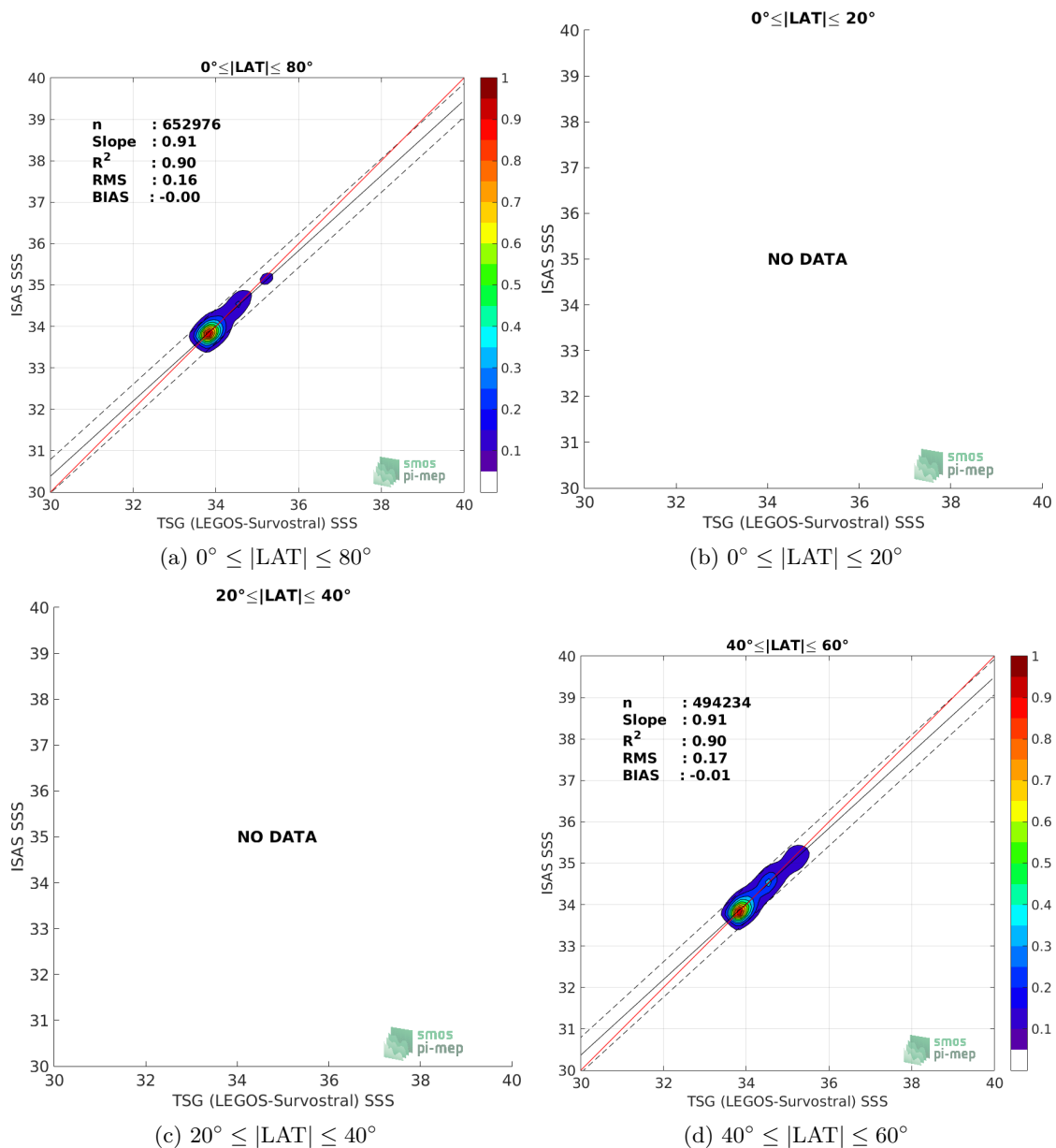
Figure 94: Contour maps of the concentration of ISAS SSS (y-axis) versus TSG (LEGOS-Survostral) SSS (x-axis) at match-up pairs for different latitude bands. For each plot, the red line shows x=y . The black thin and dashed lines indicate a linear fit through the data cloud and the \pm 95\% confidence levels, respectively. The number match-up pairs n , the slope and R^2 coefficient of the linear fit, the root mean square (RMS) and the mean bias between ISAS and in situ data are indicated for each latitude band in each plots.
