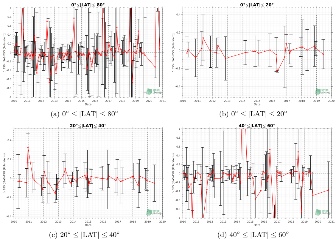
Figure 69: Monthly median (red curves) of \Delta\text{SSS} (ISAS - TSG (Polarstern)) and \pm 1 Std (black vertical thick bars) as function of time for all the collected Pi-MEP match-up pairs for the full in situ dataset period are shown for different latitude bands: (a) 80^\circ\text{S}-80^\circ\text{N} , (b) 20^\circ\text{S}-20^\circ\text{N} , (c) 40^\circ\text{S}-20^\circ\text{S} and 20^\circ\text{N}-40^\circ\text{N} and (d) 60^\circ\text{S}-40^\circ\text{S} and 40^\circ\text{N}-60^\circ\text{N} .
