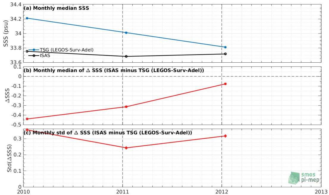
Figure 105: Time series of the monthly median SSS (top), median of \Delta SSS (ISAS - TSG (LEGOS-Survostral-Adelie)) and Std of \Delta SSS (ISAS - TSG (LEGOS-Survostral-Adelie)) considering all match-ups collected by the Pi-MEP.
