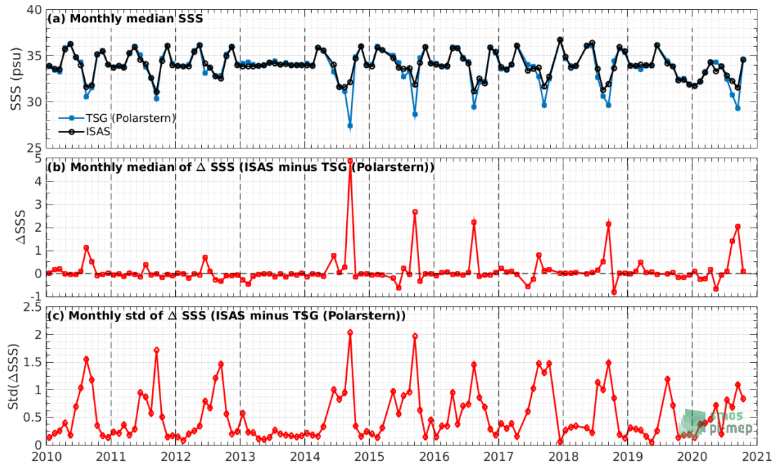
Figure 66: Time series of the monthly median SSS (top), median of \Delta SSS (ISAS - TSG (Polarstern)) and Std of \Delta SSS (ISAS - TSG (Polarstern)) considering all match-ups collected by the Pi-MEP.
