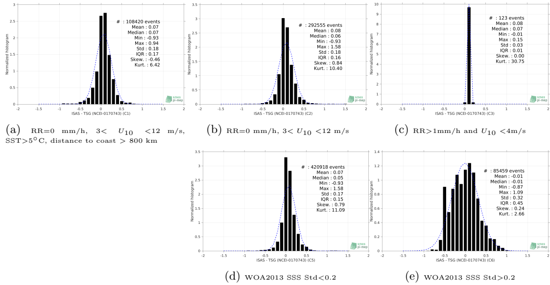
Figure 85: Normalized histogram of \Delta SSS (ISAS - TSG (NCEI-0170743)) for 5 different sub-datasets corresponding to: RR=0 mm/h, 3 < U_{10} < 12 m/s, SST > 5°C, distance to coast > 800 km (a), RR=0 mm/h, 3 < U_{10} < 12 m/s (b), RR > 1mm/h and U_{10} < 4 m/s (c), WOA2013 SSS Std < 0.2 (d), WOA2013 SSS Std > 0.2 (e).
