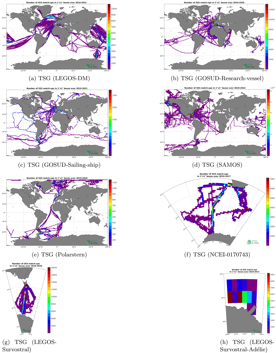
Figure 116: Number of SSS in 1°x1° boxes.
