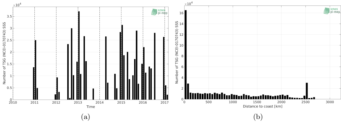
Figure 74: Number of SSS from TSG (NCEI-0170743) as a function of time (a) and distance to coast (b).
