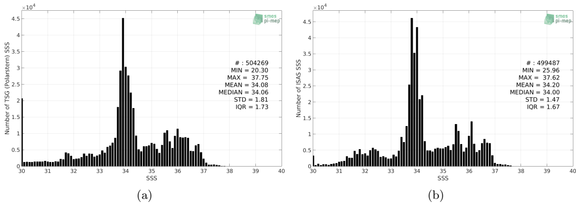
Figure 62: Histograms of SSS from TSG (Polarstern) (a) and ISAS (b) per bins of 0.1.
