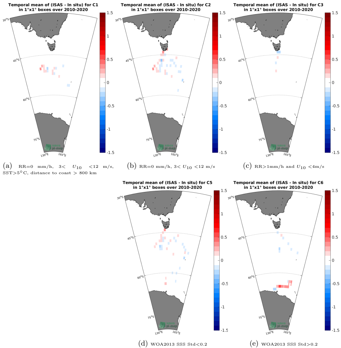
Figure 97: Temporal mean gridded over spatial boxes of size 1°x1° of \Delta SSS (ISAS - TSG (LEGOS-Survostral)) for 5 different subdatasets corresponding to:RR=0 mm/h, 3 < U_{10} < 12 m/s, SST>5°C, distance to coast > 800 km (a), RR=0 mm/h, 3 < U_{10} < 12 m/s (b), RR>1mm/h and U_{10} < 4 m/s (c),WOA2013 SSS Std<0.2 (d),WOA2013 SSS Std>0.2 (e).
