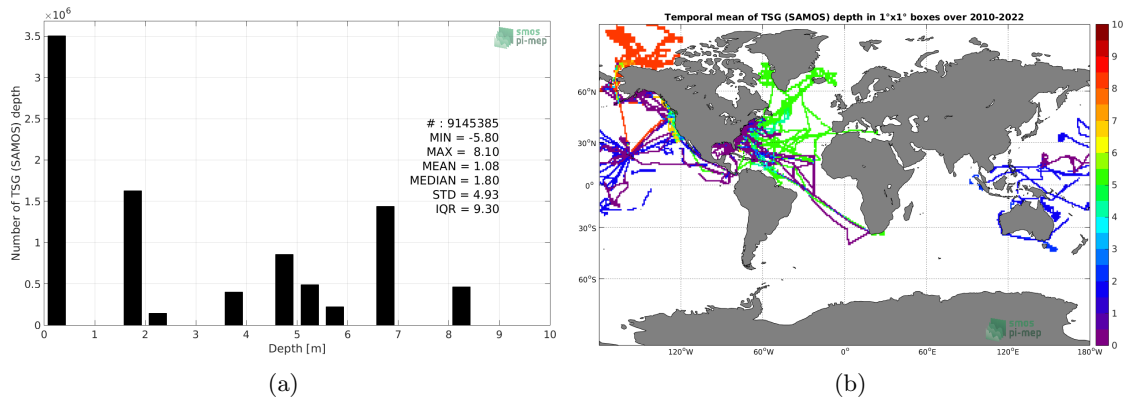
Figure 39: Depth distribution of the upper level SSS measurements from TSG (SAMOS) (a) and spatial distribution of the in situ SSS depth measurements showing the mean value in 1^\circ \times 1^\circ boxes and considering the full in situ dataset period (b).
