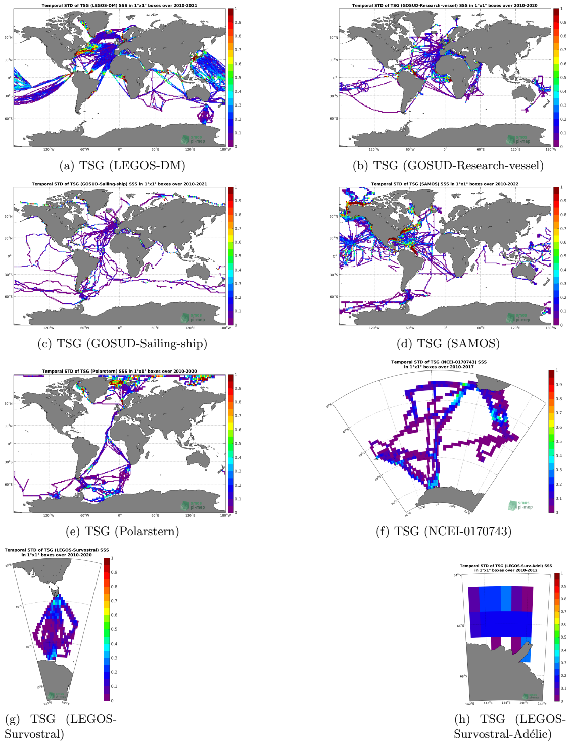
Figure 115: Temporal Std of SSS in 1°x1° boxes.
