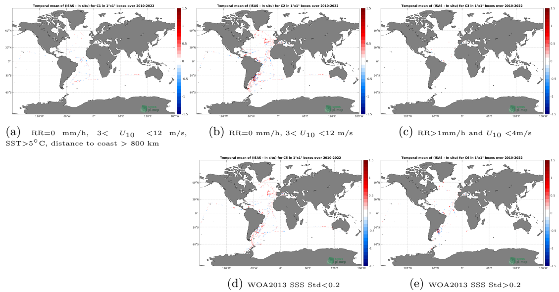
Figure 59: Temporal mean gridded over spatial boxes of size 1^\circ \times 1^\circ of \Delta SSS (ISAS - TSG (CSIC-UTM)) for 5 different subdatasets corresponding to: RR=0 mm/h, 3 < U_{10} < 12 m/s, SST > 5°C, distance to coast > 800 km (a), RR=0 mm/h, 3 < U_{10} < 12 m/s (b), RR > 1mm/h and U_{10} < 4 m/s (c), WOA2013 SSS Std < 0.2 (d), WOA2013 SSS Std > 0.2 (e).
