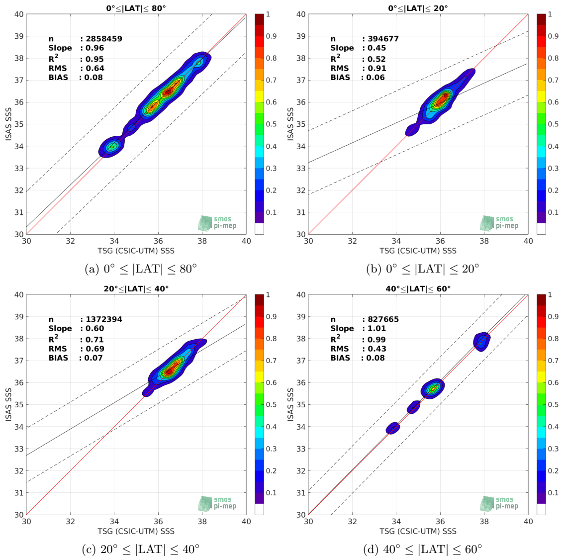
Figure 56: Contour maps of the concentration of ISAS SSS (y-axis) versus TSG (CSIC-UTM) SSS (x-axis) at match-up pairs for different latitude bands. For each plot, the red line shows x=y . The black thin and dashed lines indicate a linear fit through the data cloud and the \pm 95\% confidence levels, respectively. The number match-up pairs n , the slope and R^2 coefficient of the linear fit, the root mean square (RMS) and the mean bias between ISAS and in situ data are indicated for each latitude band in each plots.
