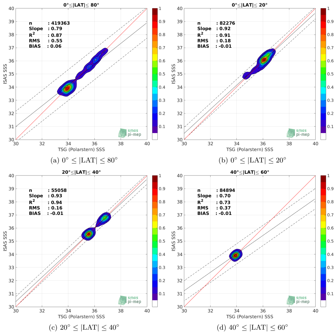
Figure 68: Contour maps of the concentration of ISAS SSS (y-axis) versus TSG (Polarstern) SSS (x-axis) at match-up pairs for different latitude bands. For each plot, the red line shows x=y . The black thin and dashed lines indicate a linear fit through the data cloud and the \pm 95\% confidence levels, respectively. The number match-up pairs n , the slope and R^2 coefficient of the linear fit, the root mean square (RMS) and the mean bias between ISAS and in situ data are indicated for each latitude band in each plots.
