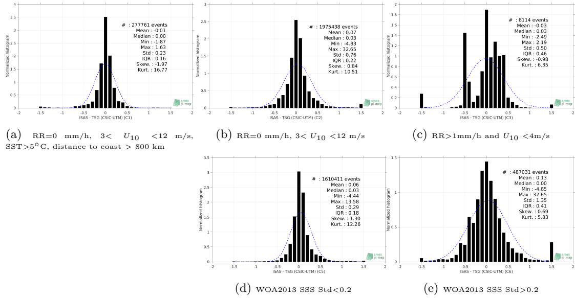
Figure 60: Normalized histogram of \Delta SSS (ISAS - TSG (CSIC-UTM)) for 5 different subdatasets corresponding to: RR=0 mm/h, 3 < U_{10} < 12 m/s, SST > 5°C, distance to coast > 800 km (a), RR=0 mm/h, 3 < U_{10} < 12 m/s (b), RR > 1mm/h and U_{10} < 4 m/s (c), WOA2013 SSS Std < 0.2 (d), WOA2013 SSS Std > 0.2 (e).
