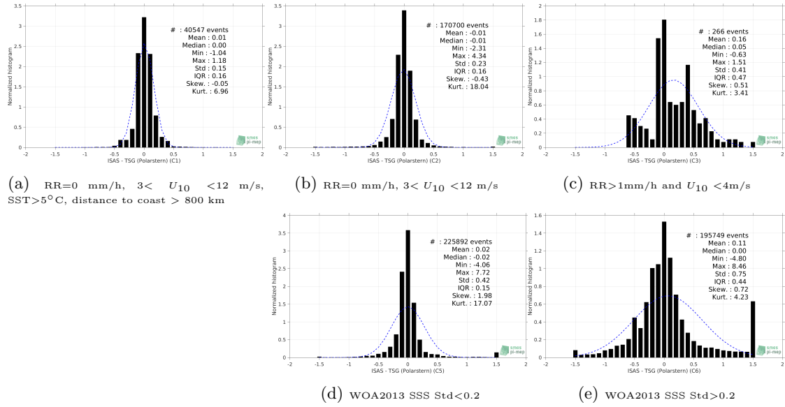
Figure 72: Normalized histogram of \Delta SSS (ISAS - TSG (Polarstern)) for 5 different subdatasets corresponding to: RR=0 mm/h, 3 < U_{10} < 12 m/s, SST > 5°C, distance to coast > 800 km (a), RR=0 mm/h, 3 < U_{10} < 12 m/s (b), RR > 1mm/h and U_{10} < 4 m/s (c), WOA2013 SSS Std < 0.2 (d), WOA2013 SSS Std > 0.2 (e).
