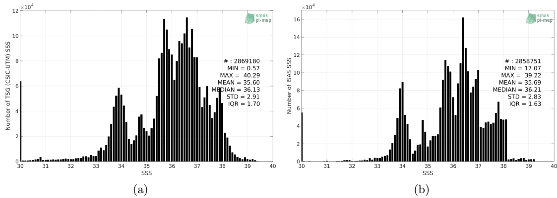
Figure 50: Histograms of SSS from TSG (CSIC-UTM) (a) and ISAS (b) per bins of 0.1.
