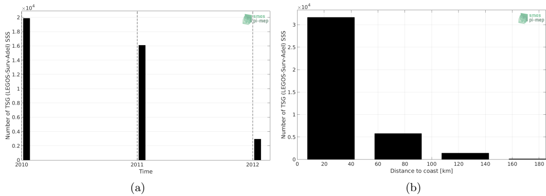
Figure 100: Number of SSS from TSG (LEGOS-Survostral-Adelie) as a function of time (a) and distance to coast (b).
