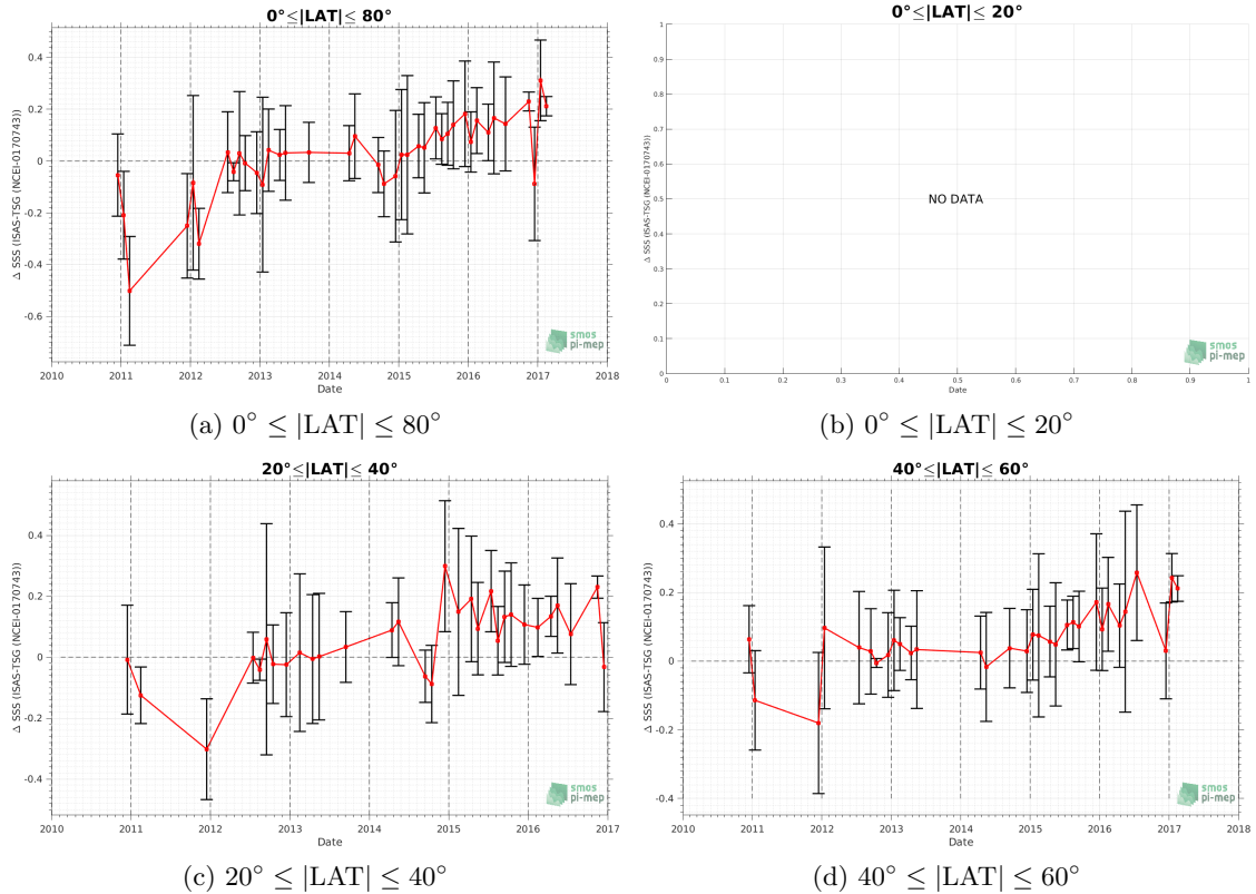
Figure 82: Monthly median (red curves) of \Delta\text{SSS} (ISAS - TSG (NCEI-0170743)) and \pm 1 Std (black vertical thick bars) as function of time for all the collected Pi-MEP match-up pairs for the full in situ dataset period are shown for different latitude bands: (a) 80°S-80°N, (b) 20°S-20°N, (c) 40°S-20°S and 20°N-40°N and (d) 60°S-40°S and 40°N-60°N.
