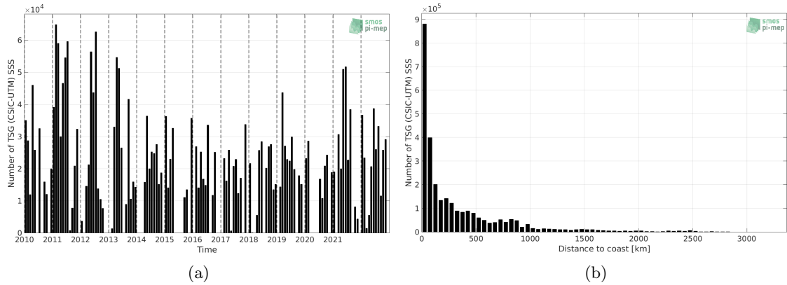
Figure 49: Number of SSS from TSG (CSIC-UTM) as a function of time (a) and distance to coast (b).
