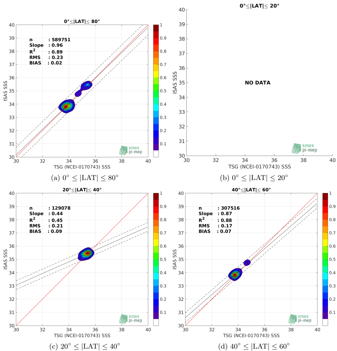
Figure 81: Contour maps of the concentration of ISAS SSS (y-axis) versus TSG (NCEI-0170743) SSS (x-axis) at match-up pairs for different latitude bands. For each plot, the red line shows x=y . The black thin and dashed lines indicate a linear fit through the data cloud and the \pm 95\% confidence levels, respectively. The number match-up pairs n , the slope and R^2 coefficient of the linear fit, the root mean square (RMS) and the mean bias between ISAS and in situ data are indicated for each latitude band in each plots.
