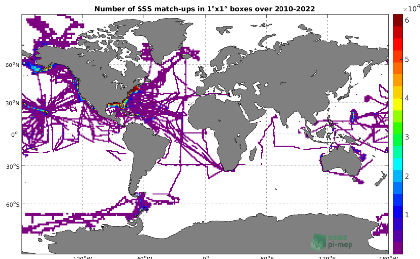
Figure 40: Number of SSS from TSG (SAMOS) in 1^\circ \times 1^\circ boxes.
