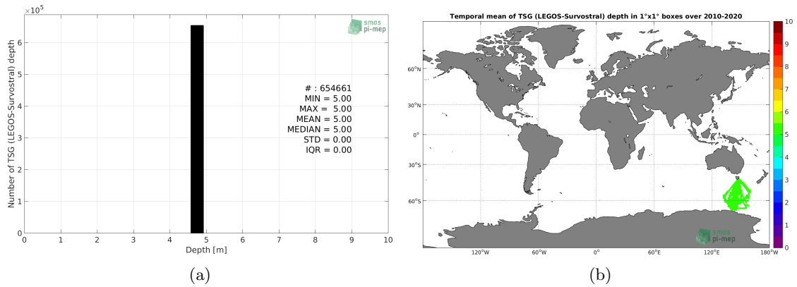
Figure 89: Depth distribution of the upper level SSS measurements from TSG (LEGOS-Survostral) (a) and spatial distribution of the in situ SSS depth measurements showing the mean value in 1^\circ \times 1^\circ boxes and considering the full in situ dataset period (b).
