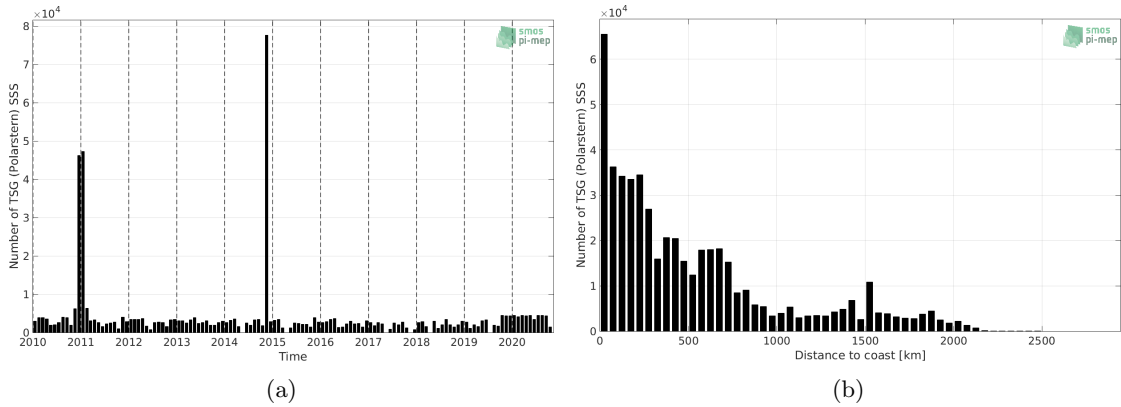
Figure 61: Number of SSS from TSG (Polarstern) as a function of time (a) and distance to coast (b).
