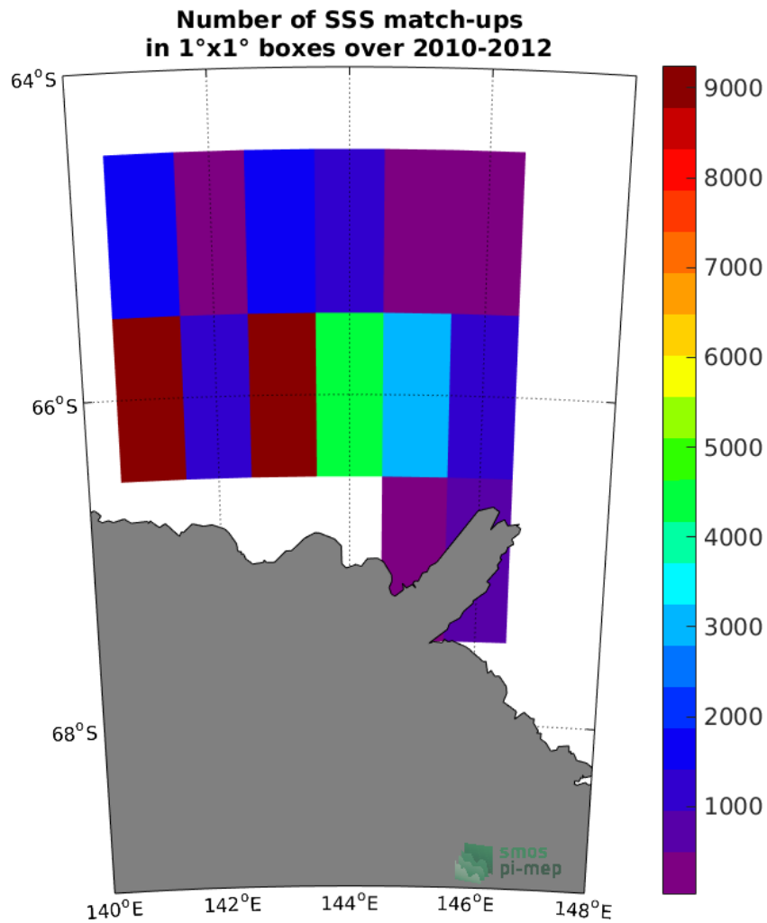
Figure 103: Number of SSS from TSG (LEGOS-Survostral-Adelie) in 1°x1° boxes.
