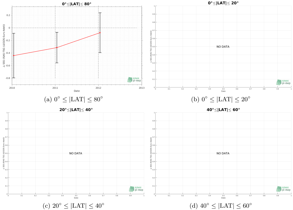
Figure 108: Monthly median (red curves) of \Delta SSS (ISAS - TSG (LEGOS-Survostral-Adelie)) and \pm 1 Std (black vertical thick bars) as function of time for all the collected Pi-MEP match-up pairs for the full in situ dataset period are shown for different latitude bands: (a) 80^{\circ}\text{S}-80^{\circ}\text{N} , (b) 20^{\circ}\text{S}-20^{\circ}\text{N} , (c) 40^{\circ}\text{S}-20^{\circ}\text{S} and 20^{\circ}\text{N}-40^{\circ}\text{N} and (d) 60^{\circ}\text{S}-40^{\circ}\text{S} and 40^{\circ}\text{N}-60^{\circ}\text{N} .
