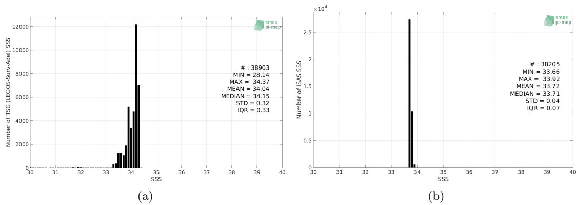
Figure 101: Histograms of SSS from TSG (LEGOS-Survostral-Adelie) (a) and ISAS (b) per bins of 0.1.
