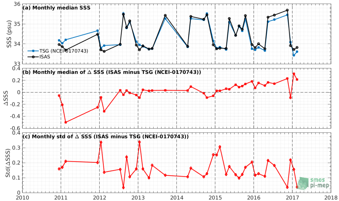
Figure 79: Time series of the monthly median SSS (top), median of \Delta SSS (ISAS - TSG (NCEI-0170743)) and Std of \Delta SSS (ISAS - TSG (NCEI-0170743)) considering all match-ups collected by the Pi-MEP.
