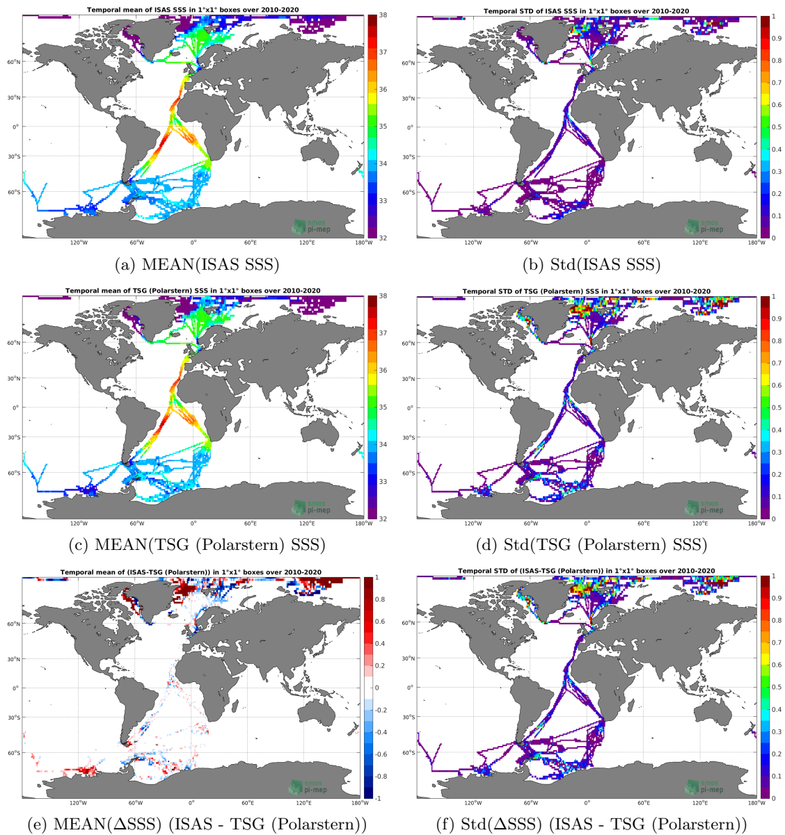
Figure 65: Temporal mean (left) and Std (right) of SSS from ISAS (top), TSG (Polarstern) (middle), and of \Delta SSS (ISAS - TSG (Polarstern)). Only match-up pairs are used to generate these maps.
