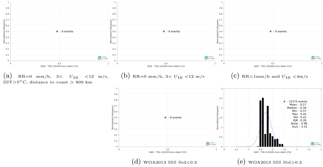
Figure 111: Normalized histogram of \Delta\text{SSS} (ISAS - TSG (LEGOS-Survostral-Adelie)) for 5 different subdatasets corresponding to: RR=0 mm/h, 3 < U_{10} < 12 m/s, SST > 5^{\circ}\text{C} , distance to coast > 800 km (a), RR=0 mm/h, 3 < U_{10} < 12 m/s (b), RR > 1\text{mm/h} and U_{10} < 4\text{m/s} (c), WOA2013 SSS Std < 0.2 (d), WOA2013 SSS Std > 0.2 (e).
