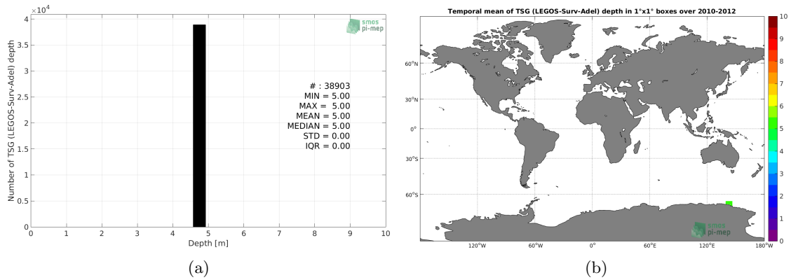
Figure 102: Depth distribution of the upper level SSS measurements from TSG (LEGOS-Survostral-Adelie) (a) and spatial distribution of the in situ SSS depth measurements showing the mean value in 1^\circ \times 1^\circ boxes and considering the full in situ dataset period (b).
