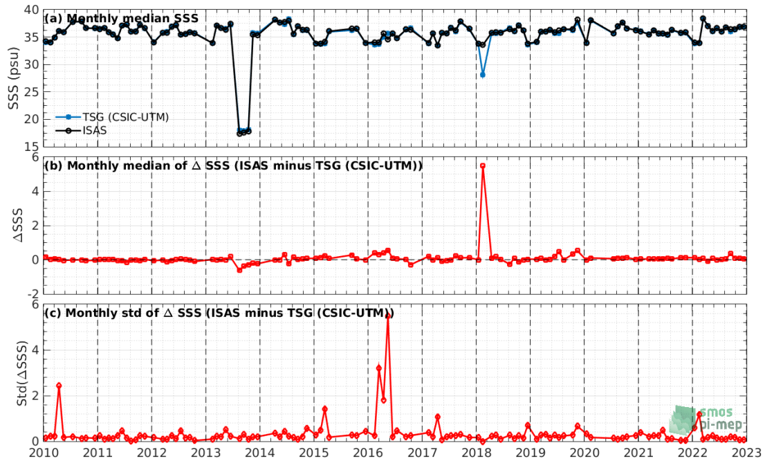
Figure 54: Time series of the monthly median SSS (top), median of \Delta SSS (ISAS - TSG (CSIC-UTM)) and Std of \Delta SSS (ISAS - TSG (CSIC-UTM)) considering all match-ups collected by the Pi-MEP.
