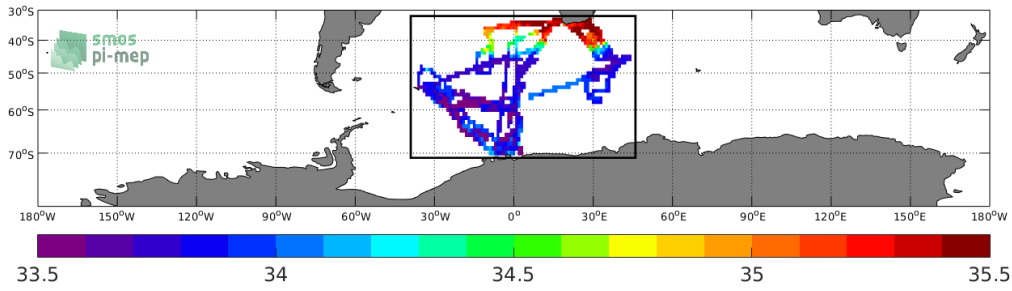
Figure 73: Location of the TSG (NCEI-0170743) dataset.
