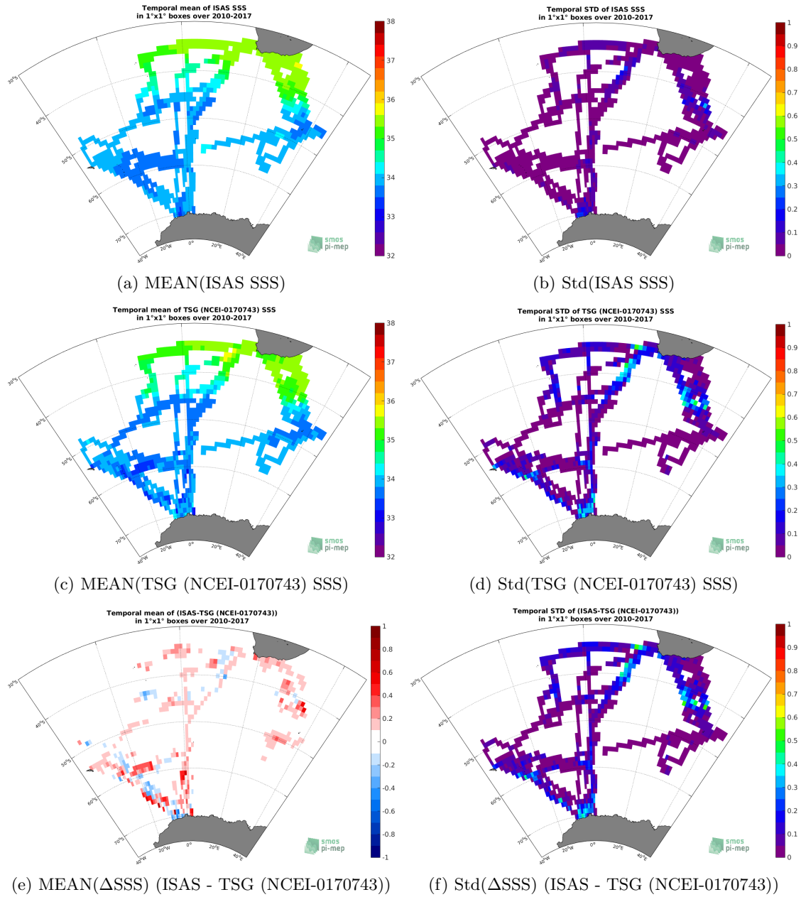
Figure 78: Temporal mean (left) and Std (right) of SSS from ISAS (top), TSG (NCEI-0170743) (middle), and of \Delta SSS (ISAS - TSG (NCEI-0170743)). Only match-up pairs are used to generate these maps.
