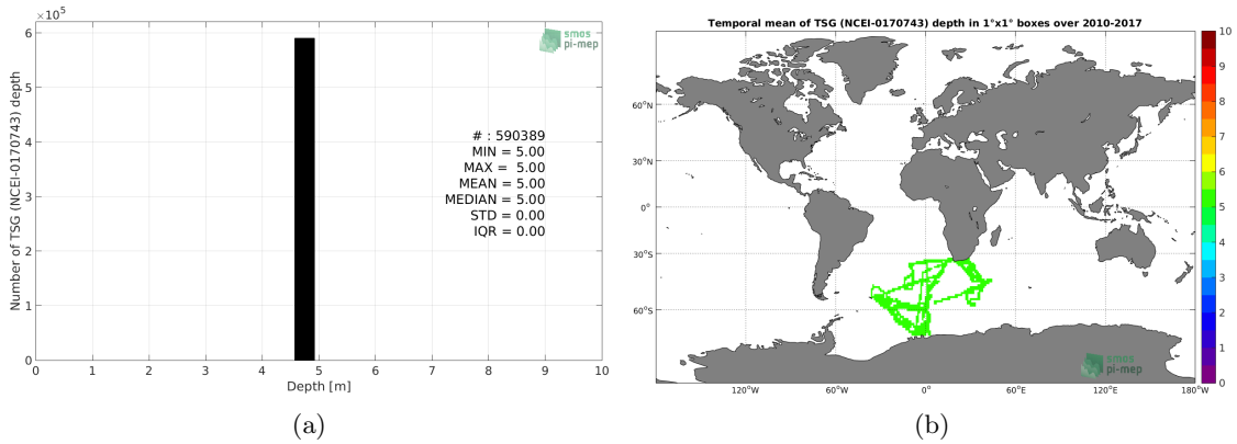
Figure 76: Depth distribution of the upper level SSS measurements from TSG (NCEI-0170743) (a) and spatial distribution of the in situ SSS depth measurements showing the mean value in 1^\circ \times 1^\circ boxes and considering the full in situ dataset period (b).
