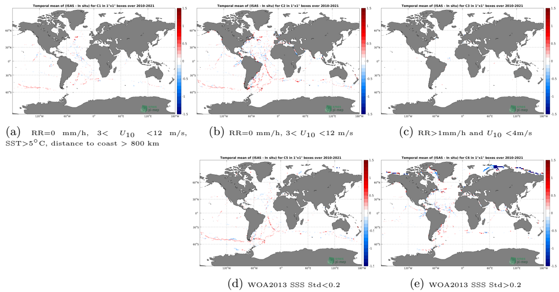
Figure 35: Temporal mean gridded over spatial boxes of size 1^\circ \times 1^\circ of \Delta\text{SSS} (ISAS - TSG (GOSUD-Sailing-ship)) for 5 different subdatasets corresponding to:RR=0 mm/h, 3 < U_{10} < 12 m/s, SST >5^\circ\text{C} , distance to coast > 800 km (a), RR=0 mm/h, 3 < U_{10} < 12 m/s (b), RR >1 mm/h and U_{10} < 4 m/s (c),WOA2013 SSS Std <0.2 (d),WOA2013 SSS Std >0.2 (e).
