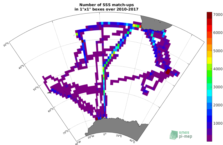
Figure 77: Number of SSS from TSG (NCEI-0170743) in 1^\circ \times 1^\circ boxes.
