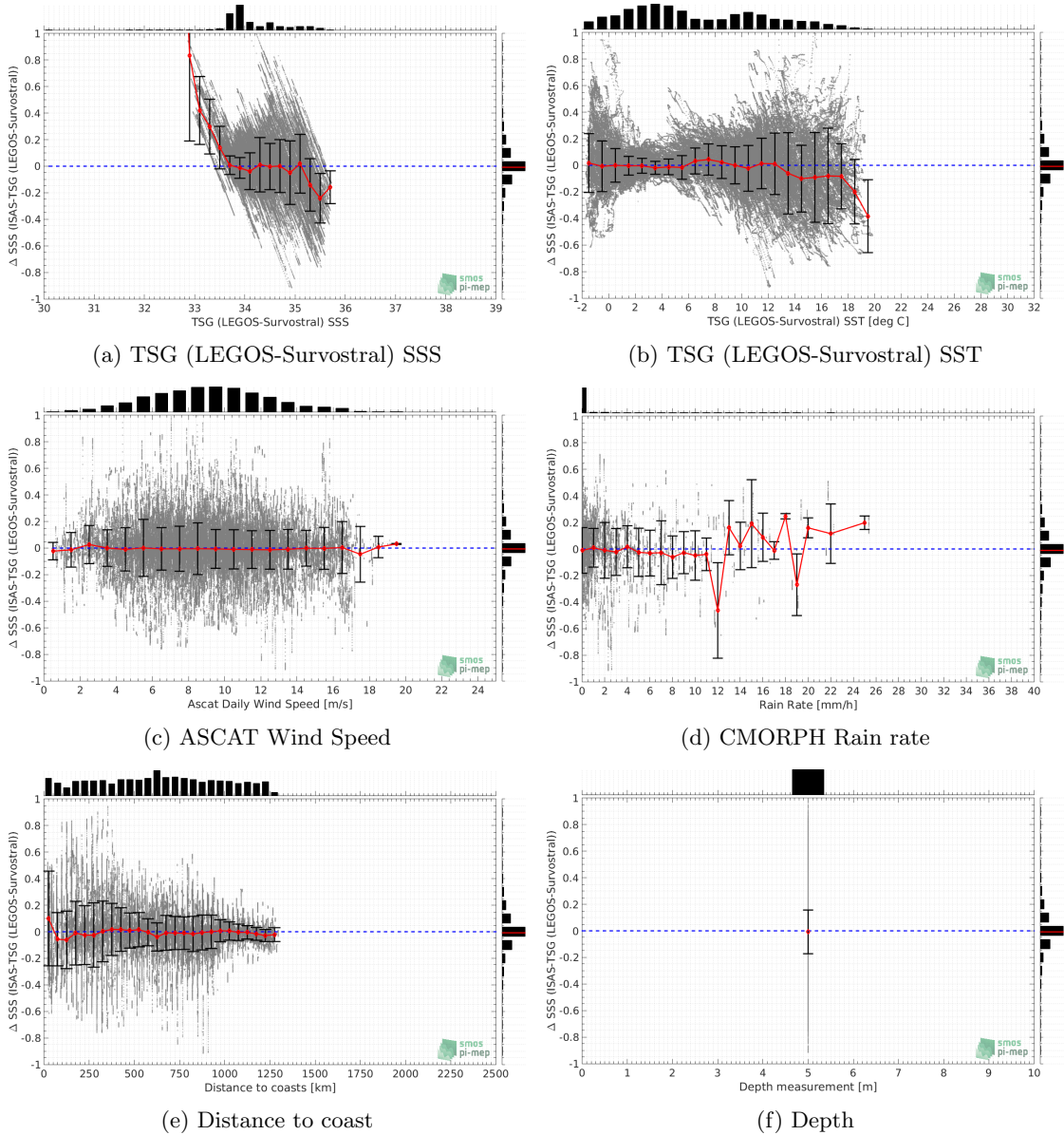
Figure 96: \Delta SSS (ISAS - TSG (LEGOS-Survostral)) sorted as geophysical conditions: TSG (LEGOS-Survostral) SSS a), TSG (LEGOS-Survostral) SST b), ASCAT Wind speed c), CMORPH rain rate d), distance to coast (e) and depth measurements (f).
