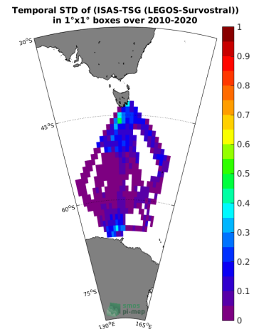
(f) Std( \Delta SSS) (ISAS - TSG (LEGOS-Survostral))
