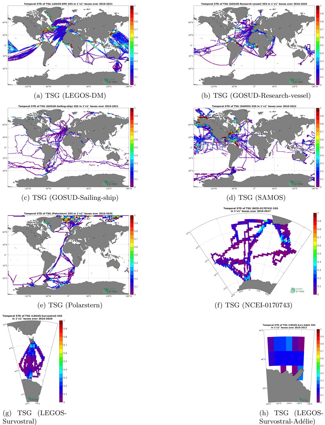
Figure 103: Temporal Std of SSS in 1^\circ \times 1^\circ boxes.
