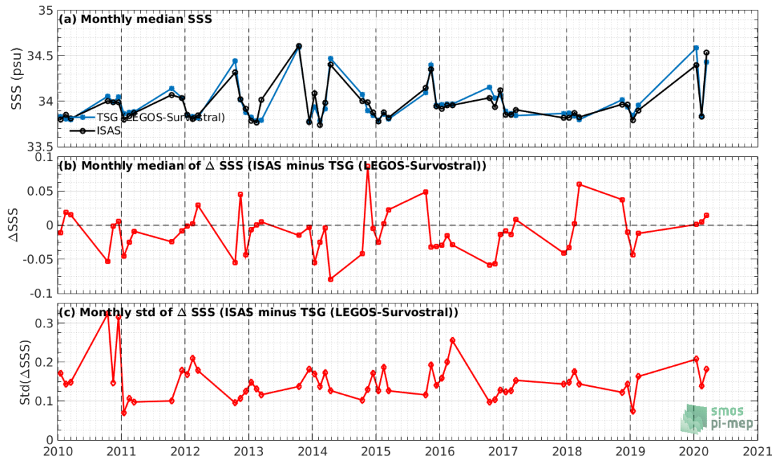
Figure 55: Time series of the monthly median SSS (top), median of \Delta SSS (ISAS - TSG (LEGOS-Survostral)) and Std of \Delta SSS (ISAS - TSG (LEGOS-Survostral)) considering all match-ups collected by the Pi-MEP.
