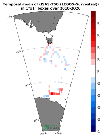
(e) MEAN( \Delta SSS) (ISAS - TSG (LEGOS-Survostral))
