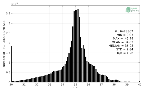
(a) TSG (LEGOS-DM)
