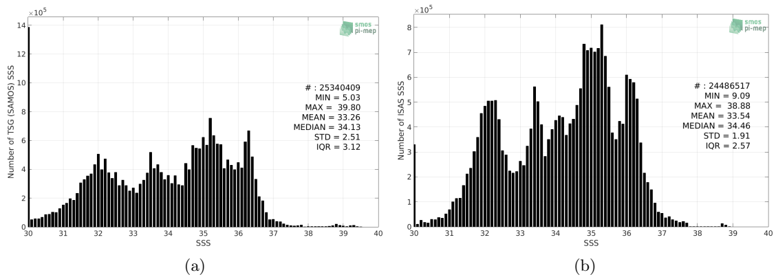
Figure 38: Histograms of SSS from TSG (SAMOS) (a) and ISAS (b) per bins of 0.1.
