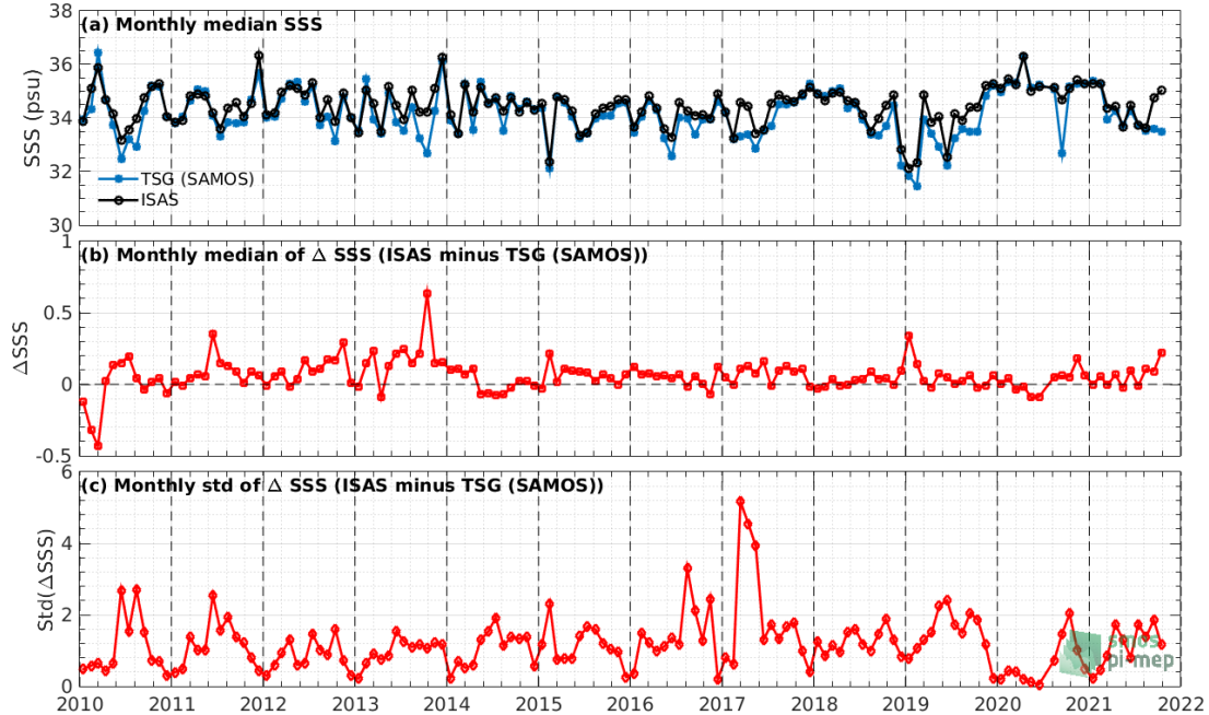
Figure 42: Time series of the monthly median SSS (top), median of \Delta SSS (ISAS - TSG (SAMOS)) and Std of \Delta SSS (ISAS - TSG (SAMOS)) considering all match-ups collected by the Pi-MEP.
