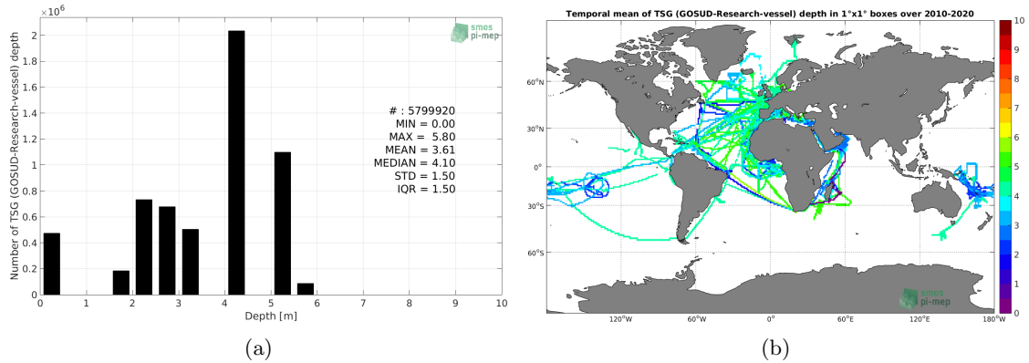
Figure 15: Depth distribution of the upper level SSS measurements from TSG (GOSUD-Research-vessel) (a) and spatial distribution of the in situ SSS depth measurements showing the mean value in 1°x1° boxes and considering the full in situ dataset period (b).
