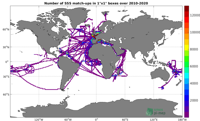
Figure 16: Number of SSS from TSG (GOSUD-Research-vessel) in 1°x1° boxes.
