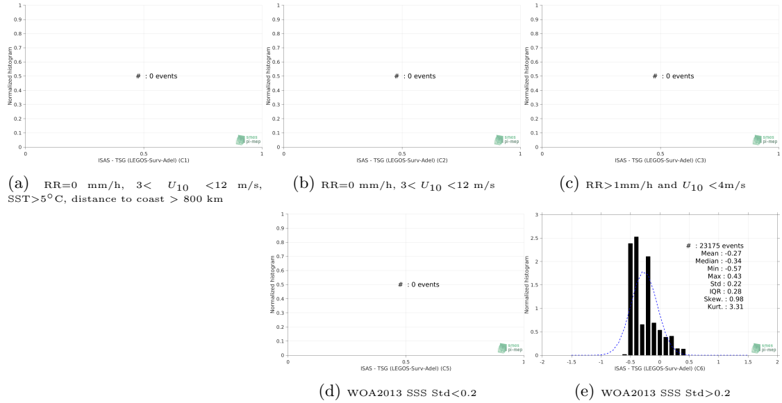
Figure 74: Normalized histogram of \Delta\text{SSS} (ISAS - TSG (LEGOS-Survostral-Adelie)) for 5 different subdatasets corresponding to: RR=0 mm/h, 3 < U_{10} < 12 m/s, SST > 5^\circ\text{C} , distance to coast > 800 km (a), RR=0 mm/h, 3 < U_{10} < 12 m/s (b), RR > 1\text{mm/h} and U_{10} < 4\text{m/s} (c), WOA2013 SSS Std < 0.2 (d), WOA2013 SSS Std > 0.2 (e).
