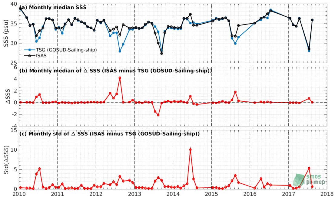
Figure 30: Time series of the monthly median SSS (top), median of \Delta SSS (ISAS - TSG (GOSUD-Sailing-ship)) and Std of \Delta SSS (ISAS - TSG (GOSUD-Sailing-ship)) considering all match-ups collected by the Pi-MEP.
