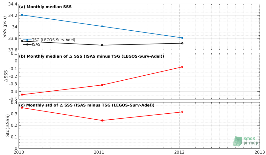
Figure 68: Time series of the monthly median SSS (top), median of \Delta SSS (ISAS - TSG (LEGOS-Survostral-Adelie)) and Std of \Delta SSS (ISAS - TSG (LEGOS-Survostral-Adelie)) considering all match-ups collected by the Pi-MEP.
