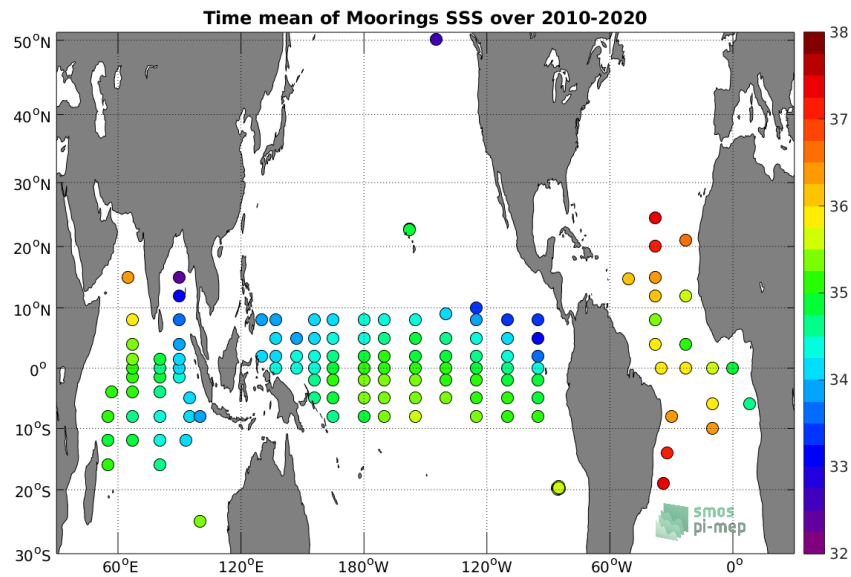
Figure 3: Time-mean SSS from Moorings.
