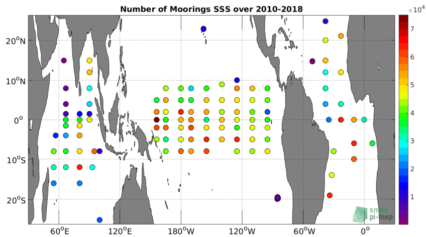
Figure 5: Number of SSS from Moorings.
