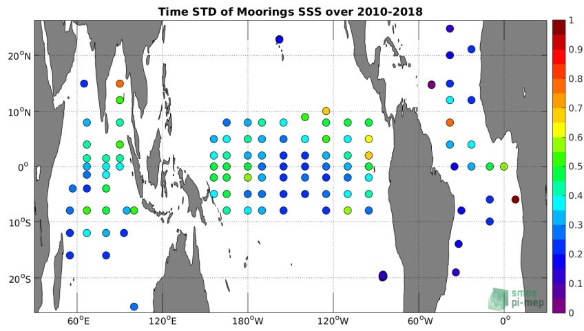
Figure 4: Temporal STD of SSS from Moorings.
