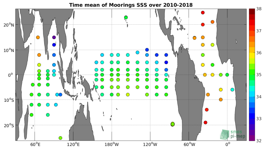
Figure 3: Time-mean SSS from Moorings.
