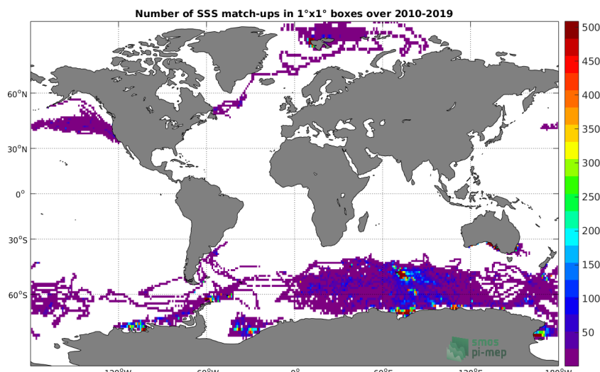
Figure 4: Number of SSS from Marine mammals in 1°x1° boxes.
