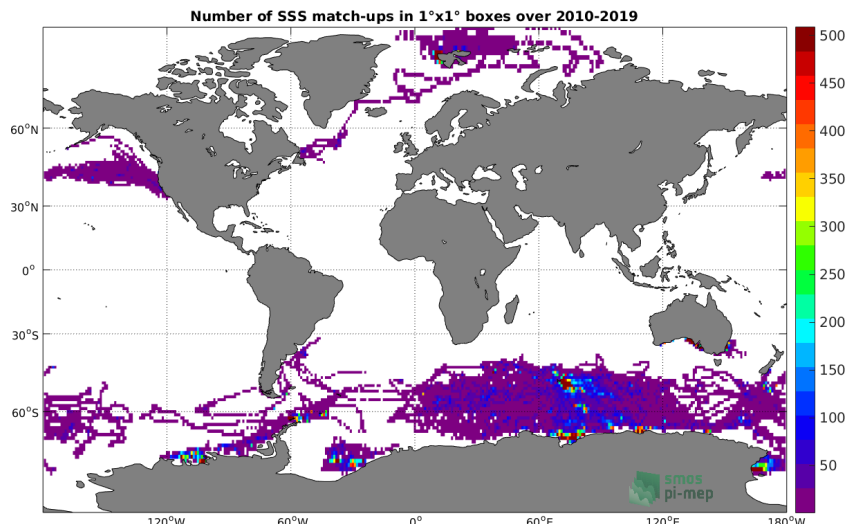
Figure 4: Number of SSS from Marine mammals in 1^\circ \times 1^\circ boxes.
