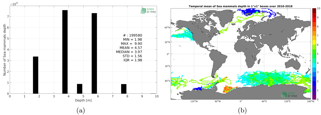
Figure 3: Depth distribution of the upper level SSS measurements from Sea mammals (a) and spatial distribution of the in situ SSS depth measurements showing the mean value in 1^{\circ} \times 1^{\circ} boxes and considering the full in situ dataset period (b).
