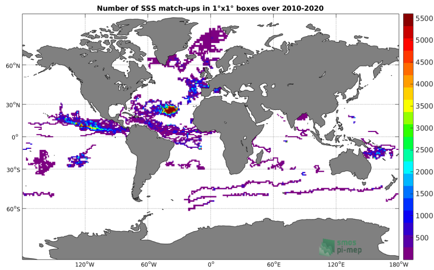
Figure 4: Number of SSS from Surface drifters in 1°x1° boxes.
