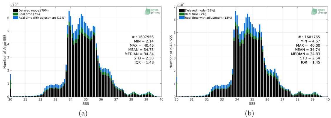
Figure 2: Histograms of SSS from Argo (a) and ISAS (b) per bins of 0.1.
