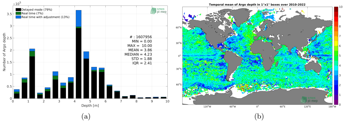
Figure 3: Depth distribution of the upper level SSS measurements from Argo (a) and spatial distribution of the in situ SSS depth measurements showing the mean value in 1^\circ \times 1^\circ boxes and considering the full in situ dataset period (b).
