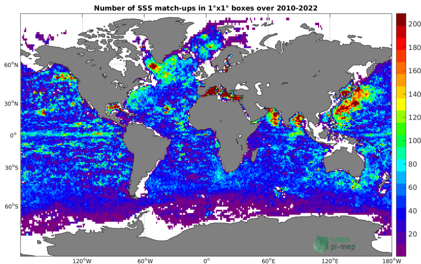
Figure 4: Number of SSS from Argo in 1^\circ \times 1^\circ boxes.
