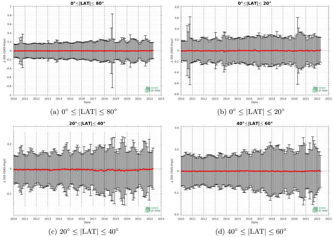
Figure 9: Monthly median (red curves) of \Delta SSS (ISAS - Argo) and \pm 1 Std (black vertical thick bars) as function of time for all the collected Pi-MEP match-up pairs for the full in situ dataset period are shown for different latitude bands: (a) 80^\circ S-80^\circ N , (b) 20^\circ S-20^\circ N , (c) 40^\circ S-20^\circ S and 20^\circ N-40^\circ N and (d) 60^\circ S-40^\circ S and 40^\circ N-60^\circ N .
