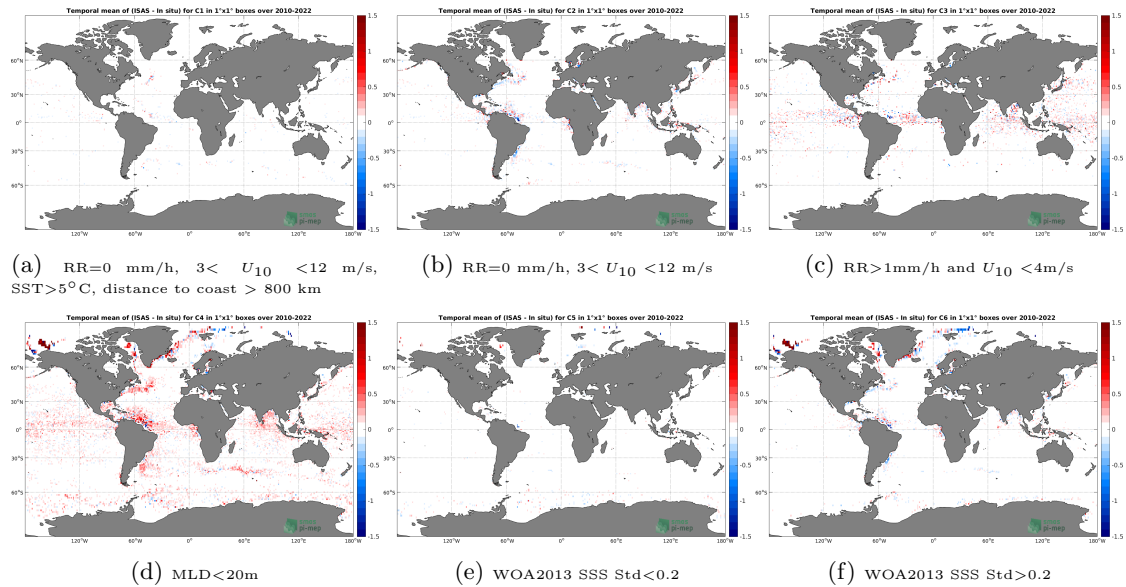
Figure 11: Temporal mean gridded over spatial boxes of size 1^\circ \times 1^\circ of \Delta SSS (ISAS - Argo) for 6 different subdatasets corresponding to:RR=0 mm/h, 3 < U_{10} < 12 m/s, SST>5°C, distance to coast > 800 km (a), RR=0 mm/h, 3 < U_{10} < 12 m/s (b), RR>1mm/h and U_{10} < 4 m/s (c),MLD<20m (d),WOA2013 SSS Std<0.2 (e),WOA2013 SSS Std>0.2 (f).
