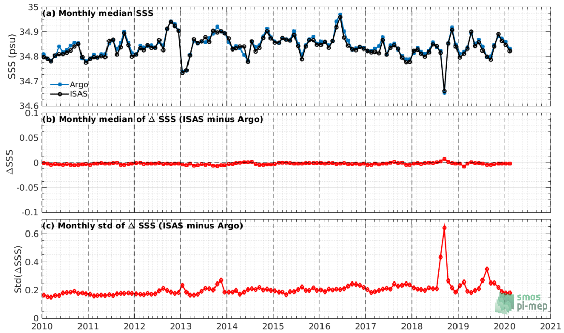
Figure 6: Time series of the monthly median SSS (top), median of \Delta SSS (ISAS - Argo) and Std of \Delta SSS (ISAS - Argo) considering all match-ups collected by the Pi-MEP.
