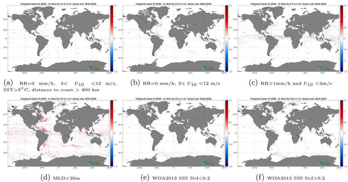
Figure 11: Temporal mean gridded over spatial boxes of size 1^\circ \times 1^\circ of \Delta SSS (ISAS - Argo) for 6 different subdatasets corresponding to: RR=0 mm/h, 3 < U_{10} < 12 m/s, SST > 5^\circ\text{C} , distance to coast > 800 km (a), RR=0 mm/h, 3 < U_{10} < 12 m/s (b), RR > 1 mm/h and U_{10} < 4 m/s (c), MLD < 20 m (d), WOA2013 SSS Std < 0.2 (e), WOA2013 SSS Std > 0.2 (f).
