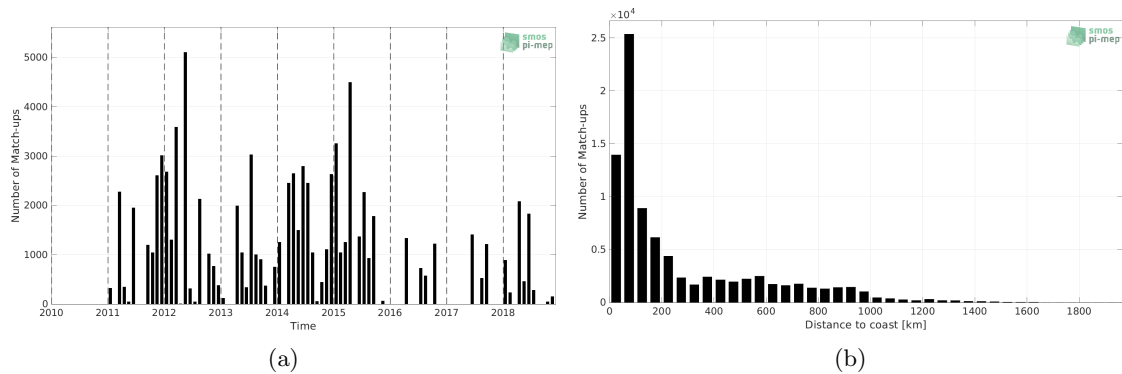
Figure 1: Number of match-ups between TSG (LEGOS-DM) and SMOS and SMAP SSS L4 OI v1 - 7 Days (LOPS) SSS as a function of time (a) and as function of the distance to coast (b) over the Gulf Stream Pi-MEP region and for the full satellite product period.
