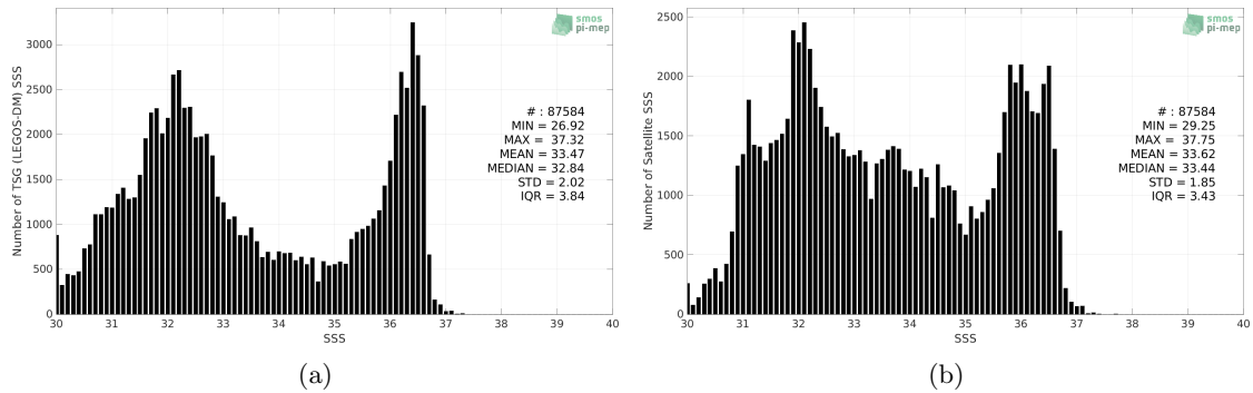
Figure 2: Histograms of SSS from TSG (LEGOS-DM) (a) and SMOS and SMAP SSS L4 OI v1 - 7 Days (LOPS) (b) considering all match-up pairs per bins of 0.1 over the Gulf Stream Pi-MEP region and for the full satellite product period.
