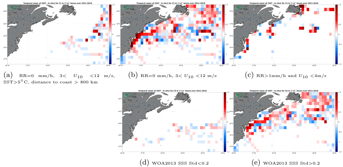
Figure 12: Temporal mean gridded over spatial boxes of size 1^{\circ}\times 1^{\circ} of \Delta\text{SSS} (SMOS and SMAP SSS L4 OI v1 - 7 Days (LOPS) - TSG (LEGOS-DM)) for 5 different subdatasets corresponding to:RR=0 mm/h, 3 < U_{10} < 12 m/s, SST >5^{\circ}\text{C} , distance to coast > 800 km (a), RR=0 mm/h, 3 < U_{10} < 12 m/s (b), RR >1 mm/h and U_{10} < 4 m/s (c), WOA2013 SSS Std <0.2 (d), WOA2013 SSS Std >0.2 (e).
