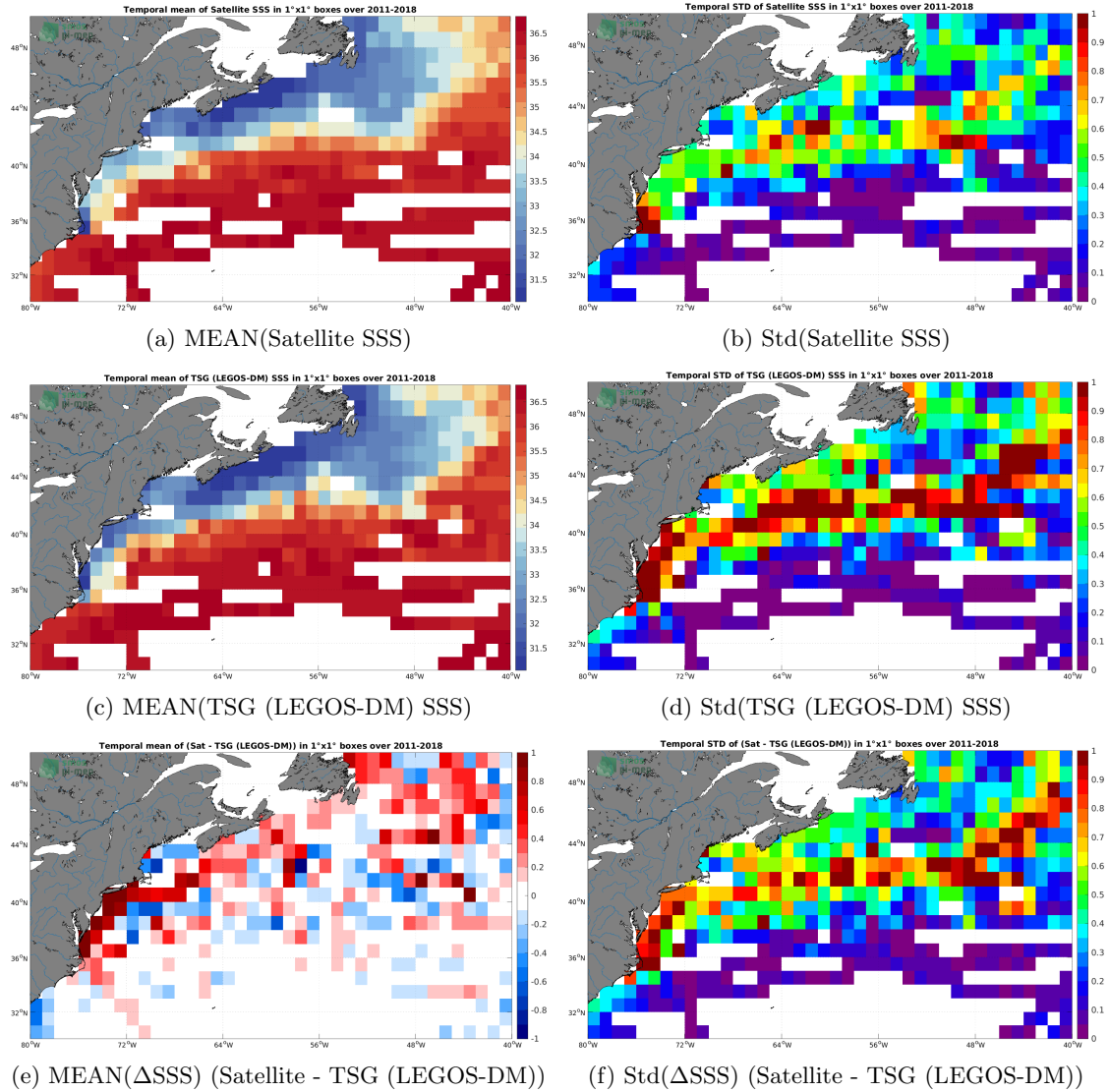
Figure 6: Temporal mean (left) and Std (right) of SSS from SMOS and SMAP SSS L4 OI v1 - 7 Days (LOPS) (top), TSG (LEGOS-DM) (middle), and of \Delta SSS (Satellite - TSG (LEGOS-DM)). Only match-up pairs are used to generate these maps.
