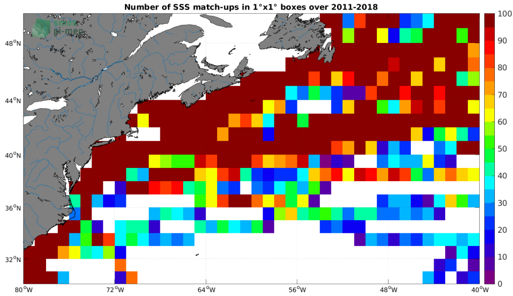
Figure 4: Number of SSS match-ups between TSG (LEGOS-DM) SSS and the SMOS and SMAP SSS L4 OI v1 - 7 Days (LOPS) SSS product for the Gulf Stream Pi-MEP region over 1^\circ \times 1^\circ boxes and for the full satellite product period.
