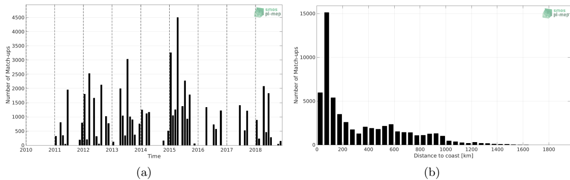
Figure 1: Number of match-ups between TSG (LEGOS-DM) and SMOS and SMAP SSS L4 OI v1 - 7 Days (LOPS) SSS as a function of time (a) and as function of the distance to coast (b) over the Gulf Stream Pi-MEP region and for the full satellite product period.
