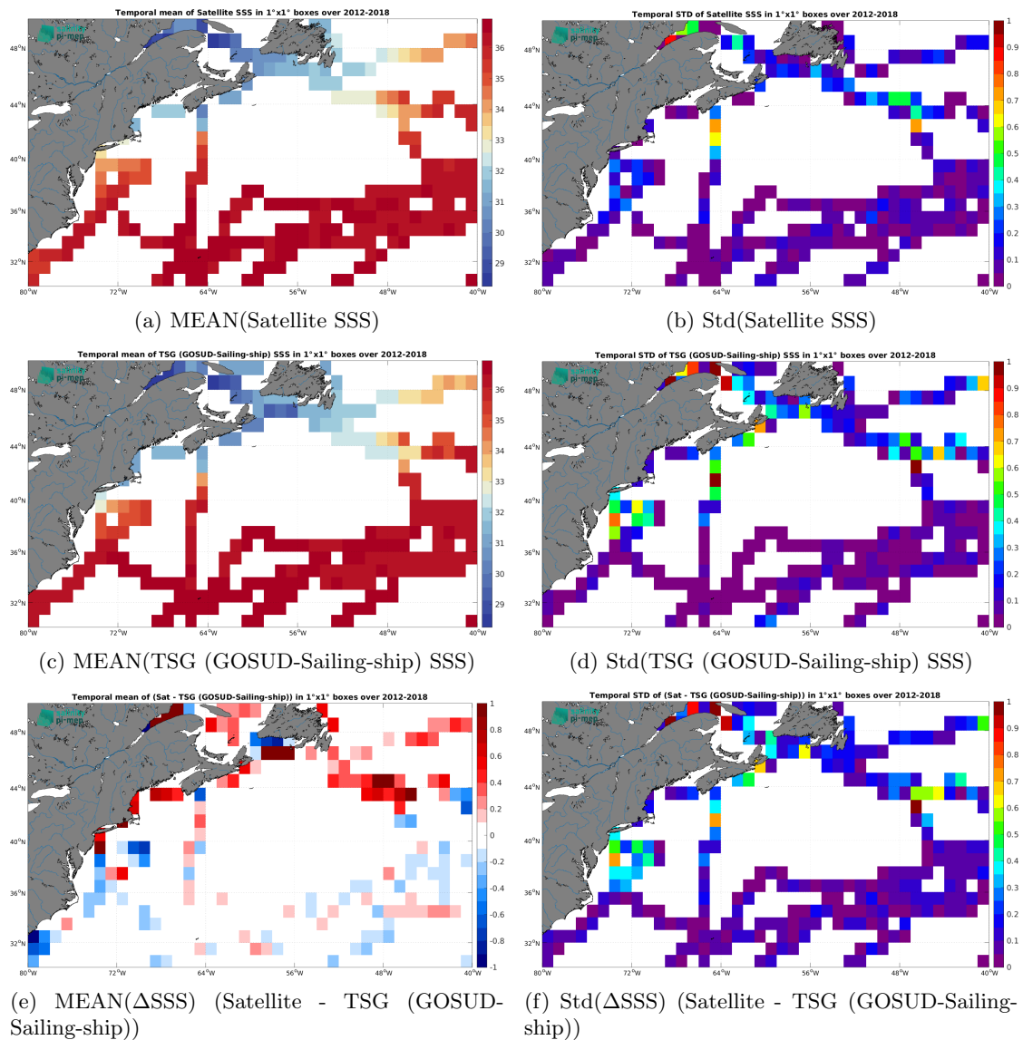
Figure 6: Temporal mean (left) and Std (right) of SSS from SMOS and SMAP SSS L4 OI v1 - 7 Days (LOPS) (top), TSG (GOSUD-Sailing-ship) (middle), and of \Delta SSS (Satellite - TSG (GOSUD-Sailing-ship)). Only match-up pairs are used to generate these maps.
