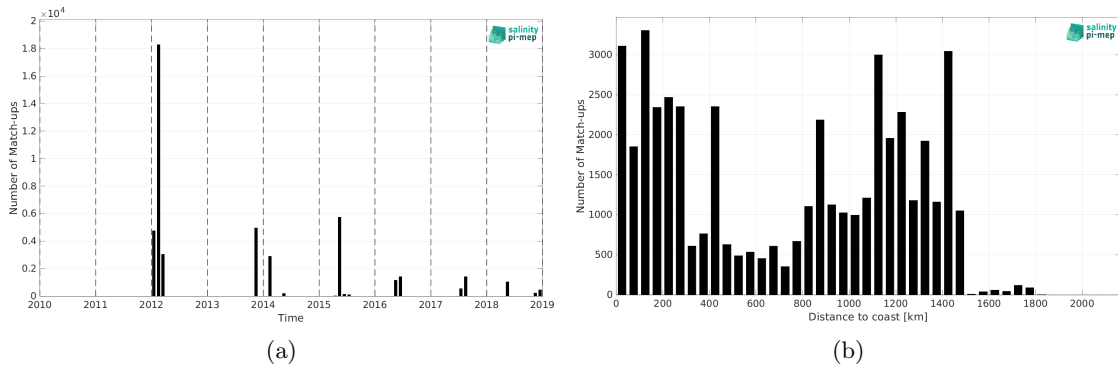
Figure 1: Number of match-ups between TSG (GOSUD-Sailing-ship) and SMOS and SMAP SSS L4 OI v1 - 7 Days (LOPS) SSS as a function of time (a) and as function of the distance to coast (b) over the Gulf Stream Pi-MEP region and for the full satellite product period.
