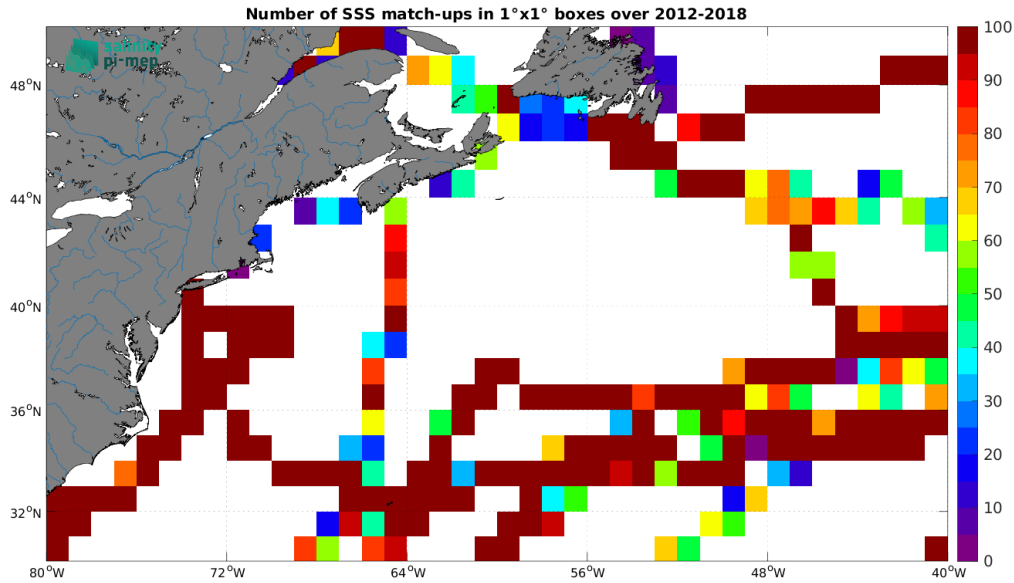
Figure 4: Number of SSS match-ups between TSG (GOSUD-Sailing-ship) SSS and the SMOS and SMAP SSS L4 OI v1 - 7 Days (LOPS) SSS product for the Gulf Stream Pi-MEP region over 1^\circ \times 1^\circ boxes and for the full satellite product period.
