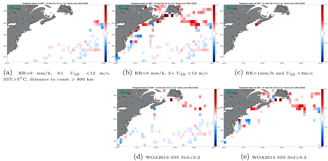
Figure 12: Temporal mean gridded over spatial boxes of size 1^{\circ}\times 1^{\circ} of \Delta SSS (SMOS and SMAP SSS L4 OI v1 - 7 Days (LOPS) - TSG (GOSUD-Sailing-ship)) for 5 different subdatasets corresponding to:RR=0 mm/h, 3 < U_{10} < 12 m/s, SST >5^{\circ}\text{C} , distance to coast > 800 km (a), RR=0 mm/h, 3 < U_{10} < 12 m/s (b), RR >1 mm/h and U_{10} < 4 m/s (c), WOA2013 SSS Std <0.2 (d), WOA2013 SSS Std >0.2 (e).
