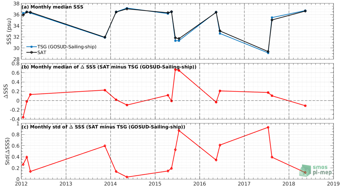
Figure 7: Time series of the monthly median SSS (top), median of \Delta\text{SSS} (Satellite - TSG (GOSUD-Sailing-ship)) and Std of \Delta\text{SSS} (Satellite - TSG (GOSUD-Sailing-ship)) over the Gulf Stream Pi-MEP region considering all match-ups collected by the Pi-MEP.
