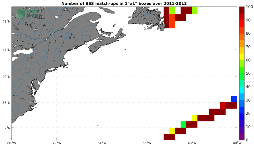
Figure 4: Number of SSS match-ups between TSG (CSIC-UTM) SSS and the SMOS and SMAP SSS L4 OI v1 - 7 Days (LOPS) SSS product for the Gulf Stream Pi-MEP region over 1^\circ \times 1^\circ boxes and for the full satellite product period.
