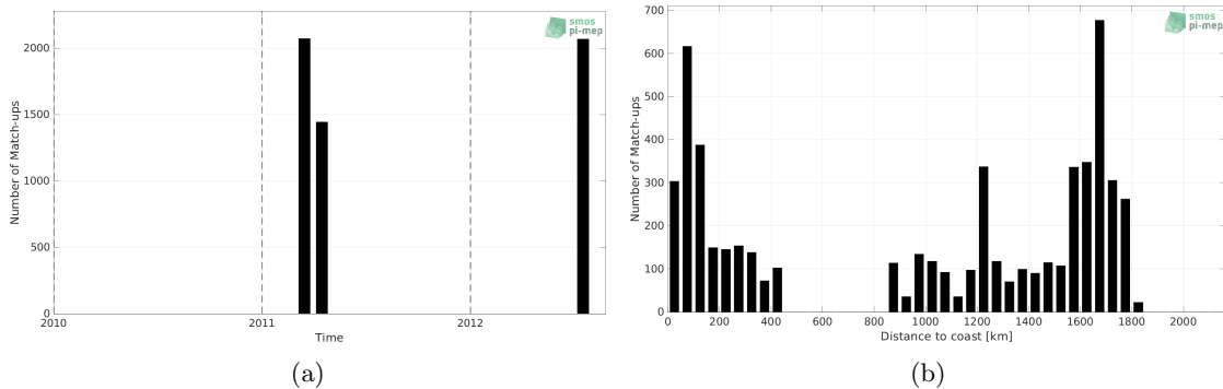
Figure 1: Number of match-ups between TSG (CSIC-UTM) and SMOS and SMAP SSS L4 OI v1 - 7 Days (LOPS) SSS as a function of time (a) and as function of the distance to coast (b) over the Gulf Stream Pi-MEP region and for the full satellite product period.
