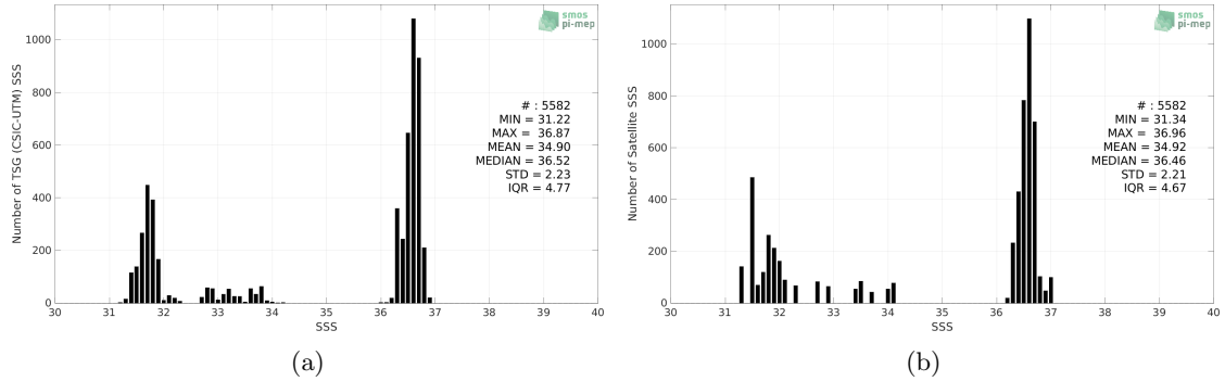
Figure 2: Histograms of SSS from TSG (CSIC-UTM) (a) and SMOS and SMAP SSS L4 OI v1 - 7 Days (LOPS) (b) considering all match-up pairs per bins of 0.1 over the Gulf Stream Pi-MEP region and for the full satellite product period.
