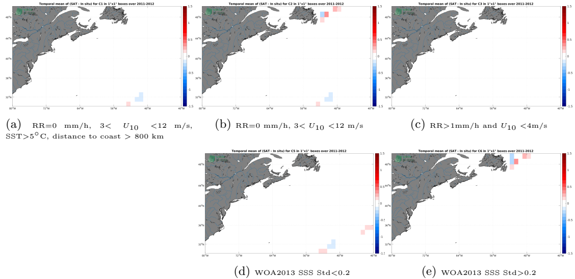
Figure 12: Temporal mean gridded over spatial boxes of size 1^{\circ}\times 1^{\circ} of \Delta\text{SSS} (SMOS and SMAP SSS L4 OI v1 - 7 Days (LOPS) - TSG (CSIC-UTM)) for 5 different subdatasets corresponding to:RR=0 mm/h, 3 < U_{10} < 12 m/s, SST >5^{\circ}\text{C} , distance to coast > 800 km (a), RR=0 mm/h, 3 < U_{10} < 12 m/s (b), RR >1 mm/h and U_{10} < 4 m/s (c), WOA2013 SSS Std <0.2 (d), WOA2013 SSS Std >0.2 (e).
