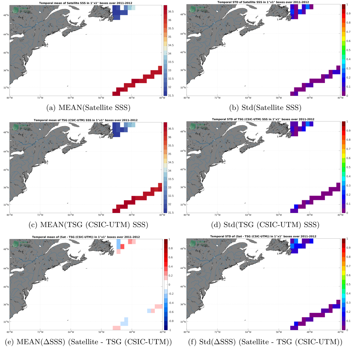
Figure 6: Temporal mean (left) and Std (right) of SSS from SMOS and SMAP SSS L4 OI v1 - 7 Days (LOPS) (top), TSG (CSIC-UTM) (middle), and of \Delta SSS (Satellite - TSG (CSIC-UTM)). Only match-up pairs are used to generate these maps.
