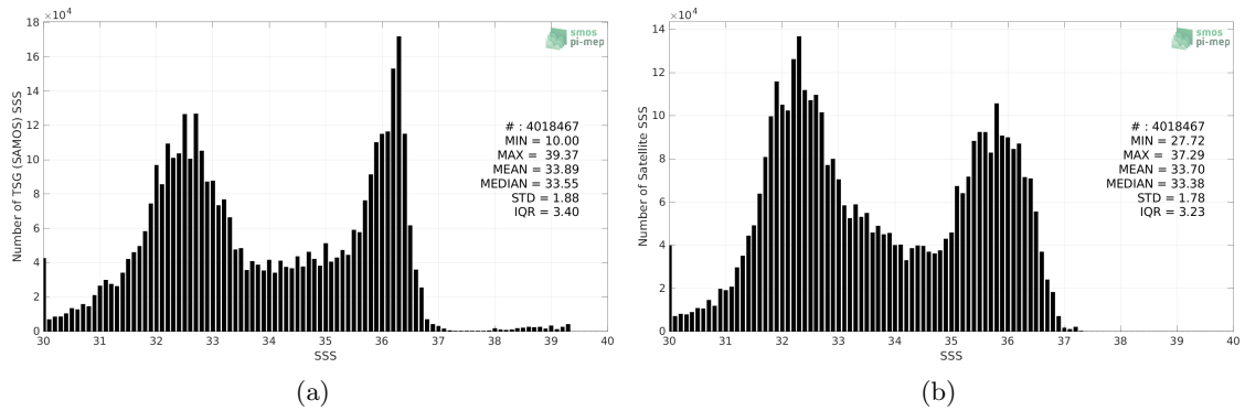
Figure 2: Histograms of SSS from TSG (SAMOS) (a) and SMOS SSS L4 v1 - Weekly (CMEMS-CNR) (b) considering all match-up pairs per bins of 0.1 over the Gulf Stream Pi-MEP region and for the full satellite product period.
