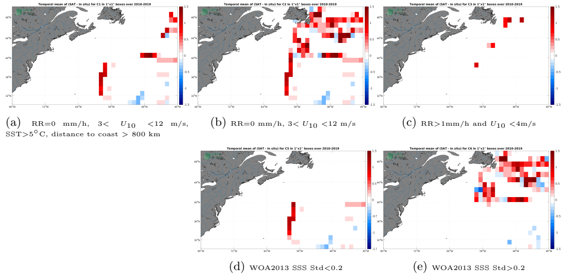
Figure 12: Temporal mean gridded over spatial boxes of size 1^{\circ}\times 1^{\circ} of \Delta SSS (SMOS SSS L4 v1 - Weekly (CMEMS-CNR) - TSG (GOSUD-Research-vessel)) for 5 different subdatasets corresponding to: RR=0 mm/h, 3 < U_{10} < 12 m/s, SST > 5^{\circ}\text{C} , distance to coast > 800 km (a), RR=0 mm/h, 3 < U_{10} < 12 m/s (b), RR > 1 mm/h and U_{10} < 4 m/s (c), WOA2013 SSS Std < 0.2 (d), WOA2013 SSS Std > 0.2 (e).
