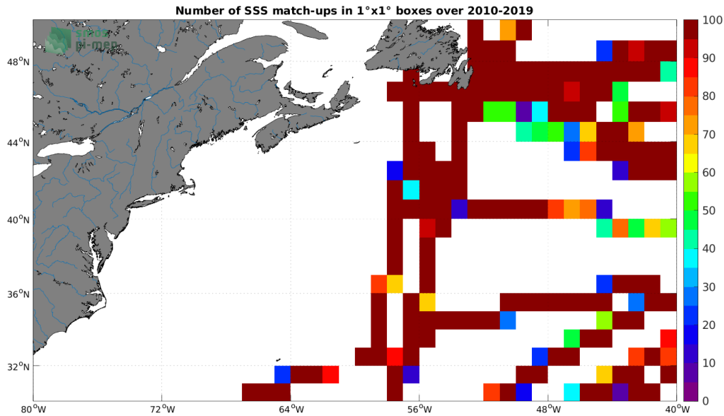
Figure 4: Number of SSS match-ups between TSG (GOSUD-Research-vessel) SSS and the SMOS SSS L4 v1 - Weekly (CMEMS-CNR) SSS product for the Gulf Stream Pi-MEP region over 1^\circ \times 1^\circ boxes and for the full satellite product period.
