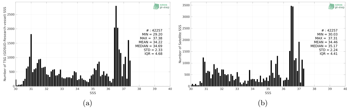
Figure 2: Histograms of SSS from TSG (GOSUD-Research-vessel) (a) and SMOS SSS L4 v1 - Weekly (CMEMS-CNR) (b) considering all match-up pairs per bins of 0.1 over the Gulf Stream Pi-MEP region and for the full satellite product period.
