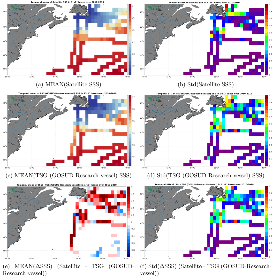
Figure 6: Temporal mean (left) and Std (right) of SSS from SMOS SSS L4 v1 - Weekly (CMEMS-CNR) (top), TSG (GOSUD-Research-vessel) (middle), and of \Delta SSS (Satellite - TSG (GOSUD-Research-vessel)). Only match-up pairs are used to generate these maps.
