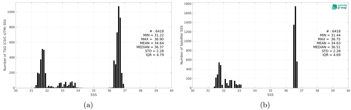
Figure 2: Histograms of SSS from TSG (CSIC-UTM) (a) and SMOS SSS L4 v1 - Weekly (CMEMS-CNR) (b) considering all match-up pairs per bins of 0.1 over the Gulf Stream Pi-MEP region and for the full satellite product period.
