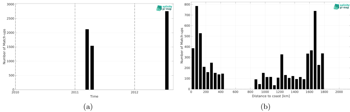
Figure 1: Number of match-ups between TSG (CSIC-UTM) and SMOS SSS L4 v1 - Weekly (CMEMS-CNR) SSS as a function of time (a) and as function of the distance to coast (b) over the Gulf Stream Pi-MEP region and for the full satellite product period.
