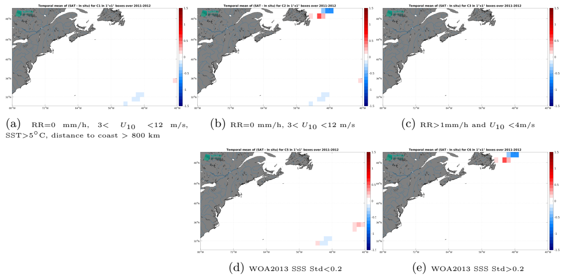
Figure 12: Temporal mean gridded over spatial boxes of size 1^\circ \times 1^\circ of \Delta SSS (SMOS SSS L4 v1 - Weekly (CMEMS-CNR) - TSG (CSIC-UTM)) for 5 different subdatasets corresponding to:RR=0 mm/h, 3 < U_{10} < 12 m/s, SST >5^\circ C, distance to coast > 800 km (a), RR=0 mm/h, 3 < U_{10} < 12 m/s (b), RR >1 mm/h and U_{10} < 4 m/s (c), WOA2013 SSS Std <0.2 (d), WOA2013 SSS Std >0.2 (e).
