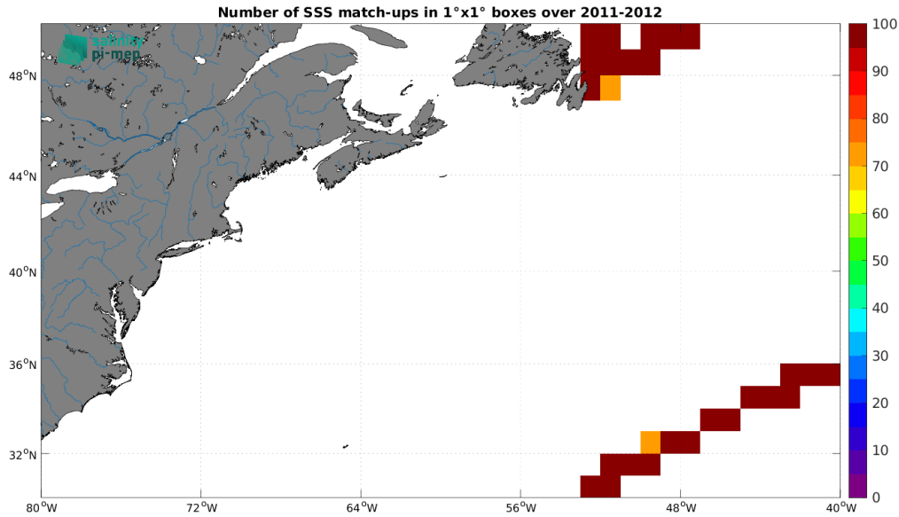
Figure 4: Number of SSS match-ups between TSG (CSIC-UTM) SSS and the SMOS SSS L4 v1 - Weekly (CMEMS-CNR) SSS product for the Gulf Stream Pi-MEP region over 1^\circ \times 1^\circ boxes and for the full satellite product period.
