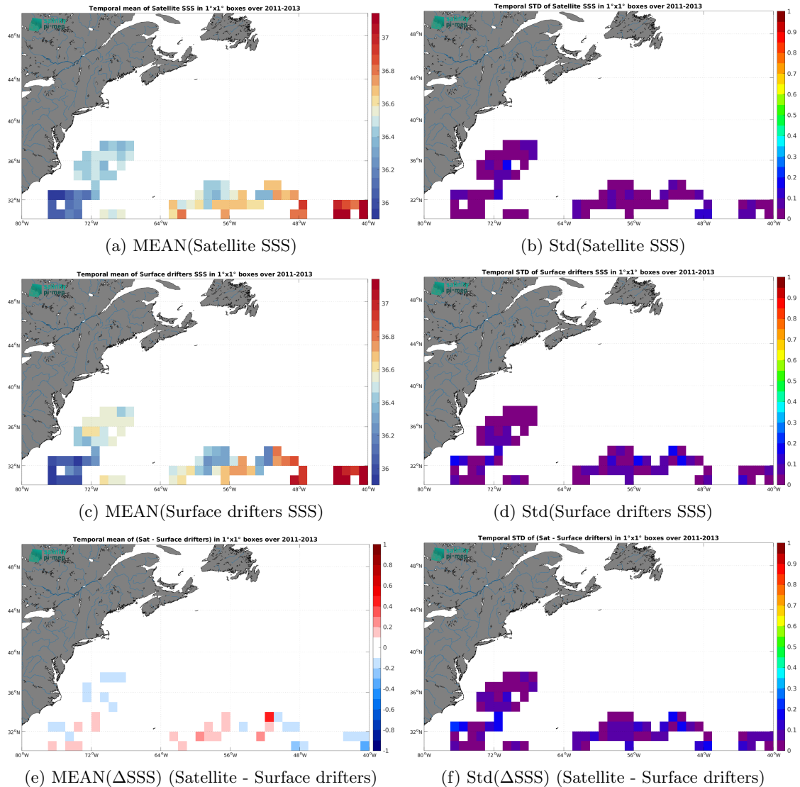
Figure 5: Temporal mean (left) and Std (right) of SSS from SMOS SSS L4 v1 - Weekly (CMEMS-CNR) (top), Surface drifters (middle), and of \Delta SSS (Satellite - Surface drifters). Only match-up pairs are used to generate these maps.
