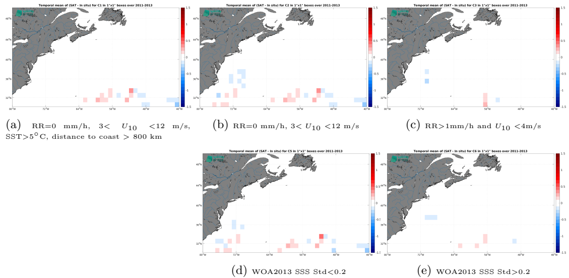
Figure 11: Temporal mean gridded over spatial boxes of size 1^{\circ}\times 1^{\circ} of \Delta\text{SSS} (SMOS SSS L4 v1 - Weekly (CMEMS-CNR) - Surface drifters) for 5 different subdatasets corresponding to:RR=0 mm/h, 3 < U_{10} < 12 m/s, SST >5^{\circ}\text{C} , distance to coast > 800 km (a), RR=0 mm/h, 3 < U_{10} < 12 m/s (b), RR >1 mm/h and U_{10} < 4 m/s (c), WOA2013 SSS Std <0.2 (d), WOA2013 SSS Std >0.2 (e).
