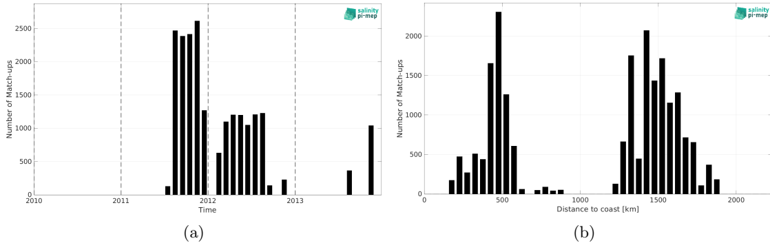
Figure 1: Number of match-ups between Surface drifters and SMOS SSS L4 v1 - Weekly (CMEMS-CNR) SSS as a function of time (a) and as function of the distance to coast (b) over the Gulf Stream Pi-MEP region and for the full satellite product period.
