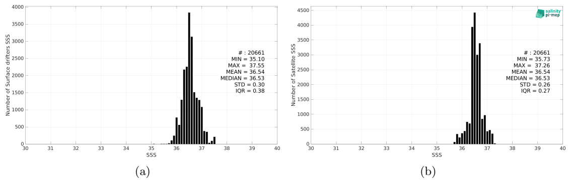
Figure 2: Histograms of SSS from Surface drifters (a) and SMOS SSS L4 v1 - Weekly (CMEMS-CNR) (b) considering all match-up pairs per bins of 0.1 over the Gulf Stream Pi-MEP region and for the full satellite product period.
