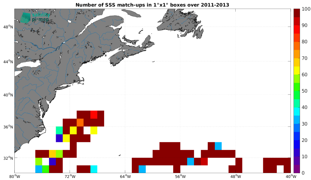
Figure 3: Number of SSS match-ups between Surface drifters SSS and the SMOS SSS L4 v1 - Weekly (CMEMS-CNR) SSS product for the Gulf Stream Pi-MEP region over 1^\circ \times 1^\circ boxes and for the full satellite product period.
