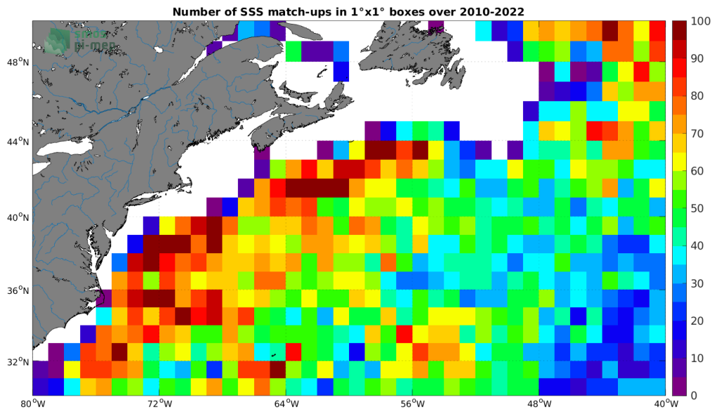
Figure 4: Number of SSS match-ups between Argo SSS and the SMOS SSS L4 v1 - Weekly (CMEMS-CNR) SSS product for the Gulf Stream Pi-MEP region over 1^\circ \times 1^\circ boxes and for the full satellite product period.
