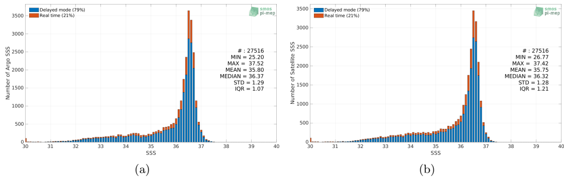
Figure 2: Histograms of SSS from Argo (a) and SMOS SSS L4 v1 - Weekly (CMEMS-CNR) (b) considering all match-up pairs per bins of 0.1 over the Gulf Stream Pi-MEP region and for the full satellite product period.
