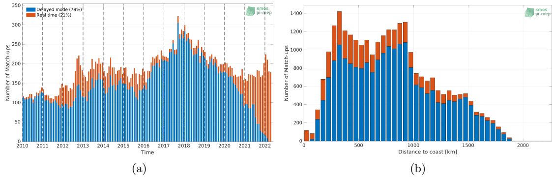
Figure 1: Number of match-ups between Argo and SMOS SSS L4 v1 - Weekly (CMEMS-CNR) SSS as a function of time (a) and as function of the distance to coast (b) over the Gulf Stream Pi-MEP region and for the full satellite product period.
