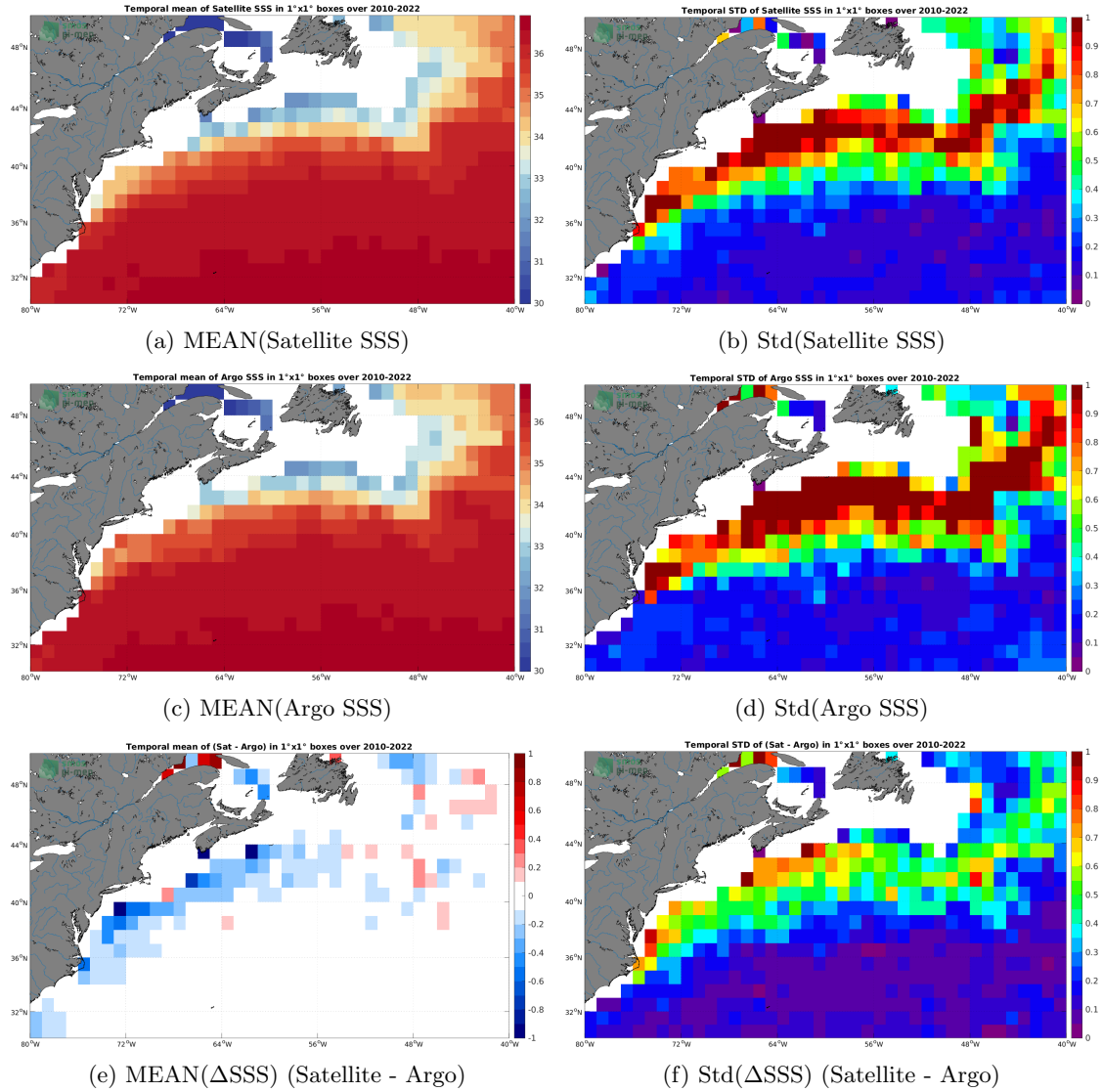
Figure 6: Temporal mean (left) and Std (right) of SSS from SMOS SSS L4 v1 - Weekly (CMEMS-CNR) (top), Argo (middle), and of \Delta SSS (Satellite - Argo). Only match-up pairs are used to generate these maps.
