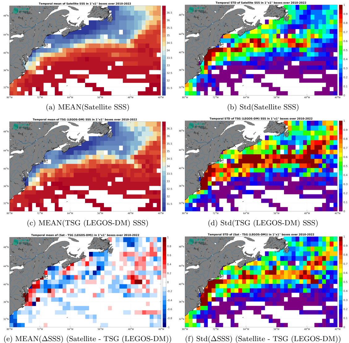
Figure 7: Temporal mean (left) and Std (right) of SSS from SMOS SSS L4 v1 - Monthly (CMEMS-CNR) (top), TSG (LEGOS-DM) (middle), and of \Delta SSS (Satellite - TSG (LEGOS-DM)). Only match-up pairs are used to generate these maps.
