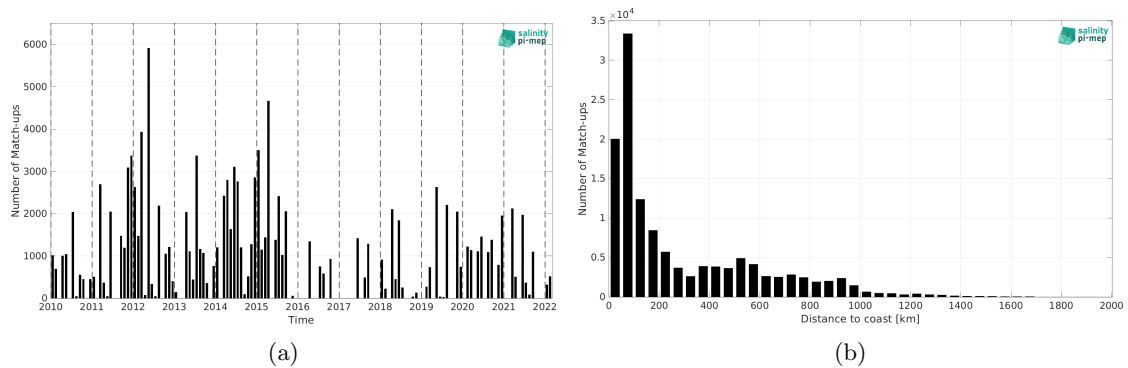
Figure 2: Number of match-ups between TSG (LEGOS-DM) and SMOS SSS L4 v1 - Monthly (CMEMS-CNR) SSS as a function of time (a) and as function of the distance to coast (b) over the Gulf Stream Pi-MEP region and for the full satellite product period.
