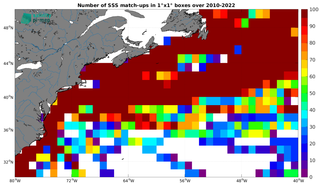
Figure 5: Number of SSS match-ups between TSG (LEGOS-DM) SSS and the SMOS SSS L4 v1 - Monthly (CMEMS-CNR) SSS product for the Gulf Stream Pi-MEP region over 1^\circ \times 1^\circ boxes and for the full satellite product period.
