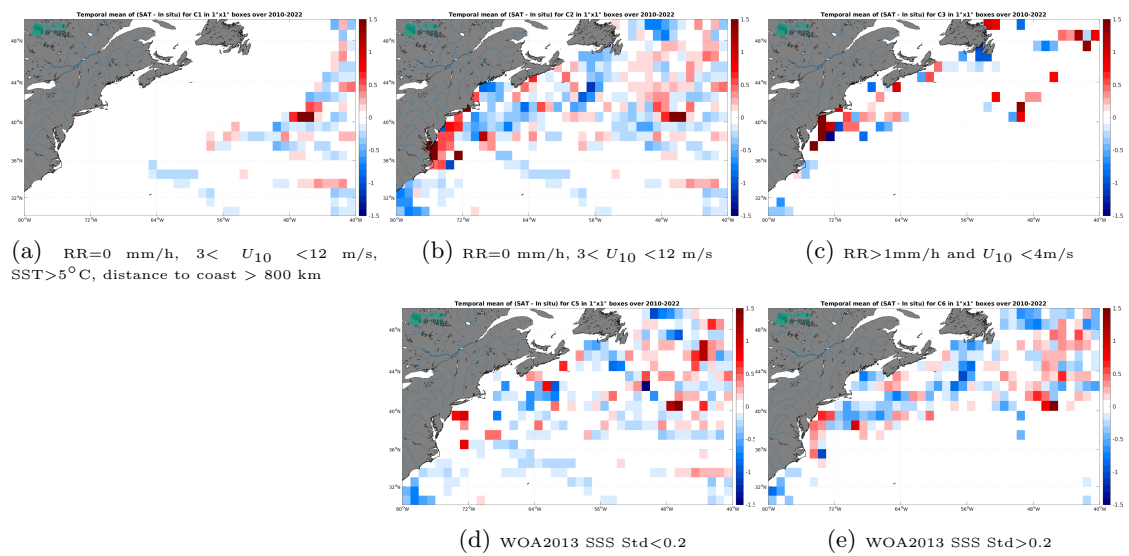
Figure 14: Temporal mean gridded over spatial boxes of size 1^\circ \times 1^\circ of \Delta SSS (SMOS SSS L4 v1 - Monthly (CMEMS-CNR) - TSG (LEGOS-DM)) for 5 different subdatasets corresponding to: RR=0 mm/h, 3 < U_{10} < 12 m/s, SST > 5°C, distance to coast > 800 km (a), RR=0 mm/h, 3 < U_{10} < 12 m/s (b), RR > 1mm/h and U_{10} < 4 m/s (c), WOA2013 SSS Std < 0.2 (d), WOA2013 SSS Std > 0.2 (e).
