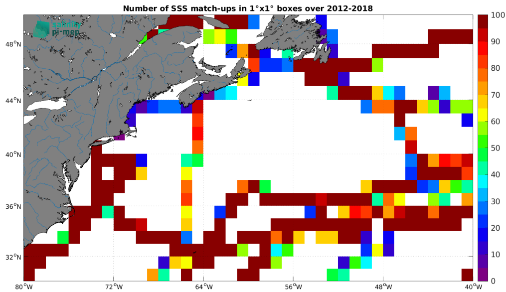
Figure 5: Number of SSS match-ups between TSG (GOSUD-Sailing-ship) SSS and the SMOS SSS L4 v1 - Monthly (CMEMS-CNR) SSS product for the Gulf Stream Pi-MEP region over 1^\circ \times 1^\circ boxes and for the full satellite product period.
