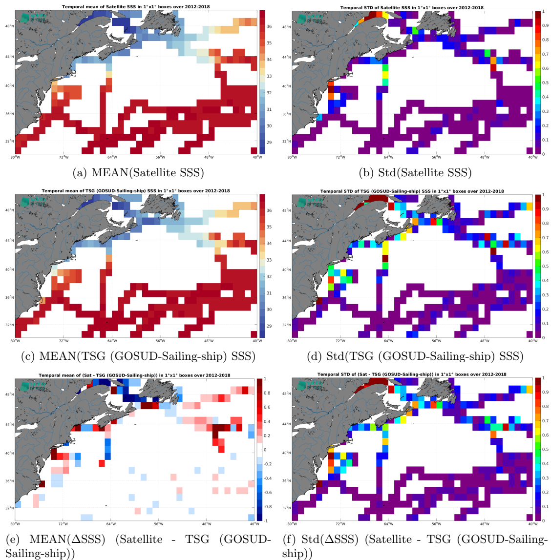
Figure 7: Temporal mean (left) and Std (right) of SSS from SMOS SSS L4 v1 - Monthly (CMEMS-CNR) (top), TSG (GOSUD-Sailing-ship) (middle), and of \Delta SSS (Satellite - TSG (GOSUD-Sailing-ship)). Only match-up pairs are used to generate these maps.
