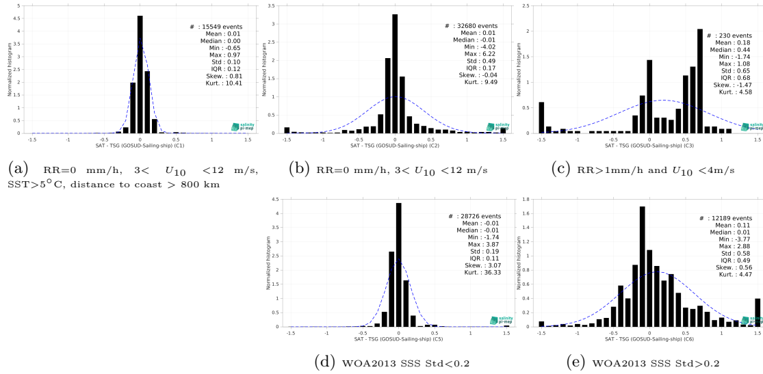
Figure 15: Normalized histogram of \Delta SSS (SMOS SSS L4 v1 - Monthly (CMEMS-CNR) - TSG (GOSUD-Sailing-ship)) for 5 different subdatasets corresponding to: RR=0 mm/h, 3 < U_{10} < 12 m/s, SST>5°C, distance to coast > 800 km (a), RR=0 mm/h, 3 < U_{10} < 12 m/s (b), RR>1mm/h and U_{10} < 4 m/s (c), WOA2013 SSS Std<0.2 (d), WOA2013 SSS Std>0.2 (e).
