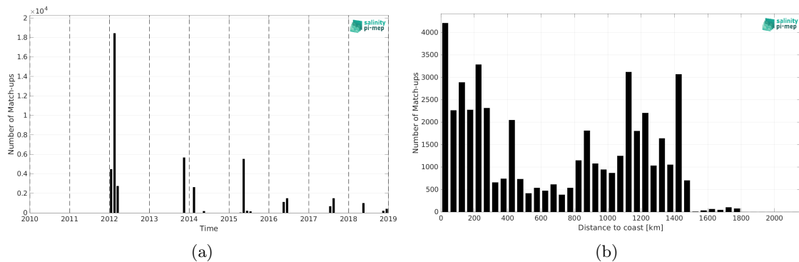
Figure 2: Number of match-ups between TSG (GOSUD-Sailing-ship) and SMOS SSS L4 v1 - Monthly (CMEMS-CNR) SSS as a function of time (a) and as function of the distance to coast (b) over the Gulf Stream Pi-MEP region and for the full satellite product period.
