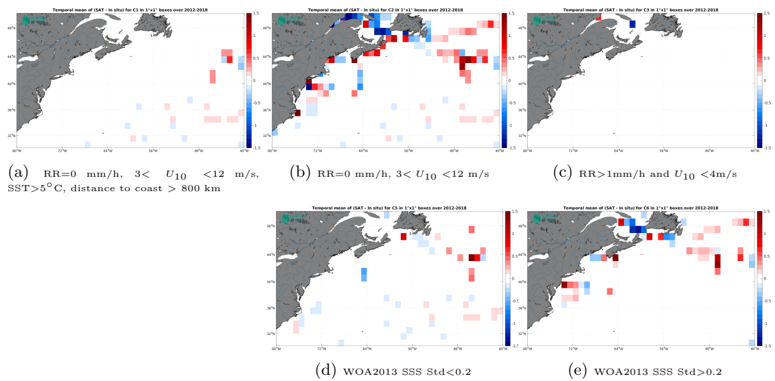
Figure 14: Temporal mean gridded over spatial boxes of size 1^\circ \times 1^\circ of \Delta SSS (SMOS SSS L4 v1 - Monthly (CMEMS-CNR) - TSG (GOSUD-Sailing-ship)) for 5 different subdatasets corresponding to:RR=0 mm/h, 3 < U_{10} < 12 m/s, SST>5°C, distance to coast > 800 km (a), RR=0 mm/h, 3 < U_{10} < 12 m/s (b), RR>1mm/h and U_{10} < 4 m/s (c), WOA2013 SSS Std<0.2 (d), WOA2013 SSS Std>0.2 (e).
