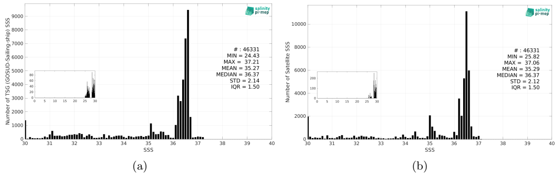
Figure 3: Histograms of SSS from TSG (GOSUD-Sailing-ship) (a) and SMOS SSS L4 v1 - Monthly (CMEMS-CNR) (b) considering all match-up pairs per bins of 0.1 over the Gulf Stream Pi-MEP region and for the full satellite product period.
