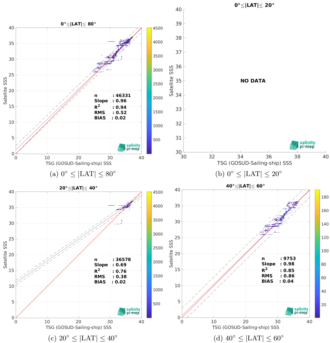
Figure 10: Contour maps of the concentration of SMOS SSS L4 v1 - Monthly (CMEMS-CNR) SSS (y-axis) versus TSG (GOSUD-Sailing-ship) SSS (x-axis) at match-up pairs for different latitude bands. For each plot, the red line shows x=y . The black thin and dashed lines indicate a linear fit through the data cloud and the \pm 95\% confidence levels, respectively. The number match-up pairs n , the slope and R^2 coefficient of the linear fit, the root mean square (RMS) and the mean bias between satellite and in situ data are indicated for each latitude band in each plots.
