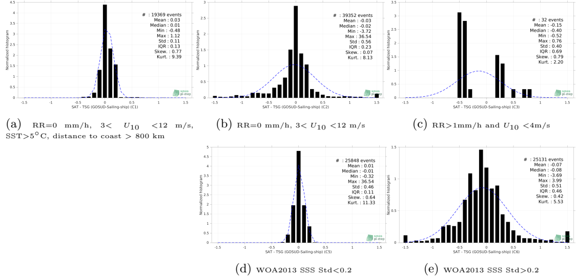
Figure 13: Normalized histogram of \Delta SSS (SMOS SSS L4 v1 - Monthly (CMEMS-CNR) - TSG (GOSUD-Sailing-ship)) for 5 different subdatasets corresponding to: RR=0 mm/h, 3 < U_{10} < 12 m/s, SST>5°C, distance to coast > 800 km (a), RR=0 mm/h, 3 < U_{10} < 12 m/s (b), RR>1mm/h and U_{10} < 4 m/s (c), WOA2013 SSS Std<0.2 (d), WOA2013 SSS Std>0.2 (e).
